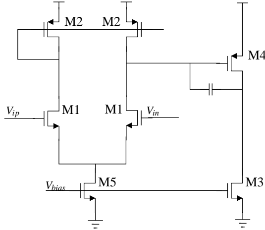
Figure 4.15: Basic operational amplifier: illustration.
