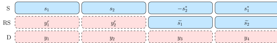
Figure 3.2: Transmission frames of the Alamouti DF protocol
