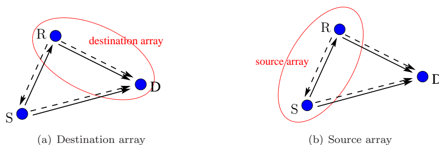
Figure 1.4: Cooperation as a virtual MIMO
