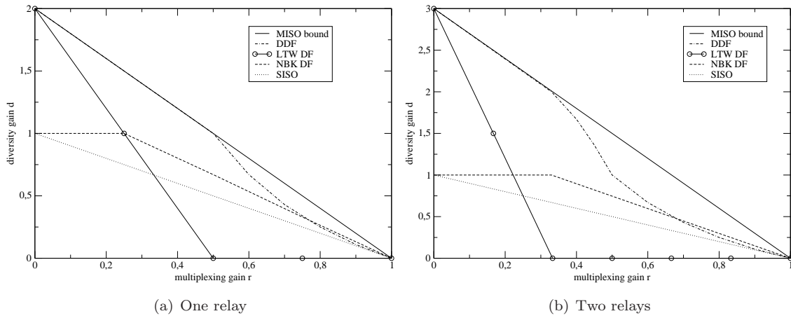
Figure 2.9: DMTs of existing DF protocols
