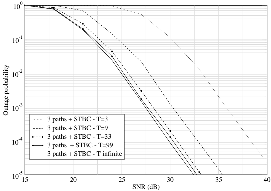
Figure 4.15: Outage probability of the path selection multihop protocol for different rate/frame length: T is the number of symbols to sent, thus the rate is \frac{T}{n+T-1} .
