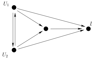
Figure 4.1: The multiple access relay channel (MARC) model for two sources
