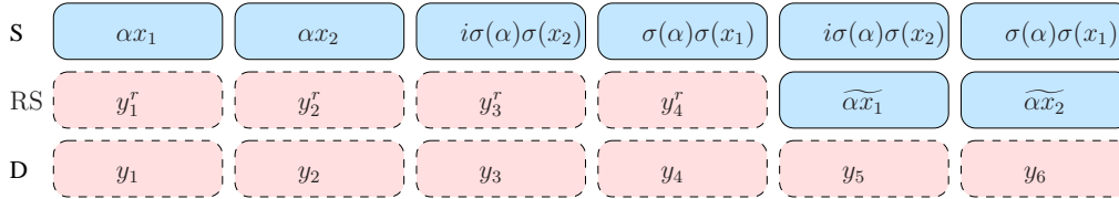
Figure 3.6: Transmission frame of the Asymmetric DF protocol implemented with a distributed Golden code in the one-relay case
