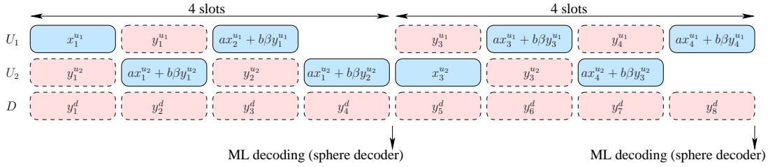
Figure 4.4: Transmission frame of the improved CMA-NAF protocol for a super frame of 8 time slots
