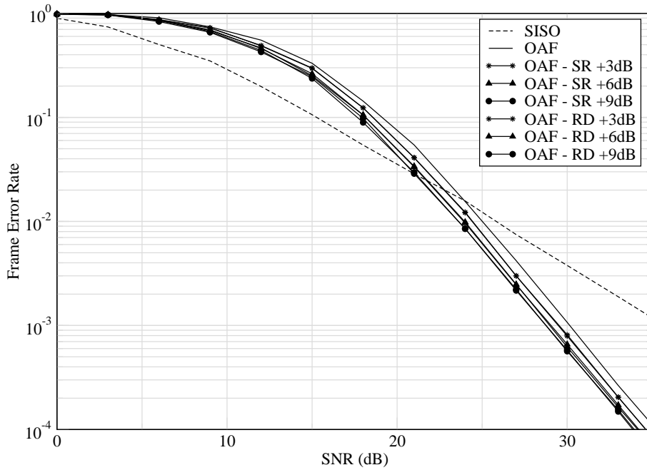
Figure 2.11: Influence of the relay location on the OAF performance
