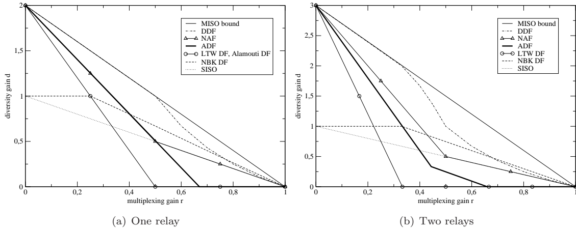
Figure 3.8: Asymmetric DF DMT
