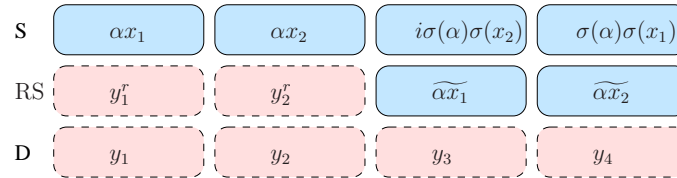
Figure 3.15: Transmission frame of the Incomplete DF protocol in the 1-relay case implemented with a distributed Golden code
