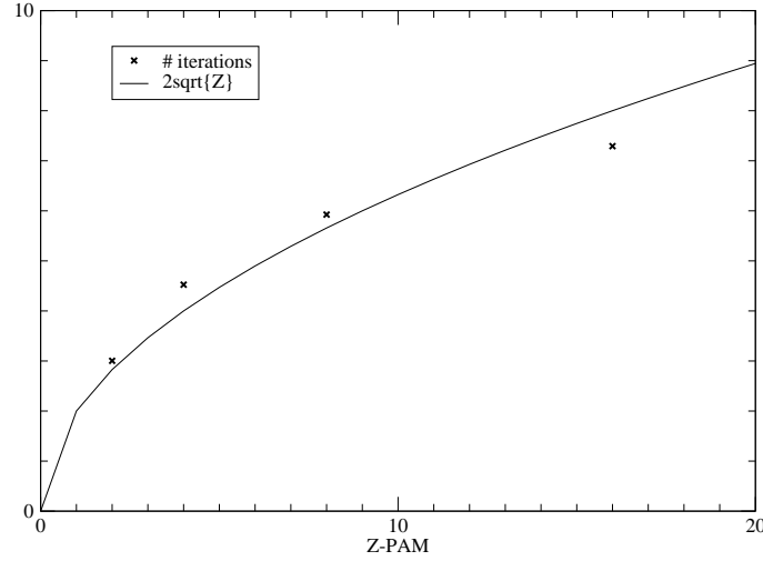
Figure 3.16: Complexity of the modified Cassels' algorithm: number of iterations of the modified Cassels' algorithm as a function of the size of the constellation
