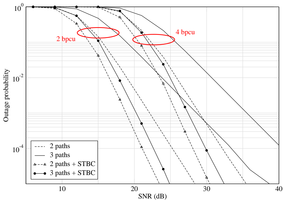
Figure 4.10: Outage probability of the path selection multihop protocol with and without a distributed STBC
