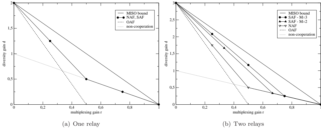
Figure 2.8: DMTs of existing AF protocols
