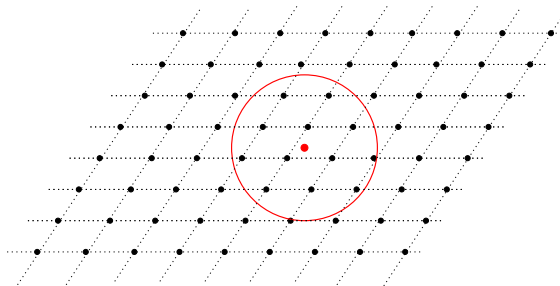
Figure 1.9: Search in an hypersphere centered on the received signal
