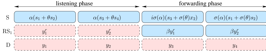
Figure 2.5: NAF frame implemented with the distributed Golden code
