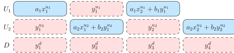
Figure 4.3: Transmission frame of the CMA-NAF protocol for 2 users and M = 2
