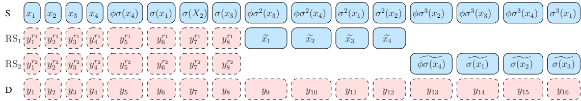
Figure 3.13: Transmission frame of the Incomplete DF protocol in the 2-relay case implemented with a distributed 4 \times 4 TAST code
