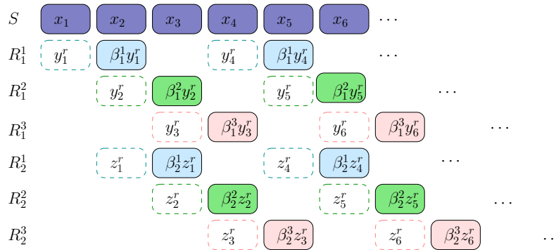
Figure 4.9: Transmission frame of the path selection multihop protocol
