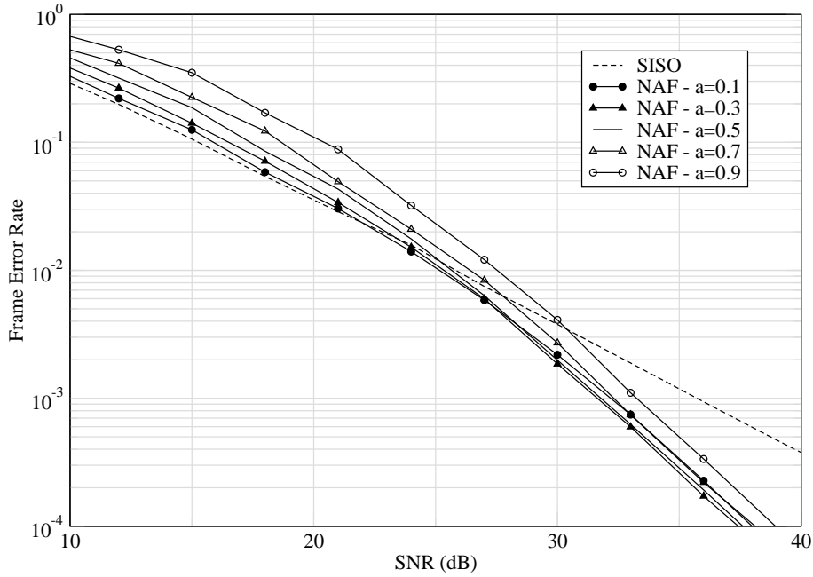
Figure 2.13: Influence of the power distribution on the NAF performance
