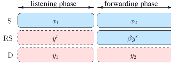
Figure 2.4: NAF frame for one relay
