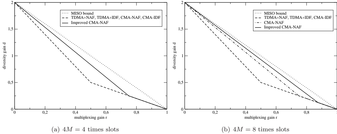
Figure 4.6: Modified CMA-NAF and CMA-IDF DMT
