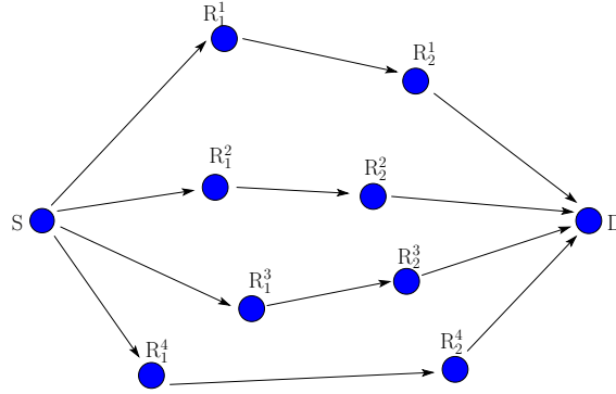
Figure 4.7: 4-PP channel with path length n = 3
