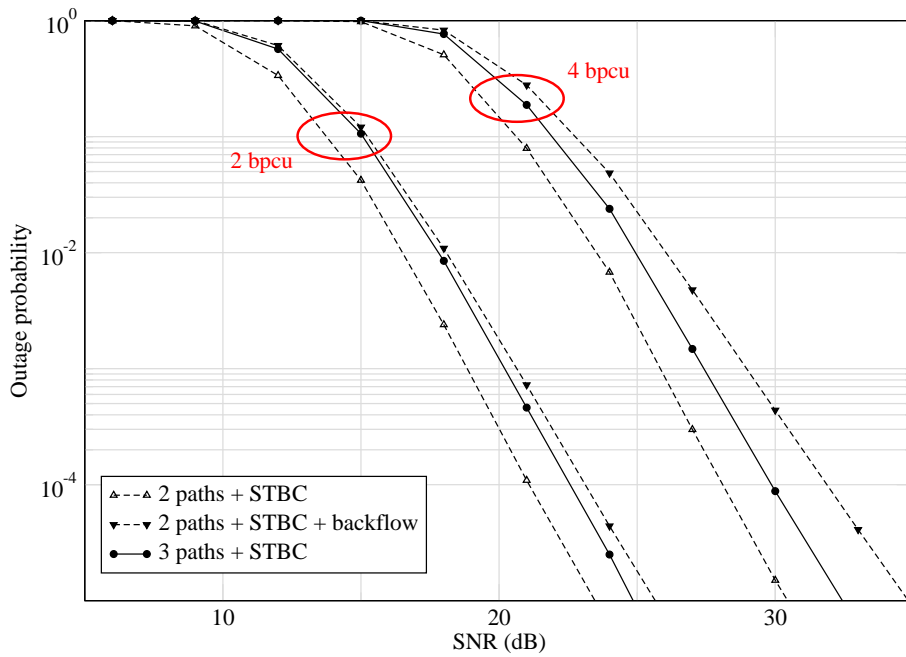
Figure 4.12: Influence of backflow on the outage probability of the path selection multihop protocol
