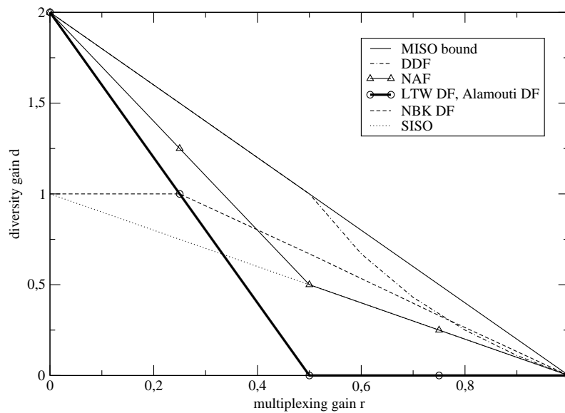
Figure 3.4: Alamouti DF DMT
