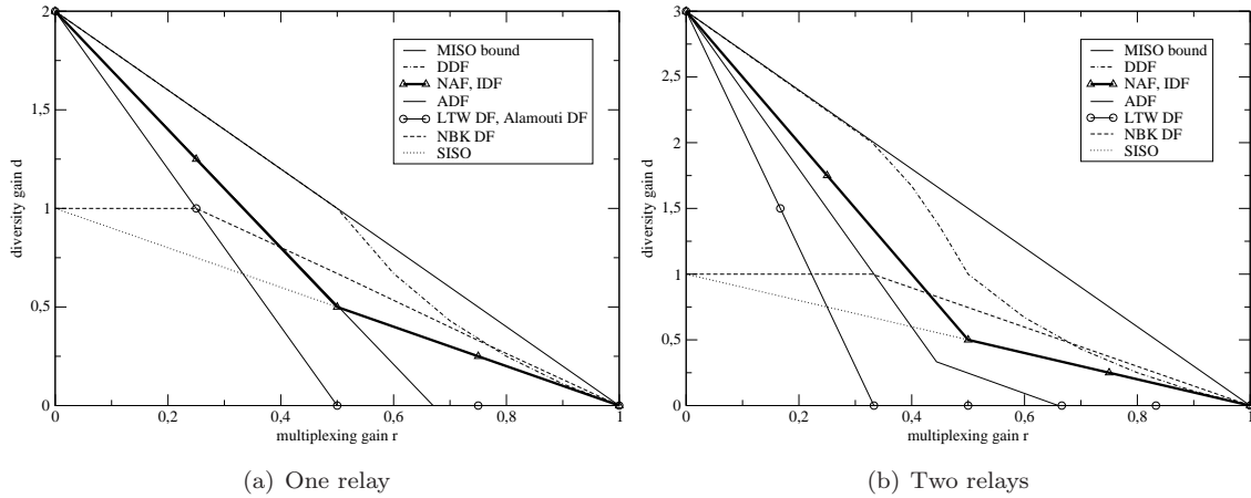
Figure 3.12: Incomplete DF DMT
