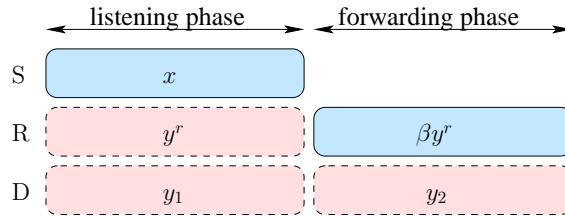
Figure 2.2: OAF protocol for 1 relay
