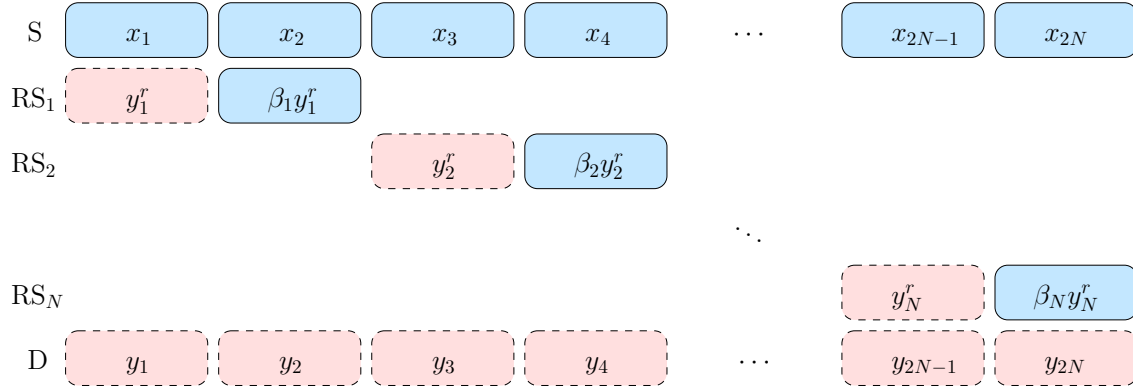
Figure 2.6: NAF frame for N relays
