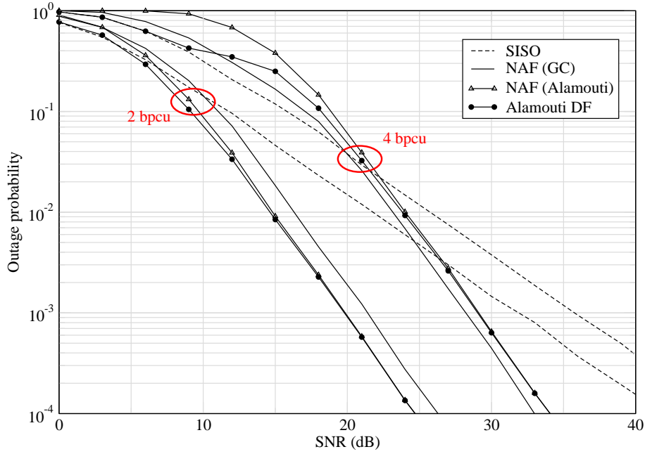
Figure 3.3: Alamouti DF outage probability
