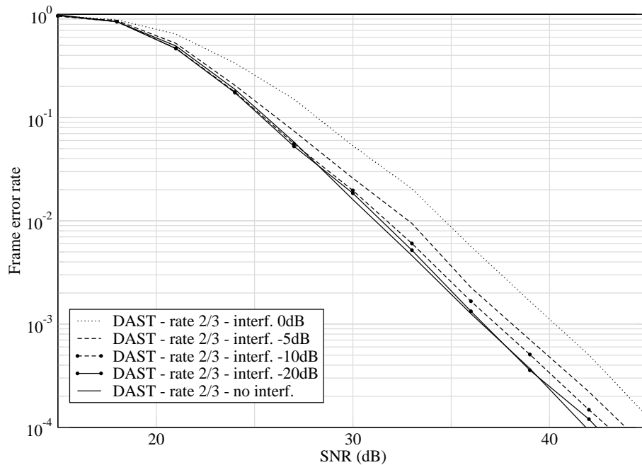
Figure 4.17: Influence of path interference on the performance of the path selection multihop protocol
