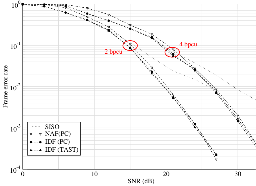
Figure 3.14: Incomplete DF frame error rate for two relays
