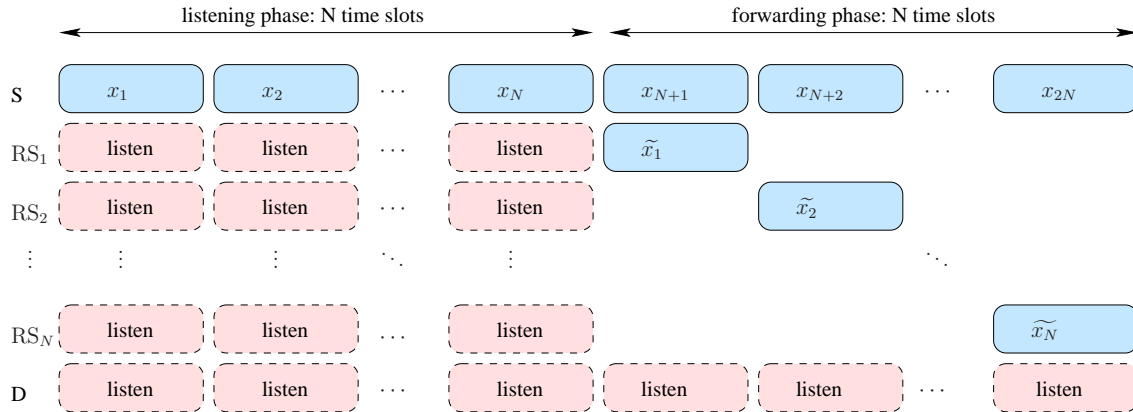
Figure 3.9: Transmission frame of the Incomplete DF protocol
