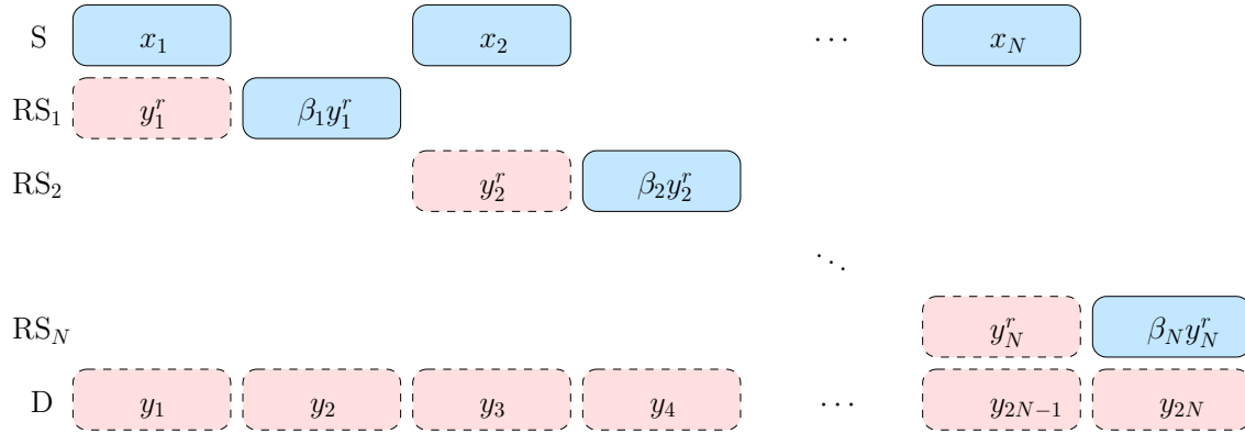
Figure 2.3: OAF protocol for N relay
