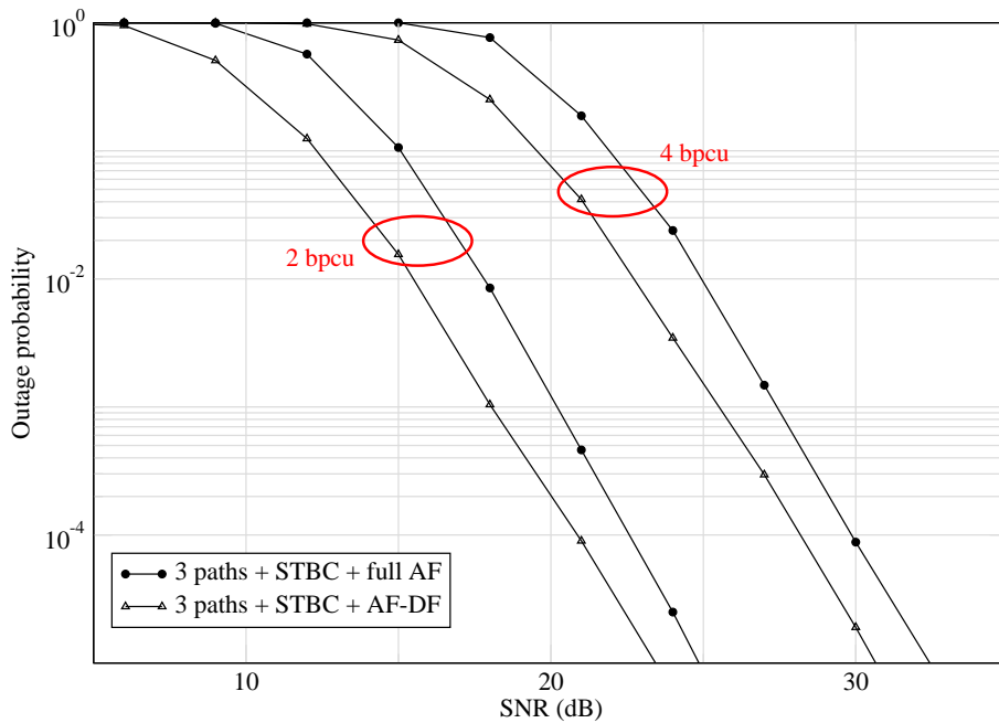
Figure 4.13: Outage probability of the path selection multihop protocol using a combination of DF and AF strategies
