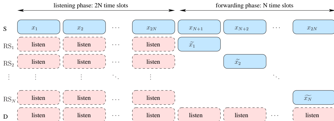
Figure 3.5: Transmission frame of the Asymmetric DF protocol
