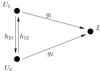
Figure 4.2: The cooperative multiple-access (CMA) channel model for two sources
