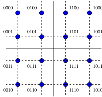
Figure 1.6: Example of the 16-QAM constellation
