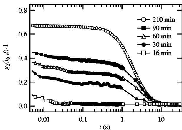
FIG. 8. Correlation functions g_2(t_0, t) - 1 ( = \beta |g_1(t_0, t)|^2 ) started at different times t_0 (indicated in the plot) after the quench of a 1% gelatine gel with 1% latex spheres from 60 to 20 °C. The typical evolution time is around 10 min. The rise of the intercept and plateau corresponds to the disappearance of the fast liquid phase relaxation process and concurrent increase of the gel elastic modulus.
