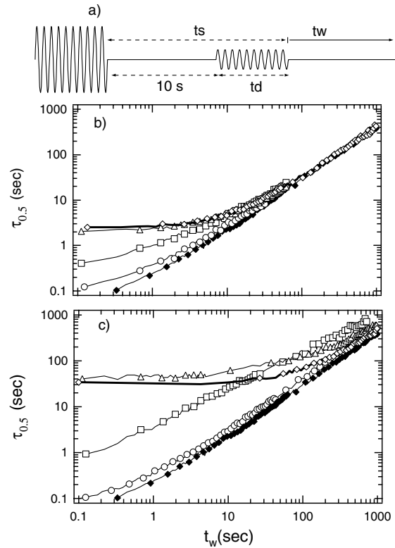
FIG. 2. (a) Strain history. (b) \tau_{1/2} for t_s = 11 s and different strain amplitudes \gamma = 0\% ( \diamond ), 2.9% ( \triangle ), 7.9% ( \square ), 11.7% ( \circ ), and the reference curve ( \blacklozenge ). \tau_{1/2} decreases monotonically with the strain amplitude at short times. For t_w \sim t_s all curves merge. (c) \tau_{1/2} for t_s = 110 s for the same strain amplitude. \tau_{1/2} for \gamma = 2.9\% and 7.9% is superior to \gamma = 0\% in the long time regime.
