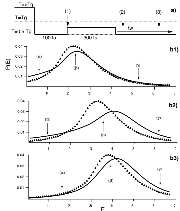
FIG. 3. (a) Temperature history. (b) P(E, t_w) vs E for various t_w . The ( \blacktriangle ) curve corresponds to the reference case; the full line corresponds to the case with a step ( \Delta T = \frac{1}{3}T_g ). Notice that 1 tu after the sample is reheated (1) the small energies are overpopulated, the intermediate ones are depleted, and the large ones remain unchanged. At 1 tu after the second quench (2) both small and large energies are overpopulated. At 3000 tu after the second quench, small energies and intermediate energies are depleted, whereas large energies stay overpopulated.
