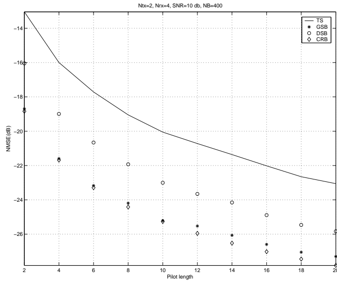
Figure 7.1: Normalized MSE vs N_{TS} : flat channel, N_{tx} = 2, N_{rx} = 4, N_B = 400, \text{SNR} = 10 \text{ dB} .
