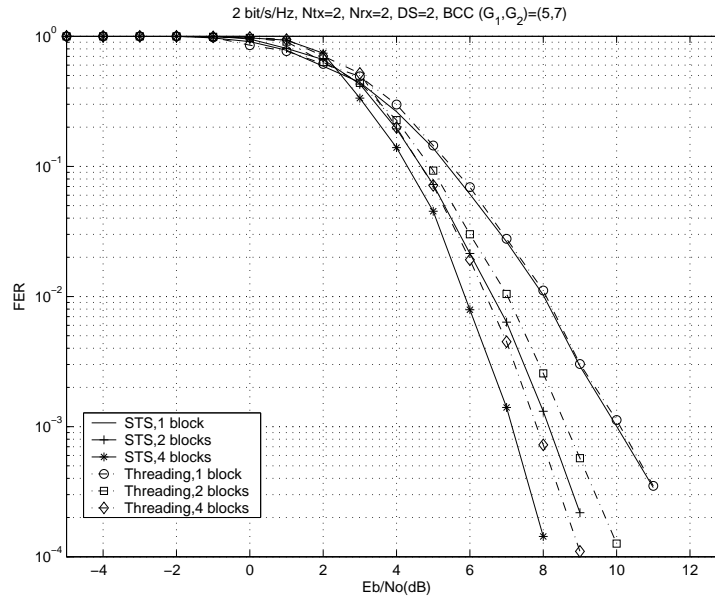
Figure 7.20: STS/Threading pour (N_{tx}, N_{rx}) = (2, 2) , L = 2 , F = 1, 2, 4 .
