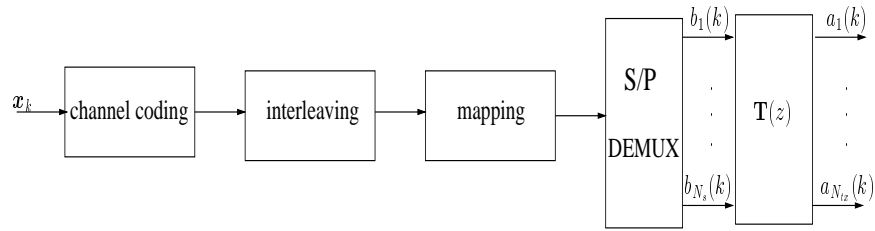
Figure 4.1: Encoder for space-time spreading.
