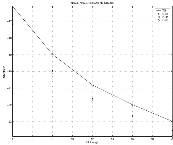
Figure 7.5: Normalized MSE vs N_{TS} : flat channel, N_{tx} = 4 , N_{rx} = 2 , N_B = 400 , SNR= 10 dB.
