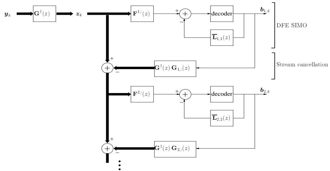
Figure 3.1: Stripping MIMO DFE receiver.
