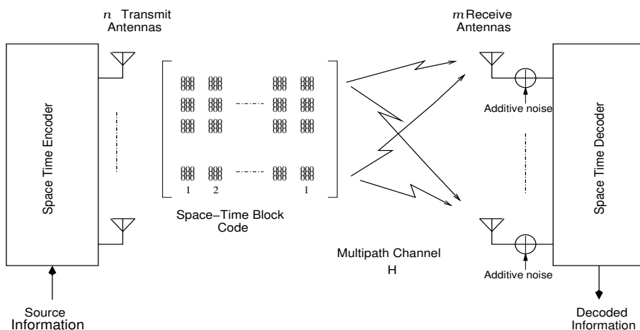
Figure 2.1: Space-Time coding scheme
