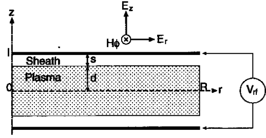
Figure 3. Uniform slab model of axisymmetric discharge.
