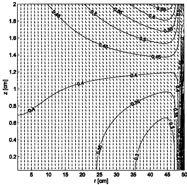
Figure 12. Direction ( \rightarrow ) of plasma electric field E_p and 5% contours of E_p^2 = E_r^2 + E_z^2 as a function of r and z for f = 40.7 MHz and n_e = 7 \times 10^9 cm ^{-3} .
