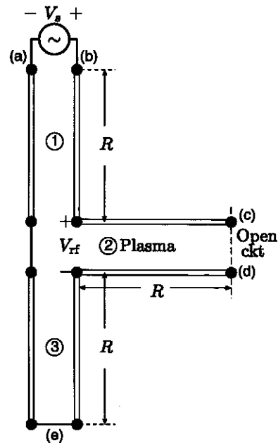
Figure 2. Transmission line model; the points (a)–(c) correspond to those shown at r = 0 in figure 1.
