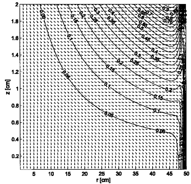
Figure 14. Direction ( \rightarrow ) of plasma electric field E_p and 5% contours of E_p^2 = E_r^2 + E_z^2 as a function of r and z for f = 40.7 MHz and n_e = 5 \times 10^{10} cm ^{-3} .
