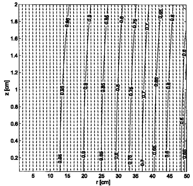
Figure 10. Direction ( \rightarrow ) of plasma electric field E_p and 5% contours of E_p^2 = E_r^2 + E_z^2 as a function of r and z for f = 40.7 MHz and n_e = 10^9 cm ^{-3} .
