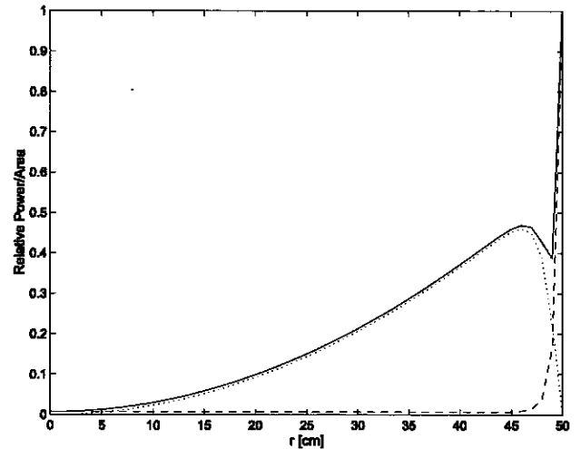
Figure 9. P_{\text{cap}} (---), P_{\text{ind}} (.....), and P_{\text{tot}} (—) as a function of r for f = 13.56 MHz and n_e = 10^{11} cm ^{-3} .
