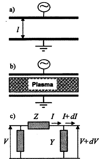
FIG. 1. Parallel plate system without plasma (a) and with plasma (b), along with the equivalent transmission line model (c).
