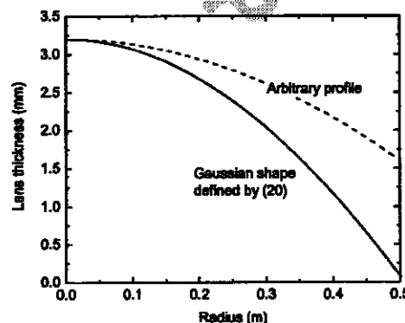
FIG. 7. Dielectric lens thickness as a function of radius; the ideal Gaussian shape defined by (20) (solid line), and an arbitrarily modified profile (dashed line).
