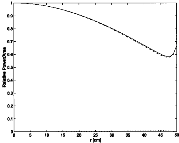
Figure 11. P_{\text{cap}} (---), P_{\text{ind}} (.....), and P_{\text{tot}} (—) as a function of r for f = 40.7 MHz and n_e = 10^9 cm ^{-3} .
