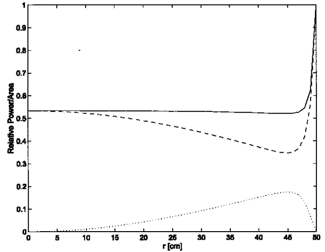
Figure 13. P_{\text{cap}} (---), P_{\text{ind}} (.....), and P_{\text{tot}} (—) as a function of r for f = 40.7 MHz and n_e = 7 \times 10^9 cm ^{-3} .
