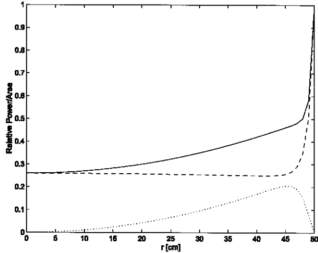
Figure 7. P_{\text{cap}} (---), P_{\text{ind}} (.....), and P_{\text{tot}} (—) as a function of r for f = 13.56 MHz and n_e = 10^{10} cm ^{-3} .
