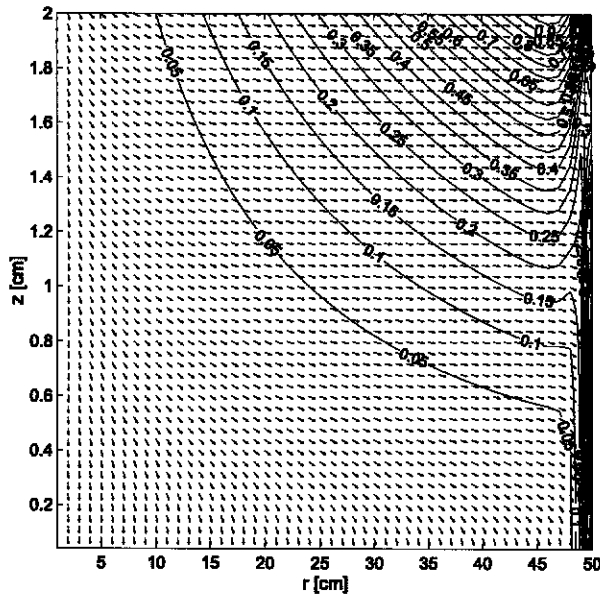
Figure 8. Direction ( \rightarrow ) of plasma electric field E_p and 5% contours of E_p^2 = E_r^2 + E_z^2 as a function of r and z for f = 13.56 MHz and n_e = 10^{11} cm ^{-3} .
