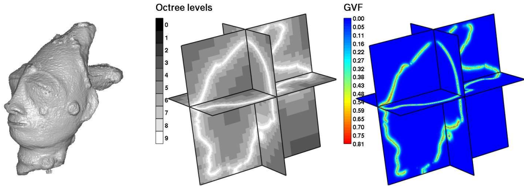
Figure 3.44: Stereo force computation for the Anyi sequence. From left to right, view of the correlation voting volume after binarization of the accumulated correlation (threshold=15), octree partition and GVF norm.
