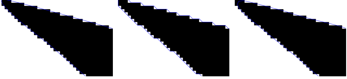
Figure 1.18: Silhouette contour discretization. Left: original exact contour (blue) superposed to the binary silhouette. Middle: extracted contour passing through the border of the contour pixels. Right: extracted contour after a curvature-driven regularization.
