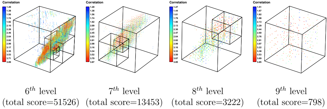
Figure 2.18: Voxel size as a function of the octree depth. The accumulated correlation score inside the voxel decreases by a factor of 4 with each new level, as expected. Individual correlation scores range from 1.2 to 4 since: i) the 4 closest cameras were used to correlate ( \pm 10^\circ and \pm 20^\circ ), with a minimum curve correlation score t_{bin} = 0.6 , and ii) a minimum of 2 coherent curves are needed n_{bin} = 2 .
