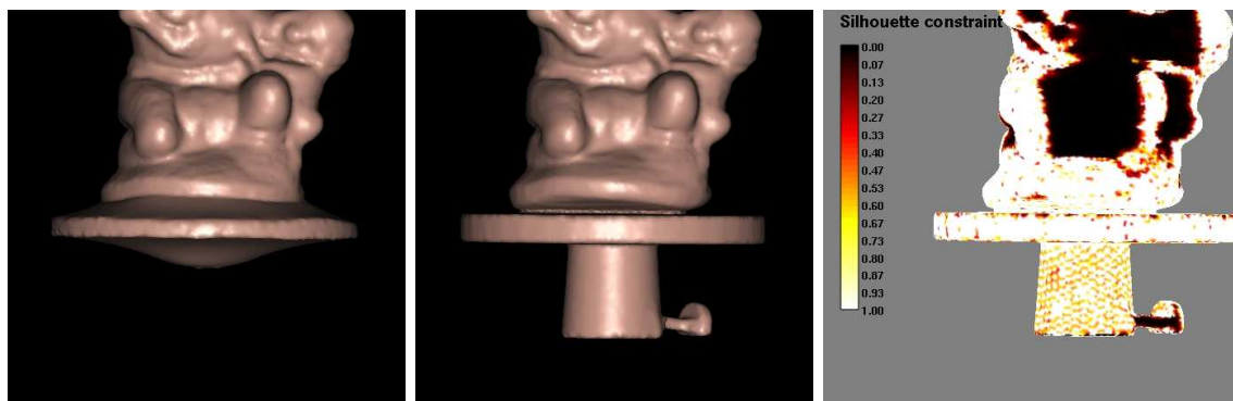
Figure 3.11: Twins model detail after convergence. Left: evolution under texture force only. Parts of the object with no texture disappear. Middle: evolution under both the texture force and the silhouette force. The parts of the object with no texture follow the silhouette force (visual hull). Right: \alpha component of the silhouette force after convergence.
