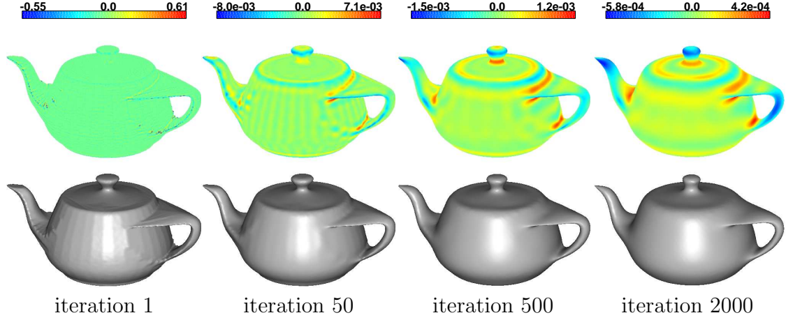
Figure 2.27: Bi-harmonic filtering ( \gamma = 1 , \rho = 1 ) for an increasing number of iterations. Top: dot product between the bi-harmonic force vector ( -\tilde{\Delta}^2 \mathbf{v} ) and the surface normal. Bottom: shaded view of the filtered model.
