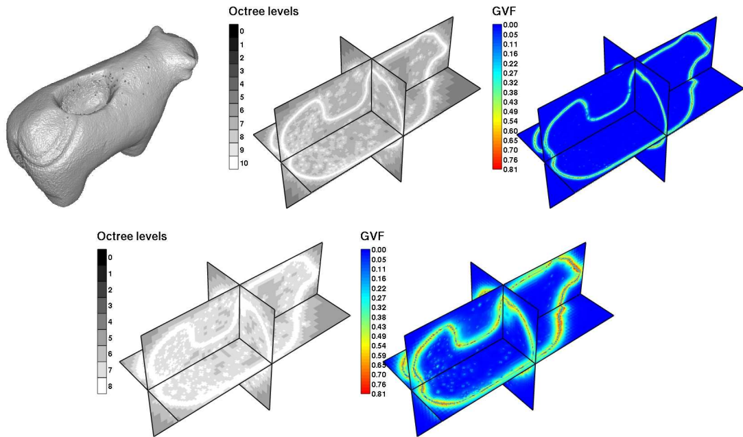
Figure 3.52: GVF computation for the first Toro sequence. From left to right: rendered view of the correlation volume after binarization of the accumulated correlation (threshold=30), octree partition and GVF norm.
