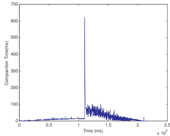
Figure 37: Performance of SR Algorithm
