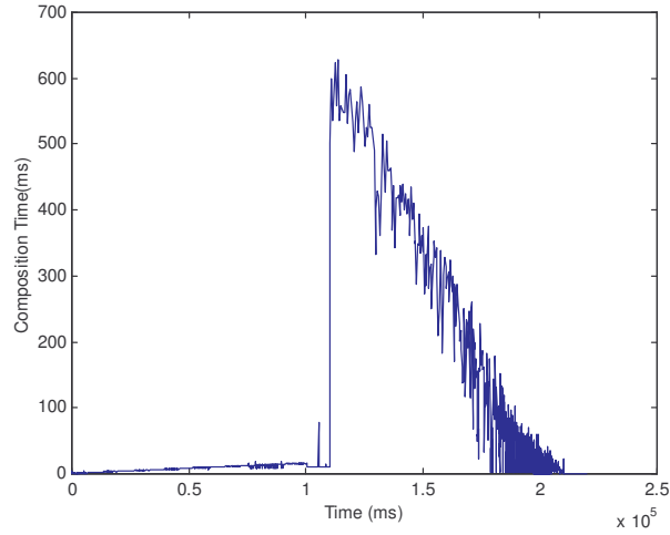
Figure 36: Performance of RS Algorithm
