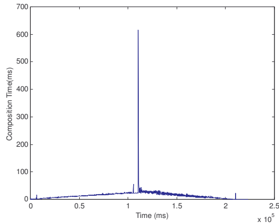
Figure 38: Performance of the DR algorithm
