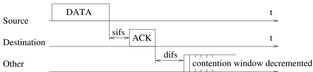
Figure 1.14: Basic mode access of IEEE 802.11 DCF.
