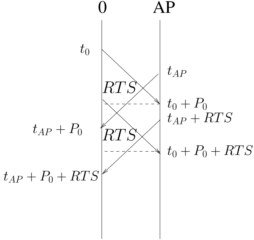
Figure B.4: Collision of the second order.
