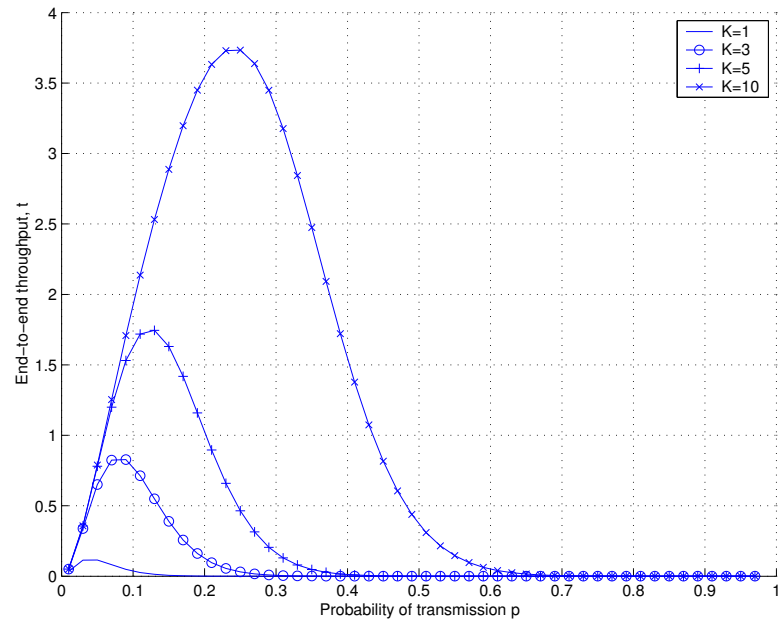
Figure 4.31: End-to-end throughput in packets/time-slot for the simple model of multi-packet reception for different values of K , and N = 100 nodes.
