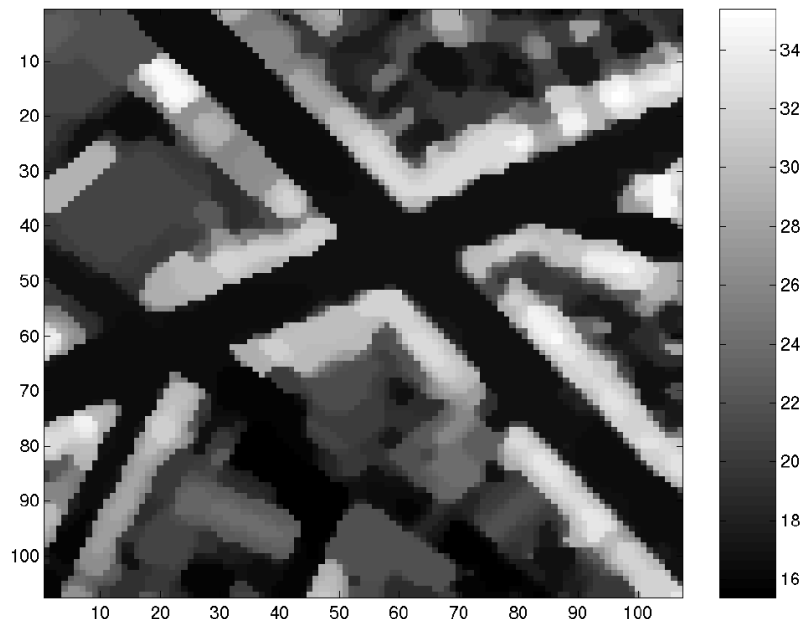
Figure 4.28: Both potential functions are total variation.
