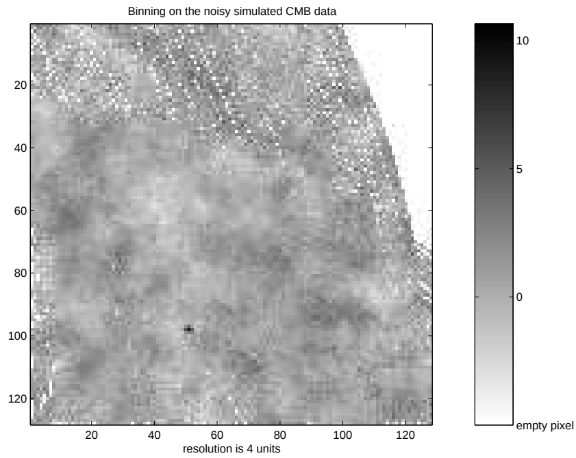
Figure 6.30: Binning on the noisy data, the resolution is 4 units.
