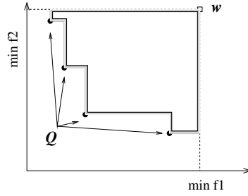
FIG. 4.10 – Hypervolume
