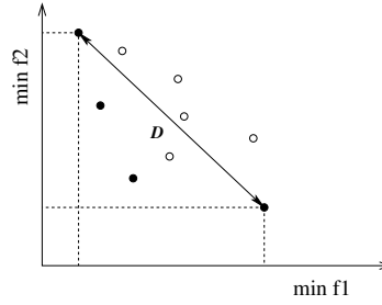
FIG. 4.9 – Maximum Spread
