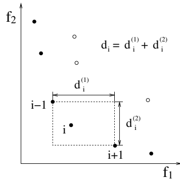
FIG. 3.7 – Crowding distance
