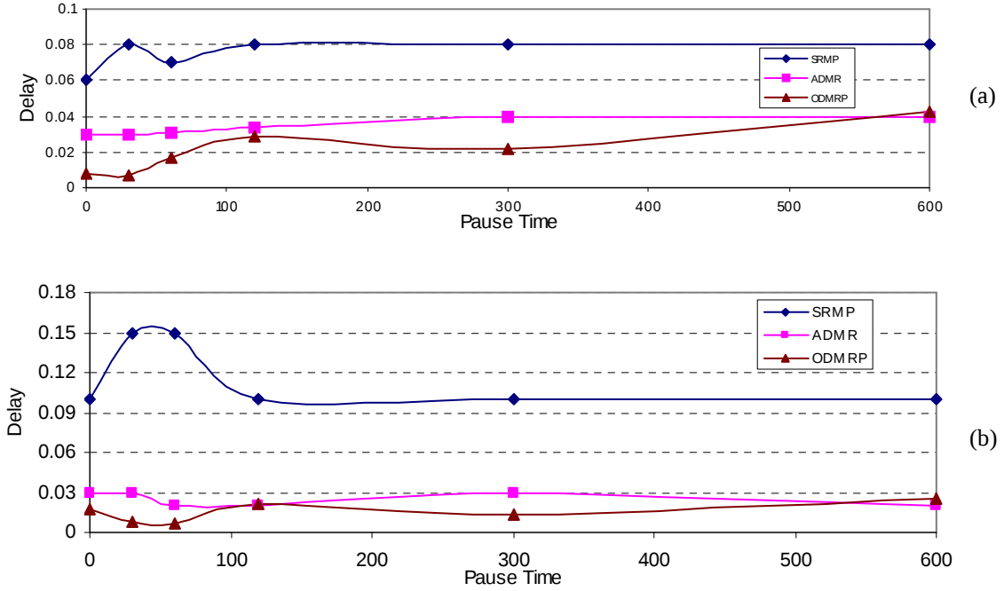
Figure 5.20 Average End-to-End Delay : (a) 1 Multicast Group Case and (b) 3 Multicast Groups Case
