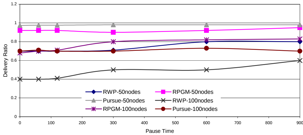
Figure 4.12 EC-DSR Average Delivery Ratio
