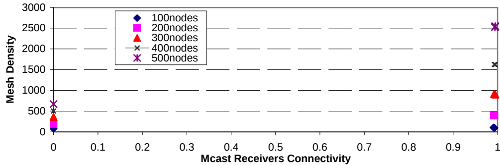
Figure 7.10 Large Scale Graph: Multicast Receivers Connectivity versus Mesh Density
