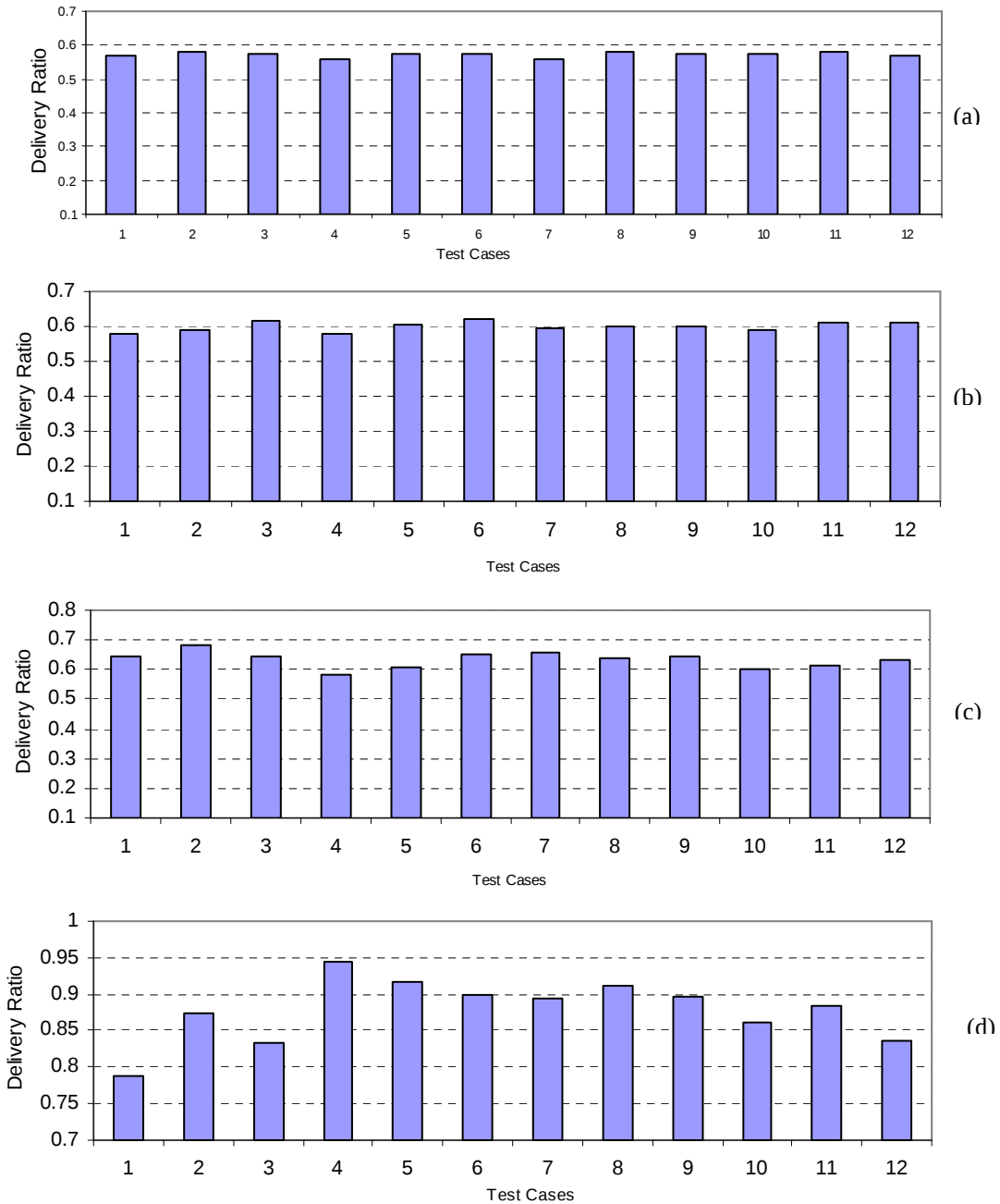
Figure 6.3 Delivery Ratio for Different Test Cases: Highly Mobile and Stable Network States, (a) Pause Time 0, (b) Pause Time 30, (c) Pause Time 300 and (d) Pause Time 600
