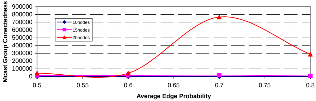
Figure 7.3 Small Size Graph: Average Edge Probability versus Multicast Group Connectedness
