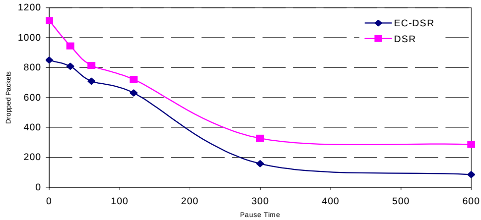
Figure.4.5 Average packets drops
