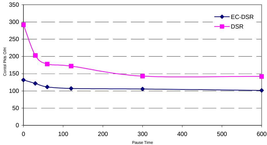
Figure 4.6 Packets Control Overhead
