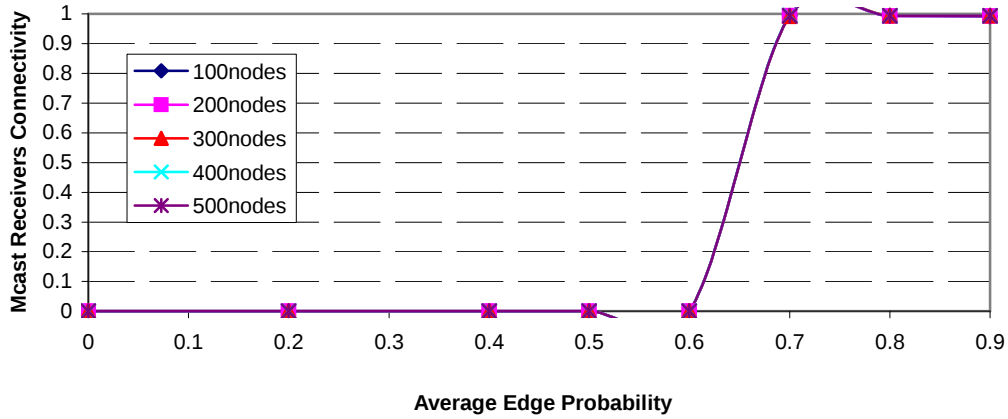
Figure 7.8 Large Scale Graph: Average Edge Probability versus Multicast Receivers Connectivity
