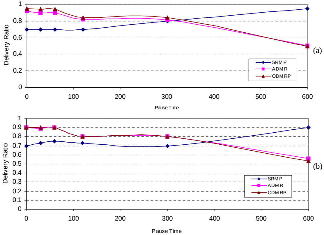
Figure 5.19 Average Delivery Ratio: (a) 1 Multicast Group Case and (b) Average Delivery Ratio: 3 Multicast Groups Case
