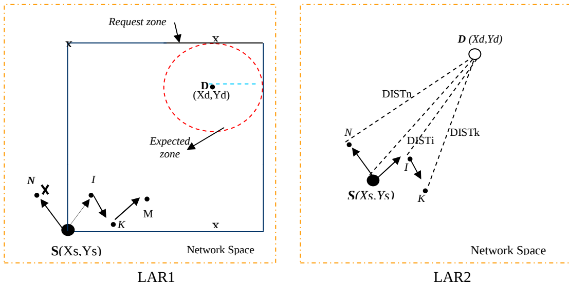
Figure 2.6 Expected and Request Zone
