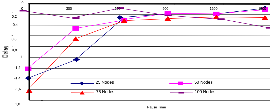
Figure 4.8 EC-DSR Vs DSR Absolute Delay
