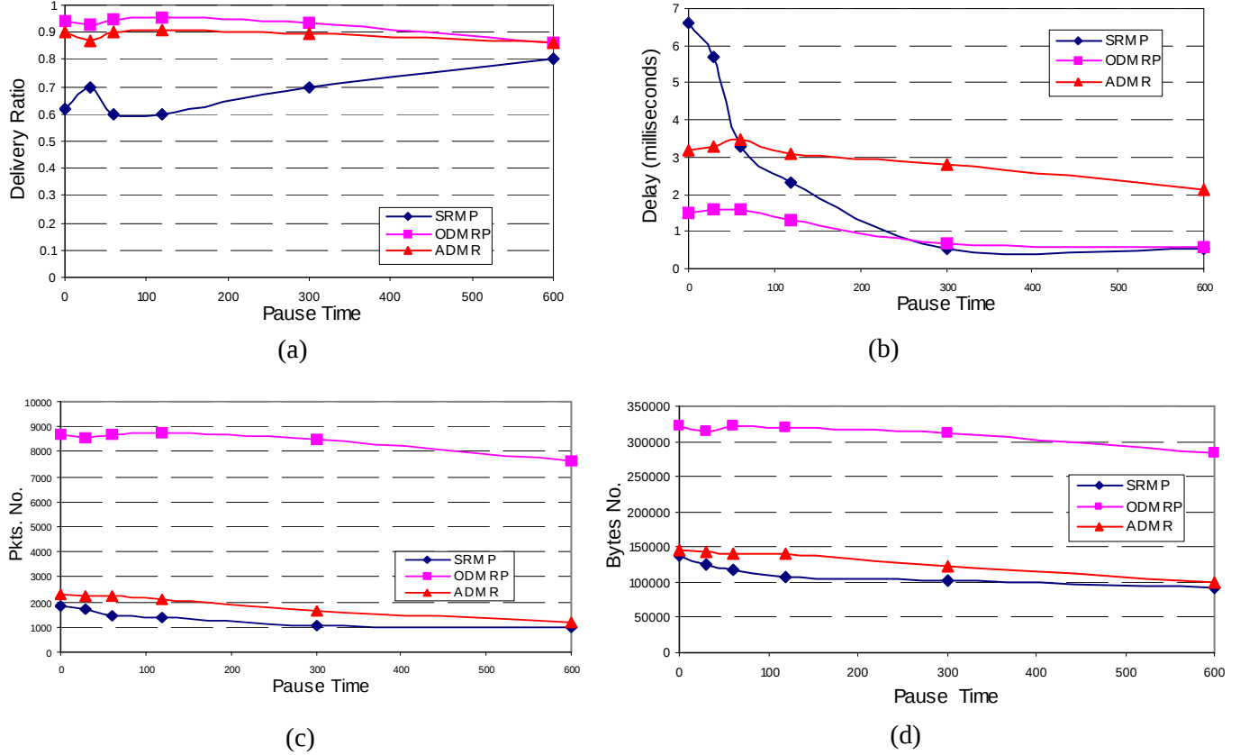
Figure 5.14 3 Sources and 3 Multicast Receivers Per Source: (a) Average Delivery Ratio, (b): Average End-to-End Delay, (c): Average Control Packets Overhead and (d): Average Control Bytes Overhead
