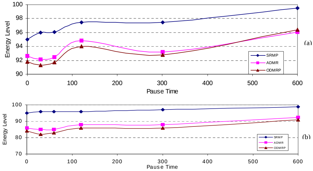
Figure 5.22 Average Energy Level: (a) 1 Multicast Group Case and (b) 3 Multicast Groups Case
