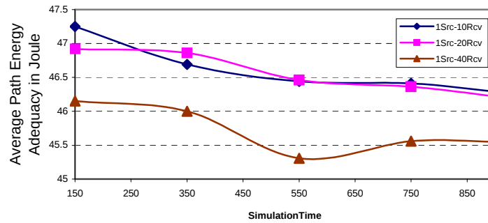
Figure 5.26 1 Multicast Group Cases: Average Path Energy
