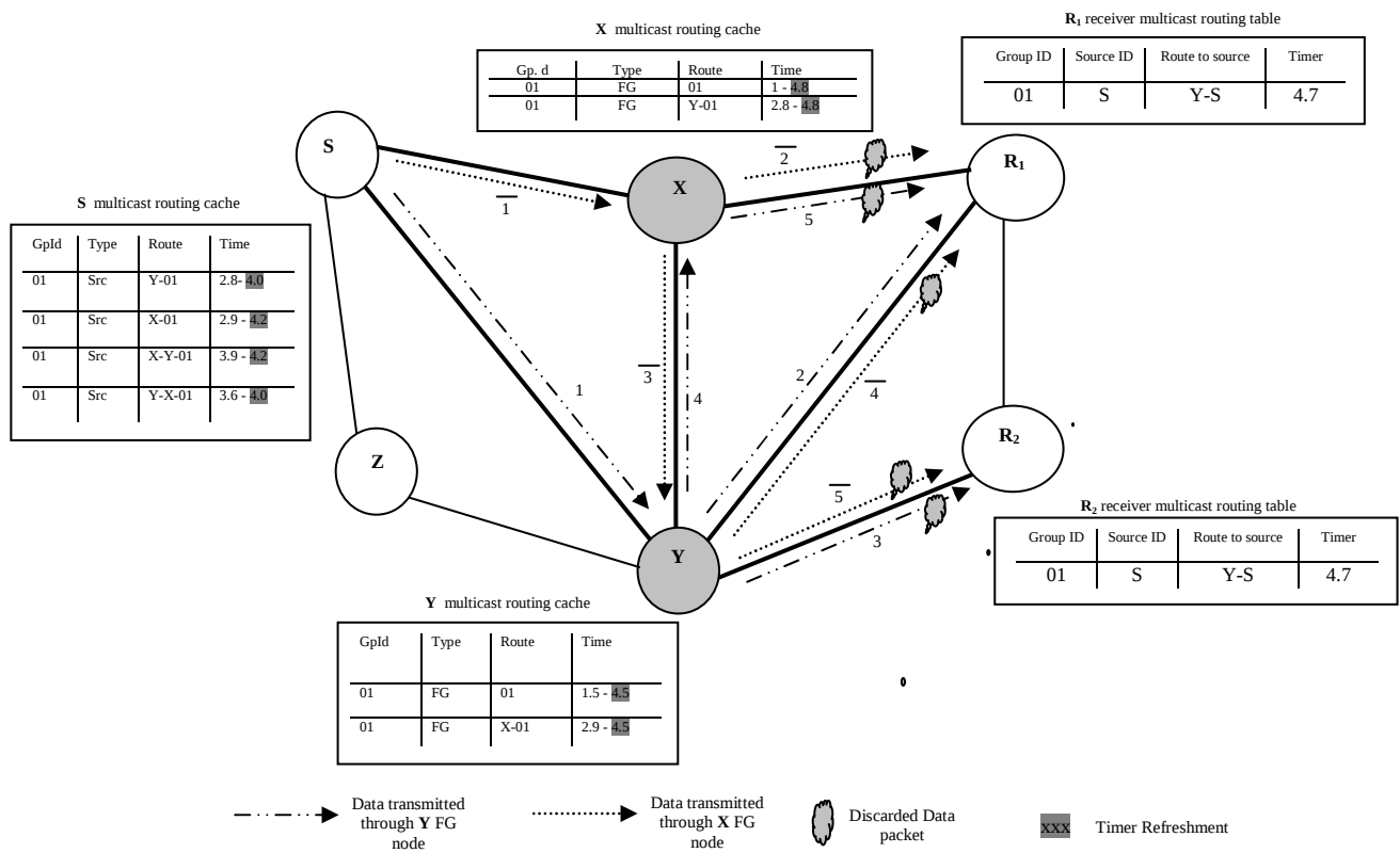
Figure 5.8 Data Transmission and Forward
