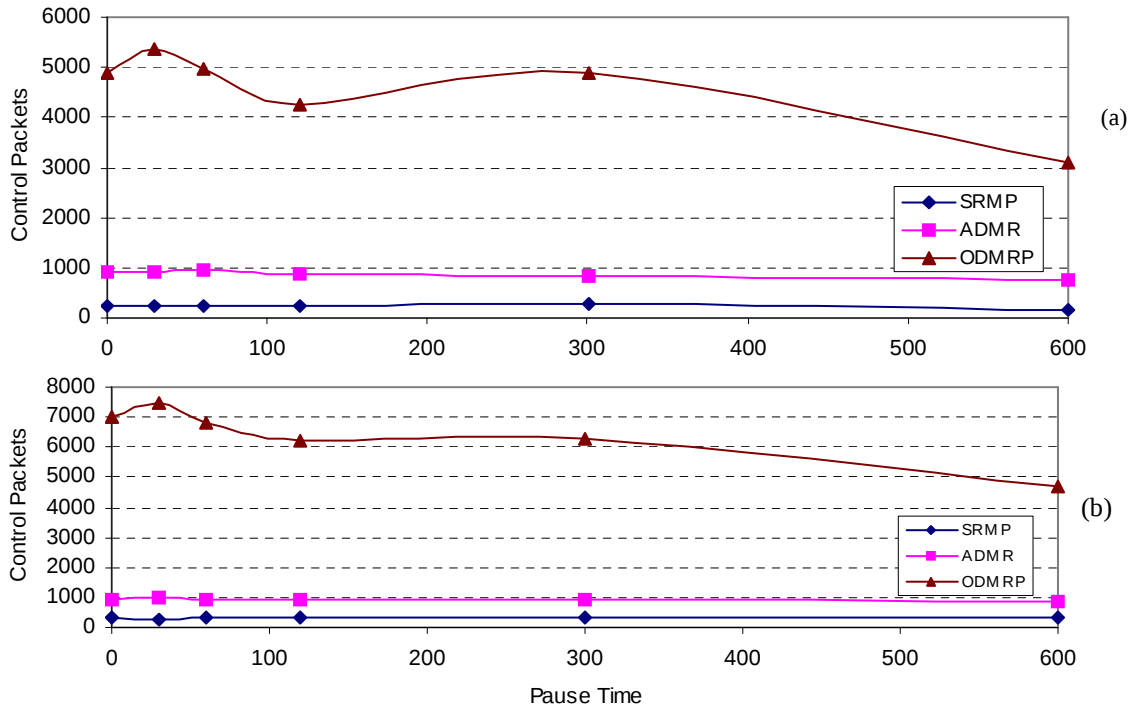
Figure 5.21 Average Control Packets: (a) 1 Multicast Group Case and (b) 3 Multicast Groups Case
