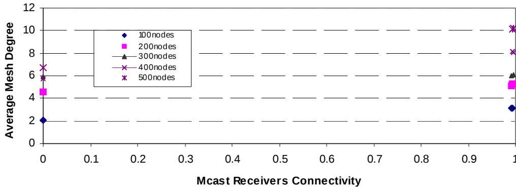
Figure 7.11 Large Scale Graph: Multicast Receivers Connectivity versus Average Mesh Degree
