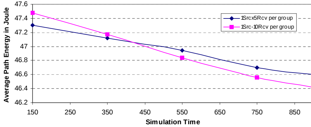
Figure 5.28 2 Multicast Groups Cases: Average Path Energy
