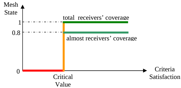
Figure 7.12 Mesh State based on Criteria Satisfaction
