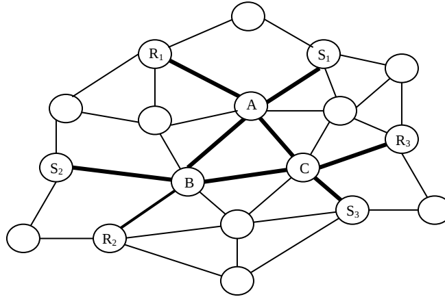
Figure 3.7 Join-Reply Forwarding
