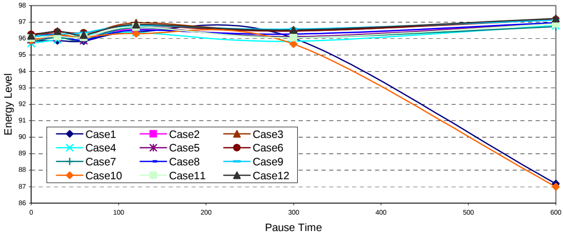
Figure 6.12 Energy Level
