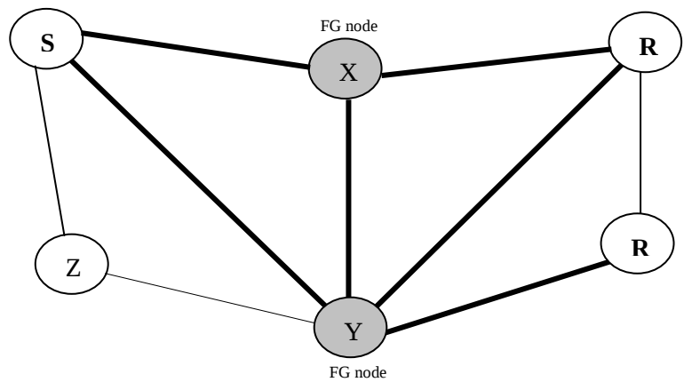
Figure 5.7 Mesh Creation
