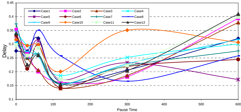
Figure 6.4 End-to-End Delay
