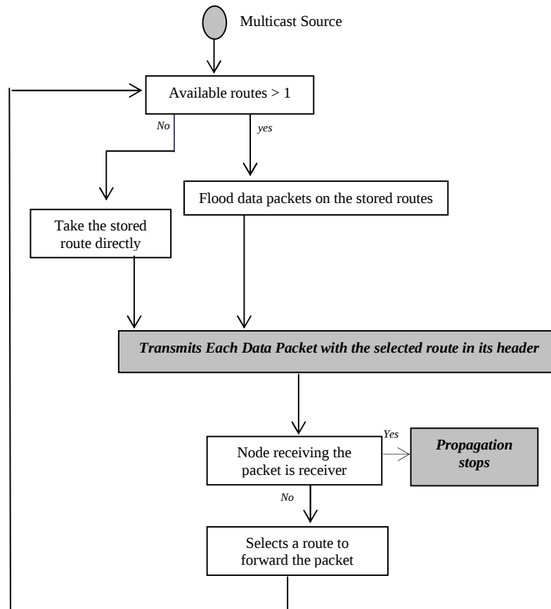
Figure 5.5 Data Forwarding
