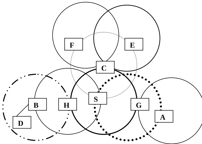
Figure 2.5 An Example of ZRP Operation
