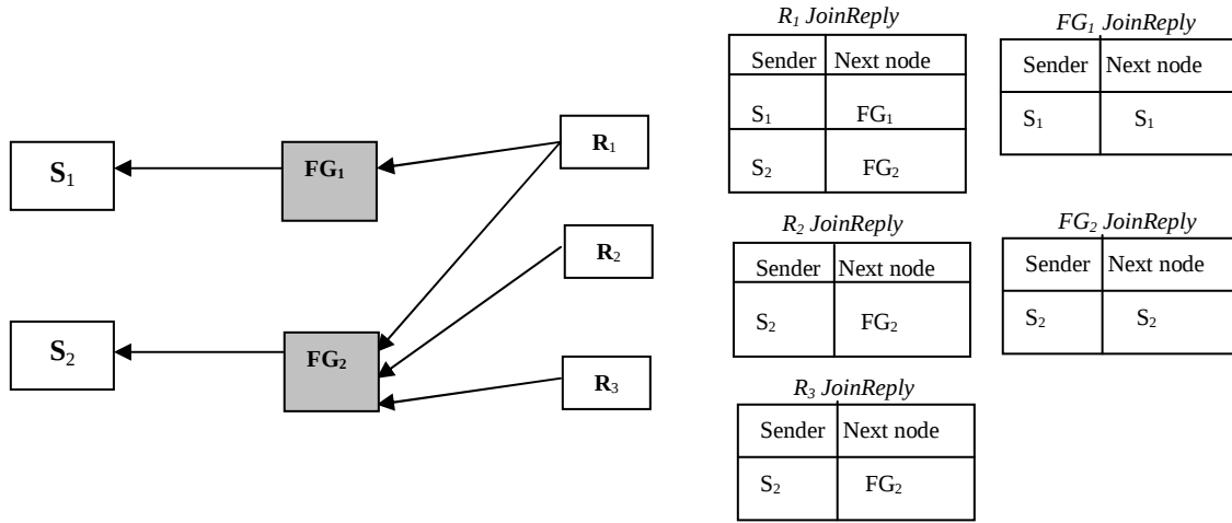
Figure 3.7 Join-Reply Forwarding
