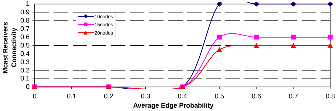
Figure 7.1 Small Size Graph: Average Edge Probability versus Multicast Receivers Connectivity
