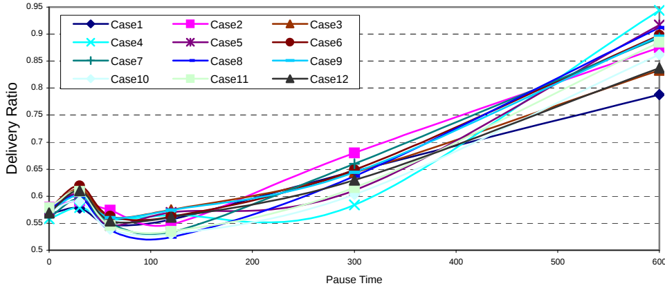
. Figure 6.2 Delivery Ratio
