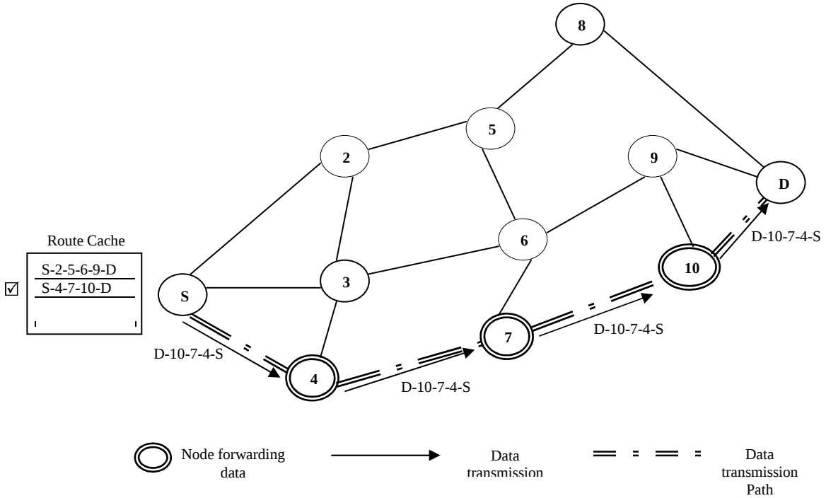
Figure 4.2 Data Transmission from S to D
