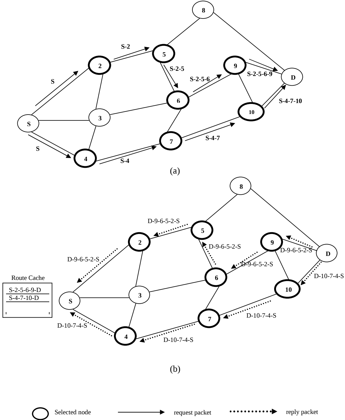
Figure 4.1 An Example of the Request/Reply Processes in a Small Network: (a) Route Discovery Process, (b) Route Reply Process
