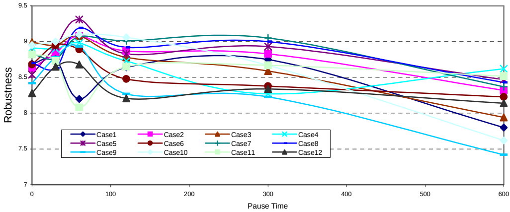
Figure 6.10 SRMP Robustness
