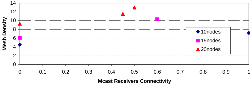
Figure 7.4 Small Size Graph: Multicast Receivers Connectivity versus Mesh Density
