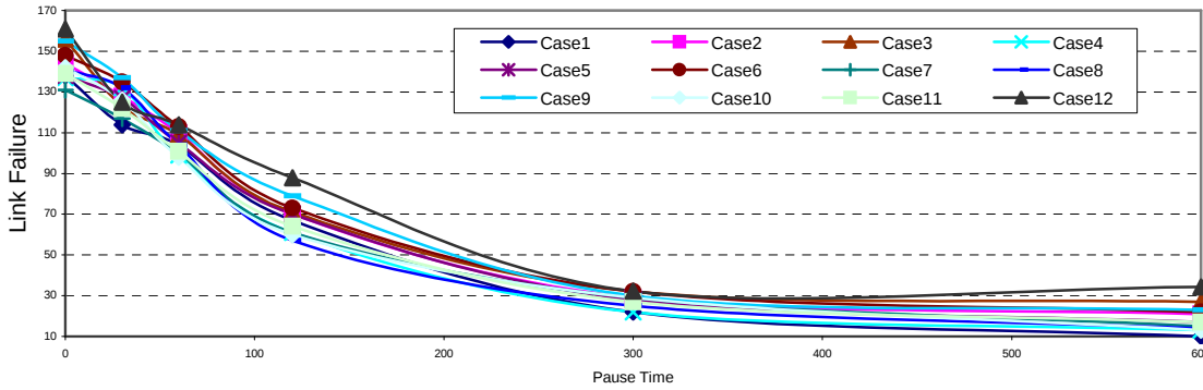
Figure 6.8 Link Failure
