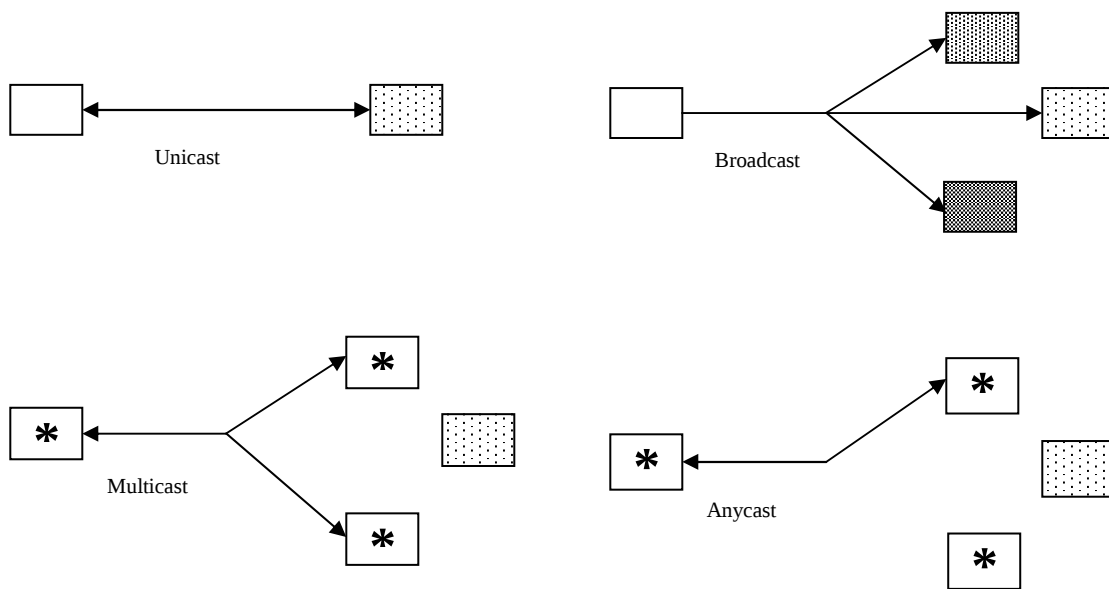
Figure 3.1 Unicast, Broadcast, Multicast, and Anycast
