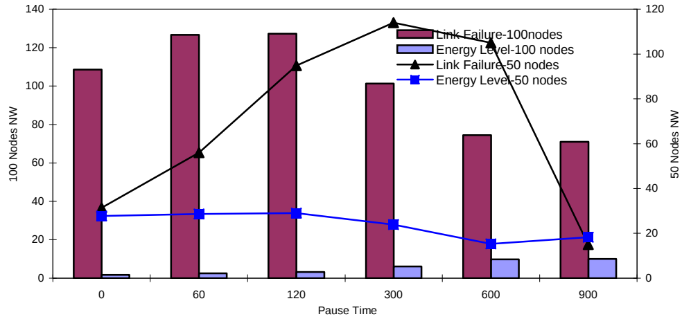
Figure 4.17 RWP Energy Level Vs Link Failure
