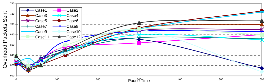
Figure 6.6 SRMP Control Overhead
