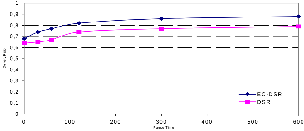
Figure 4.4 Average delivery ratio
