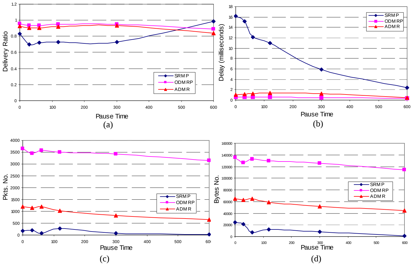
Figure 5.13 1 Source and 10 Multicast Receivers: (a) Average Delivery Ratio, (b) Average End-to-End Delay, (c) Average Control Packets Overhead and (d) Average Control Bytes Overhead
