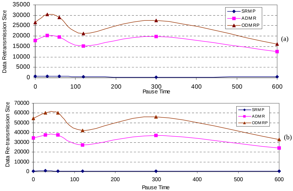
Figure 5.23 Average Data Re-transmission Size: (a) 1 Multicast Group Case and (b) 3 Multicast Groups Case
