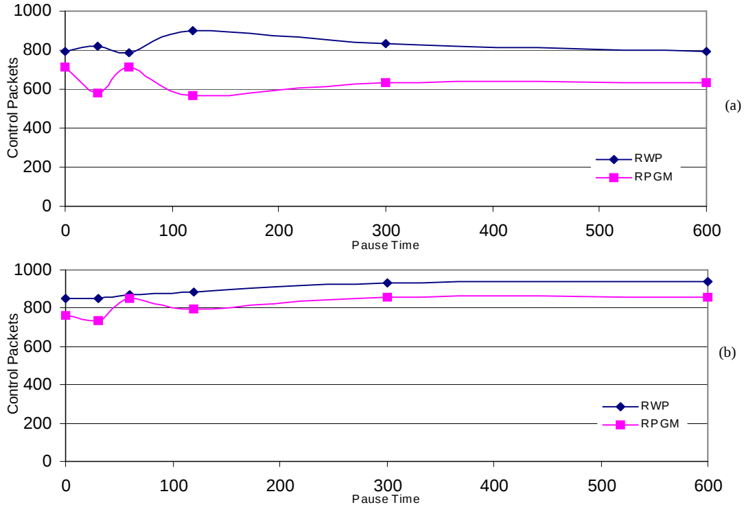
Figure 5.33 Average Control Overhead with the Two Mobility Models: (a) 1 Source and 10 Multicast Receivers and (b) 3 Sources and 3 Multicast Receivers per Source
