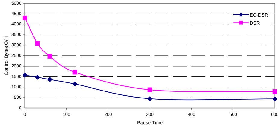
Figure 4.7 Bytes Control Overhead
