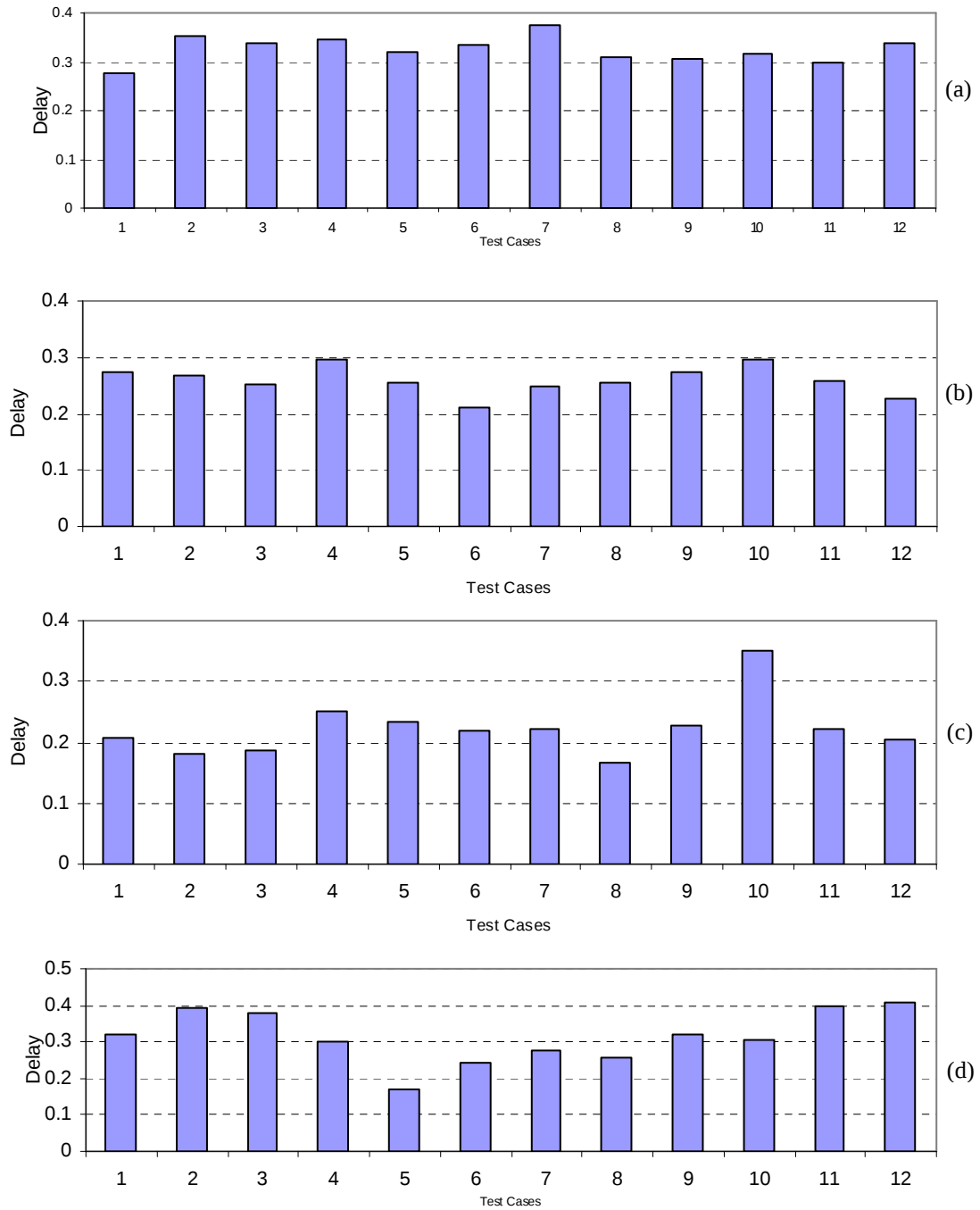
Figure 6.5 End-to-End Delay: (a) Pause Time 0, (b) Pause Time 30, (c) Pause Time 300 and (d) Pause Time 600
