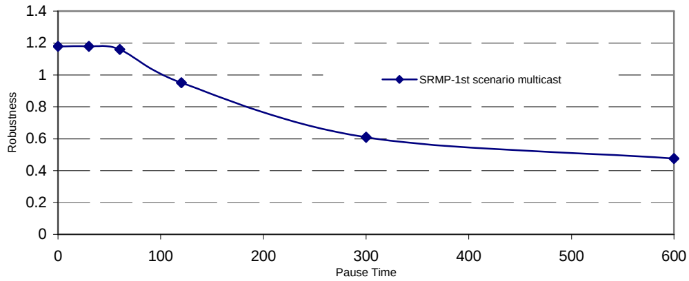
Figure 5.16 SRMP Robustness (1st Multicast Scenario)
