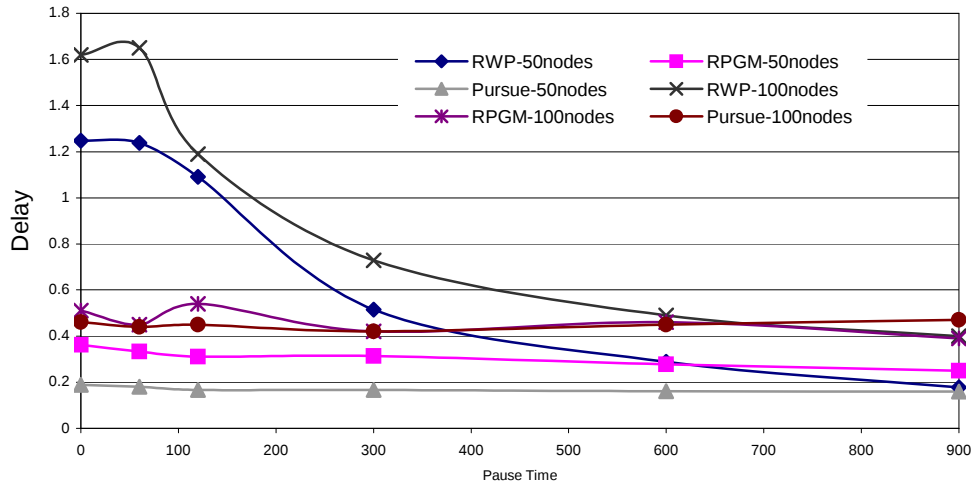
Figure 4.13 EC-DSR Average Delay
