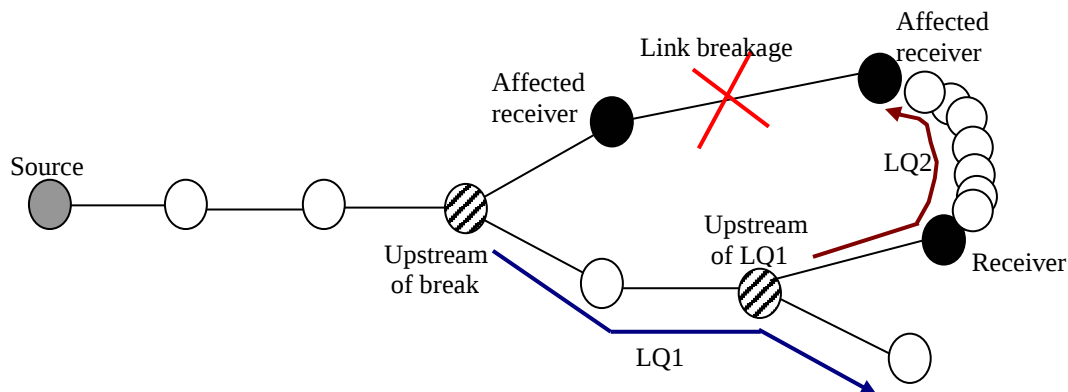
Figure 3.6 ABAM Tree Re-establishment
