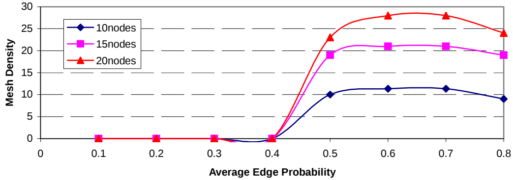
Figure 7.2 Small Size Graph: Average Edge Probability versus Mesh Density
