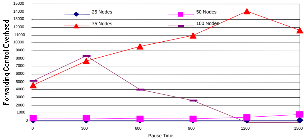
Figure 4.9 EC-DSR versus DSR Absolute Control O/H
