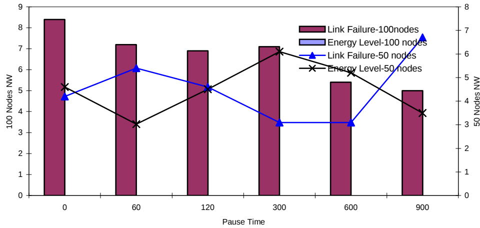
Figure 4.19 PM Energy Level Vs Link Failure
