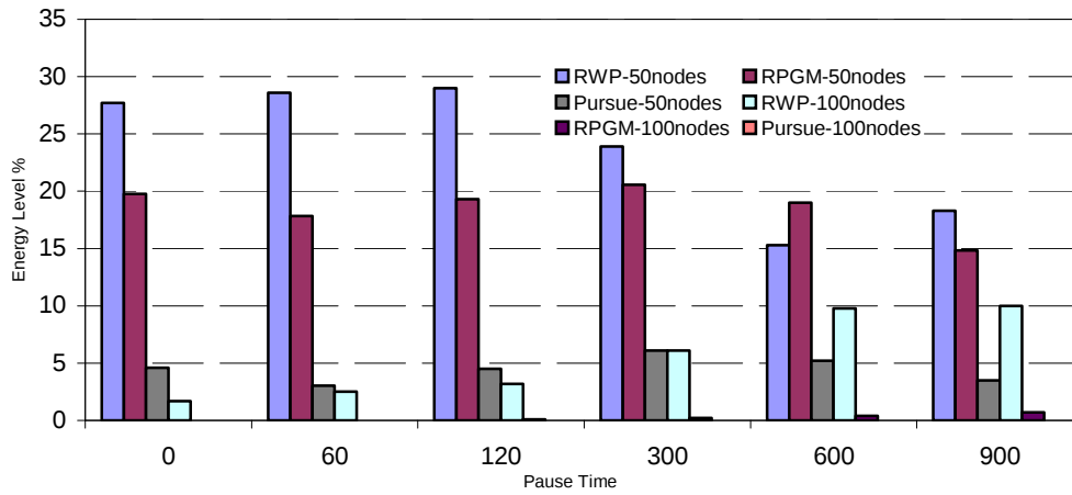
Figure 4.16 EC-DSR Average Energy Level
