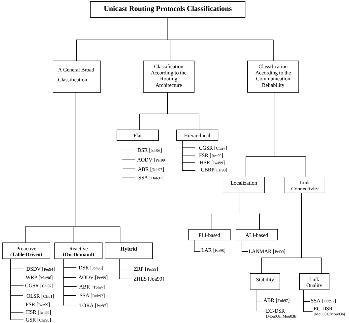
Figure 2.1 Ad hoc Routing Protocols Different Classifications
