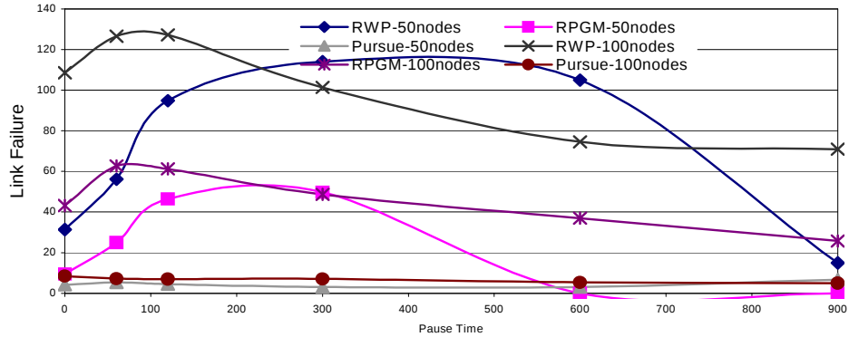
Figure 4.15 EC-DSR Average Link Failure Rate
