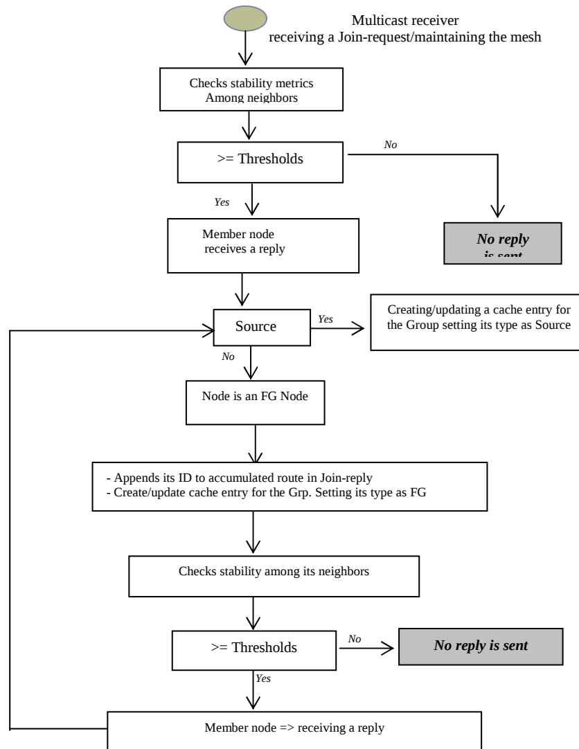
Figure 5.3 Reply Phase and Mesh Establishment
