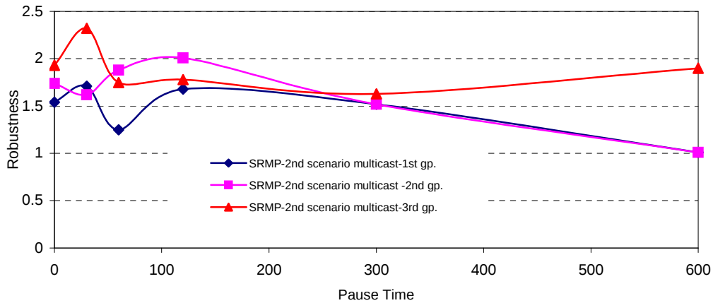
Figure 5.17 SRMP Robustness (2nd Multicast Scenario)
