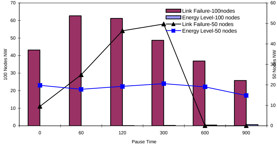
Figure 4.18 RPGM Energy Level Vs Link Failure
