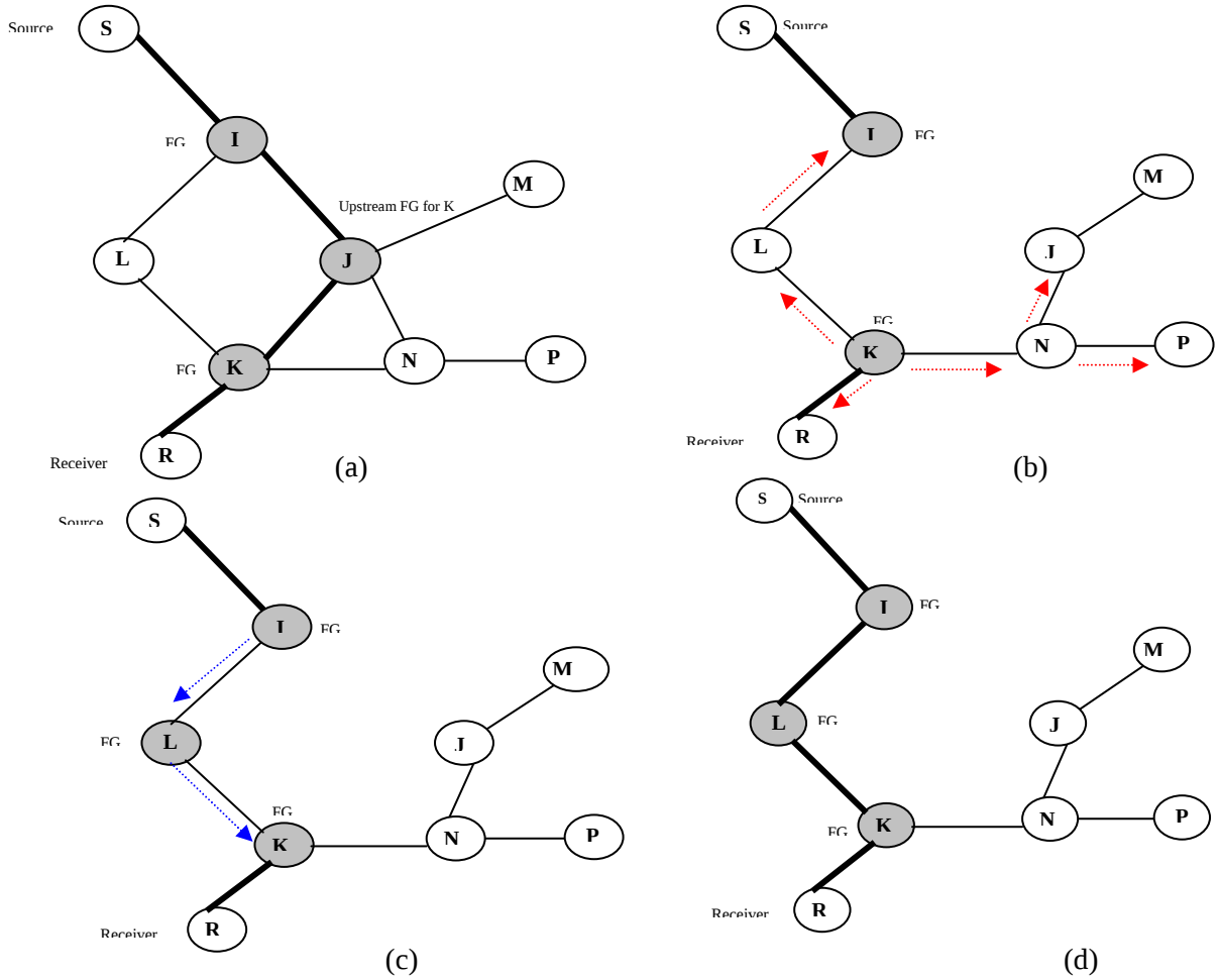
Figure 3.9 Example of PatchODMRP Operation: (a) ODMRP mesh, (b) J unreachable from K, (c) PATCH packet from I to K and (d) K marking L as FG node
