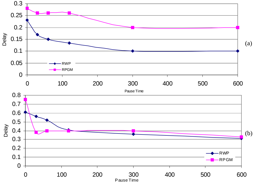
Figure 5.32 Average End-to-End Delay with The Two Mobility Models: (a) 1 Source and 10 Multicast Receivers and (b) 3 Sources and 3 Multicast Receivers per Source
