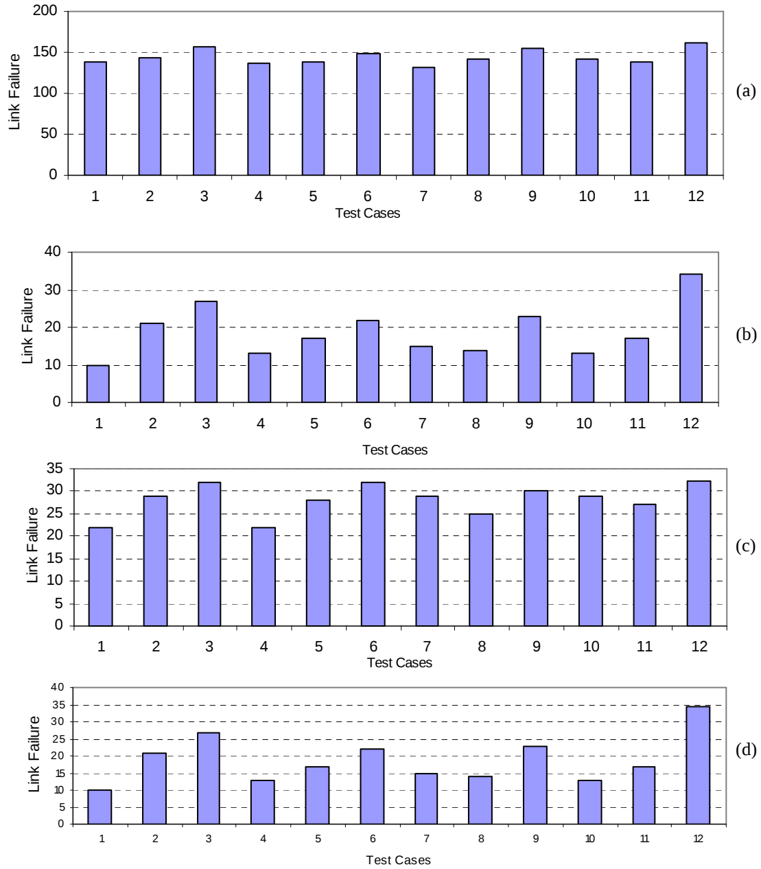
Figure 6.9 Link Failure: (a) Pause Time 0, (b) Pause Time 30, (c) Pause Time 300 and (d) Pause Time 600
