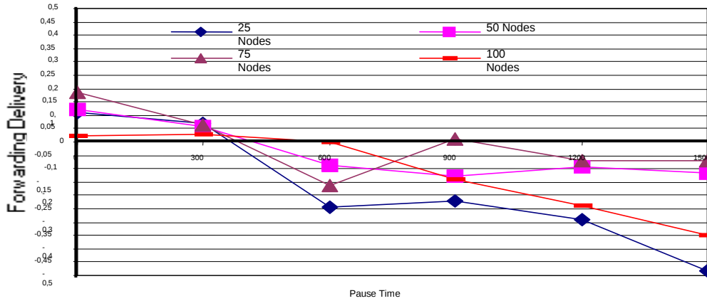
Figure 4.11 EC-DSR Vs DSR Absolute Forwarding Delivery
