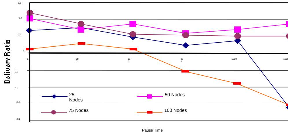
Figure 4.10 EC-DSR versus DSR Absolute Delivery Ratio
