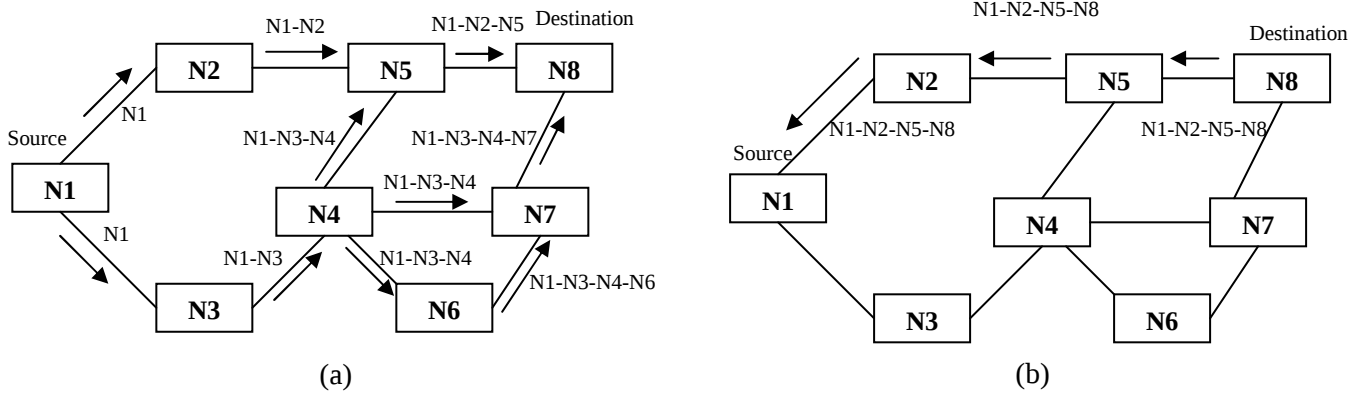
Figure 2.3 Creation of the Route Record in DSR: (a) Route record construction during route discovery, (b) Propagation of RREP
