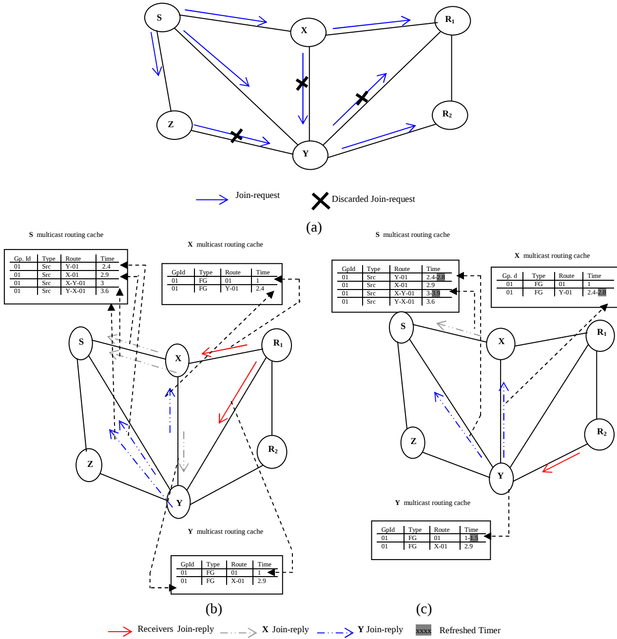
Figure 5.6 : A Small Network Running SRMP: (a) Join-request generation by S, (b) Join-reply generation by R 1 to S, and (c): Join-reply generation by R 2 to S
