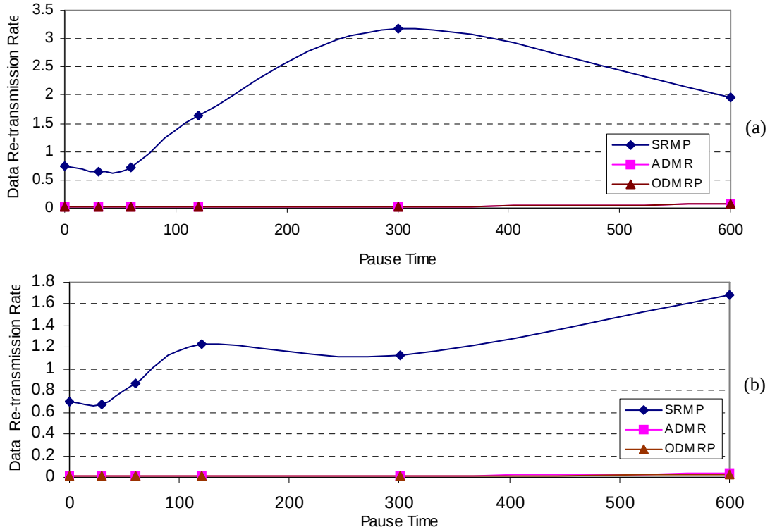
Figure 5.24 Data Re-transmission Rate: (a) 1 Multicast Group Case, (b) 3 Multicast Groups Case
