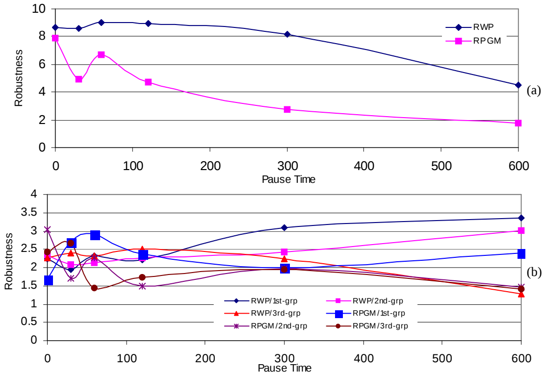
Figure 5.36 Average Nodes Robustness with the Two Mobility Models: (a) 1 Source and 10 Multicast Receivers and (b) 3 Sources and 3 Multicast Receivers per Source
