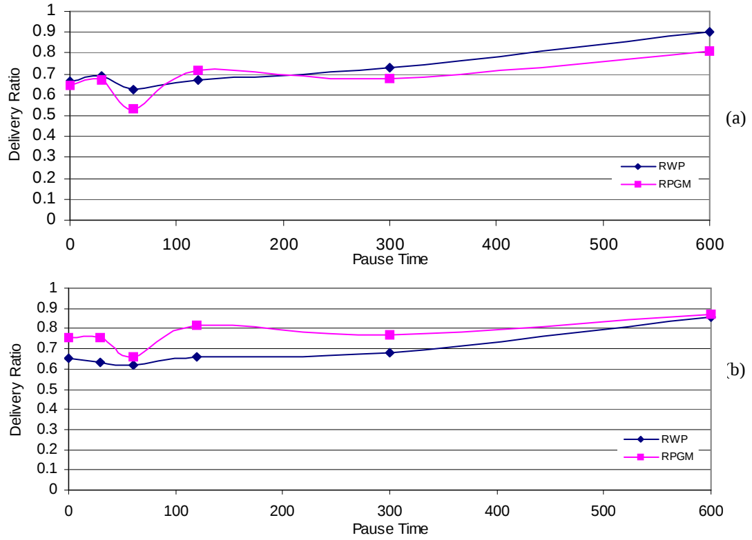
Figure 5.31 Average Delivery Ratio with the Two Mobility Models: (a) 1 Source and 10 Multicast Receivers and (b) 3 Sources and 3 Multicast Receivers per Source
