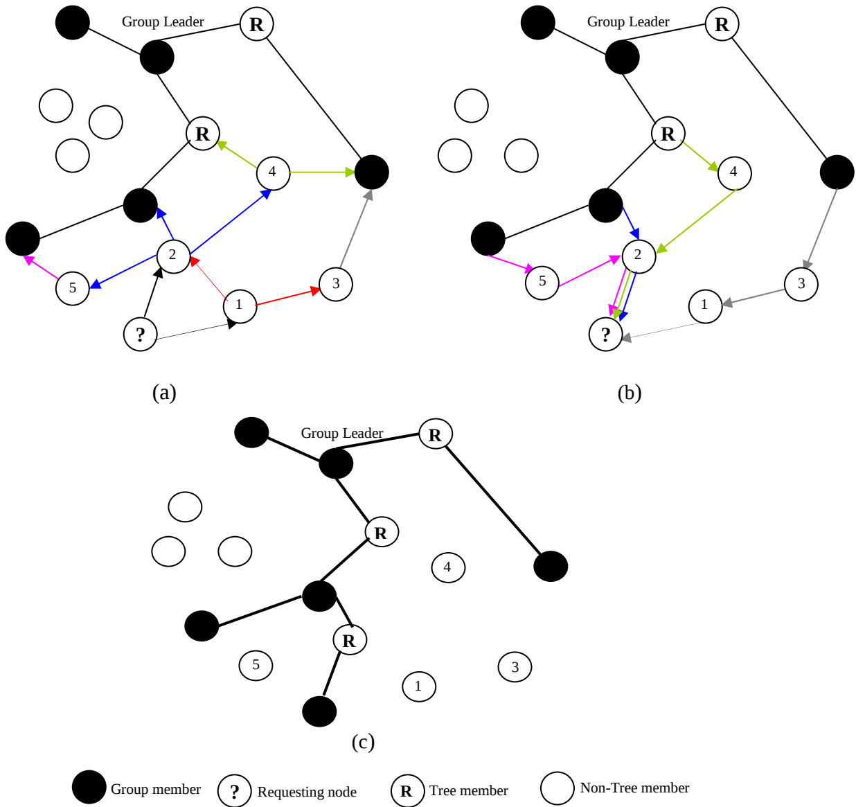
Figure 3.5 Multicast RREQ / RREP Cycle: (a) RREQ Propagation, (b) RREP Propagation and (c) Multicast Tree Creation
