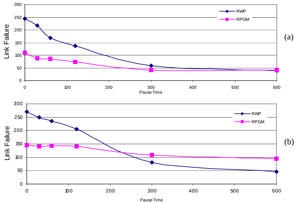
Figure 5.34 Link Failure Rate with the Two Mobility Models: (a) 1 Source and 10 Multicast Receivers and (b) 3 Sources and 3 Multicast Receivers per Source
