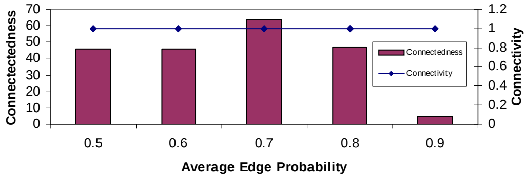
Figure 7.6 10-Node Graph: Average Edge Probability versus Receiver Connectedness and Connectivity
