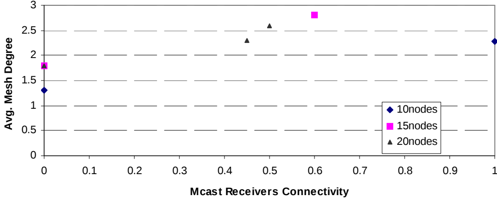
Figure 7.5 Small Size Graph: Multicast Receivers Connectivity versus Average Mesh Degree
