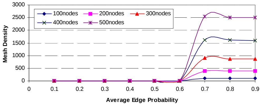
Figure 7.9 Large Scale Graph: Average Edge Probability versus Mesh Density
