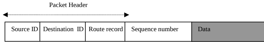
Figure 5.4 Data packet format
