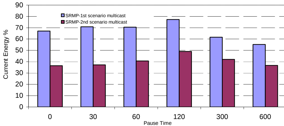
Figure 5.18 Energy Level (Both Multicast Scenario)
