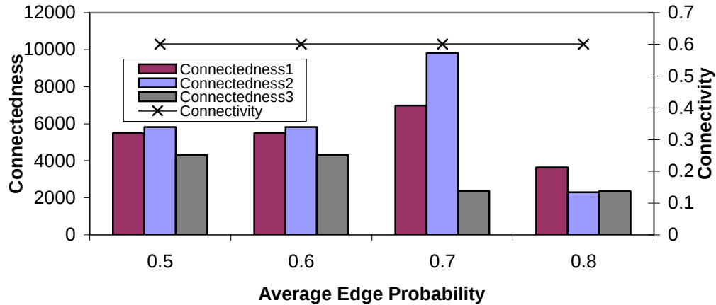
Figure 7.7 15-Node Graph: Average Edge Probability versus Receivers Connectedness and Connectivity
