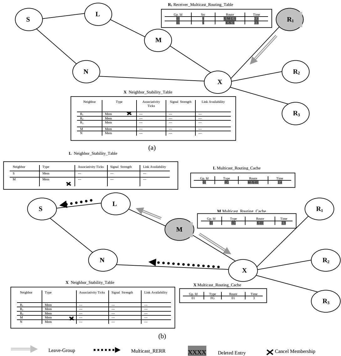
Figure 5.12A Pruning Example: (a) Multicast Receiver Pruning, (b) An FG Node Pruning
