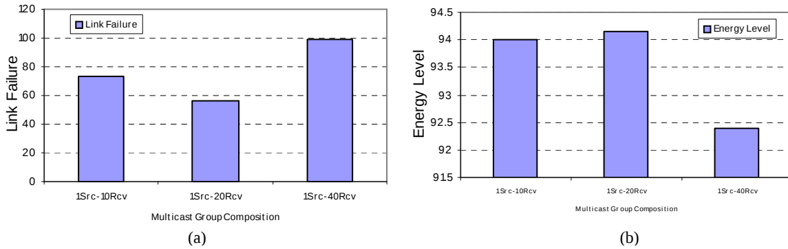
Figure 5.27 Different Multicast Group Composition: (a) Link Failure (b) Energy Level
