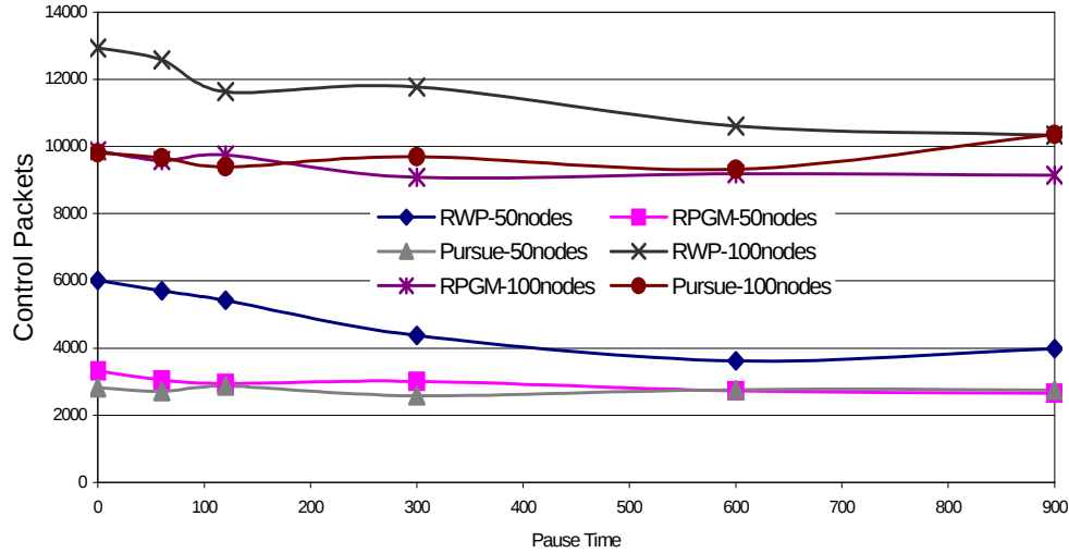
Figure 4.14 EC-DSR Average Control Overhead
