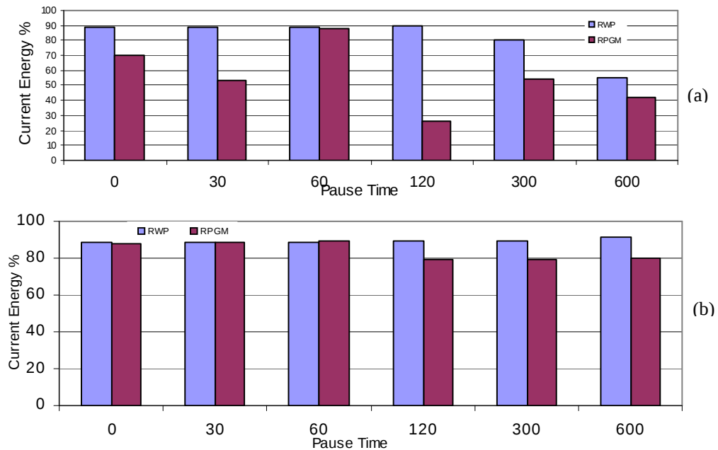
Figure 5.35 Energy Level with the Two Mobility Models (a) 1 Source and 10 Multicast Receivers and (b) 3 Sources and 3 Multicast Receivers per Source
