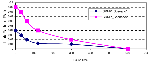
Figure 5.15 SRMP Link Failure Rate (Both Multicast Scenario)
