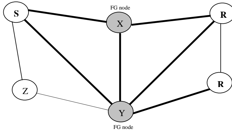
Figure 5.7 Mesh Creation
