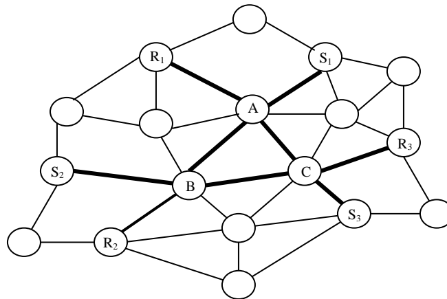
Figure 3.7 Join-Reply Forwarding
