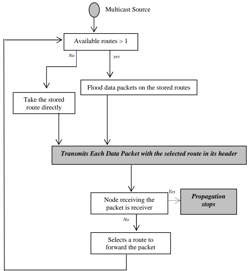
Figure 5.5 Data Forwarding
