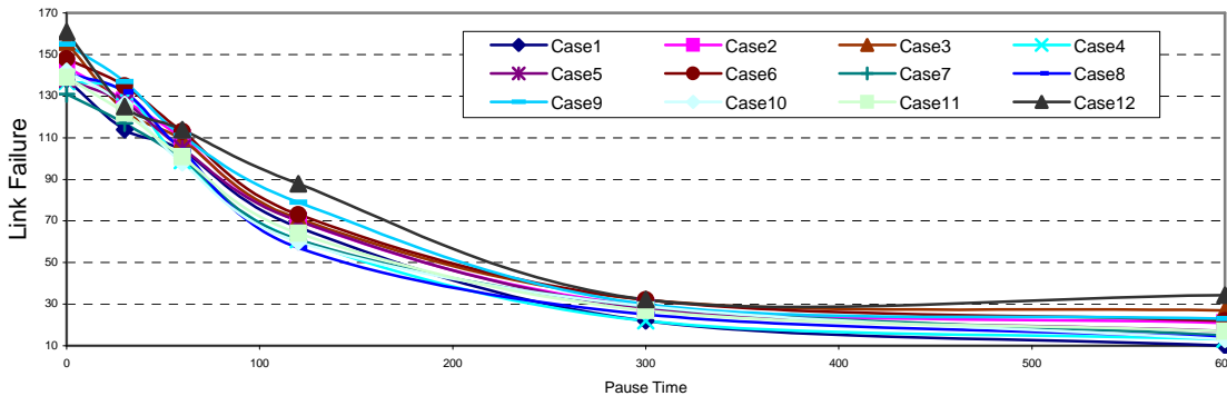
Figure 6.8 Link Failure
