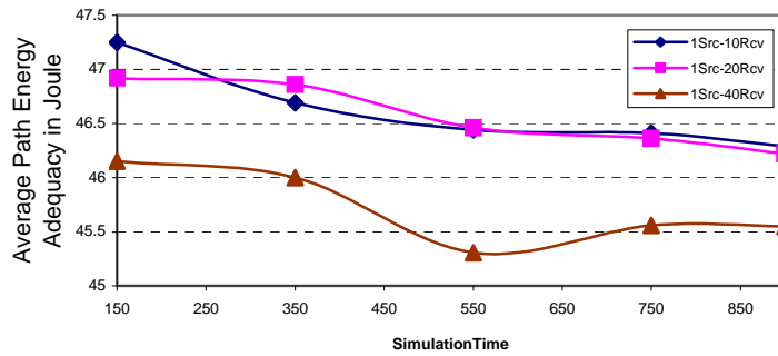
Figure 5.26 1 Multicast Group Cases: Average Path Energy
