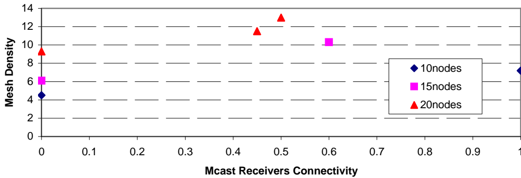
Figure 7.4 Small Size Graph: Multicast Receivers Connectivity versus Mesh Density
