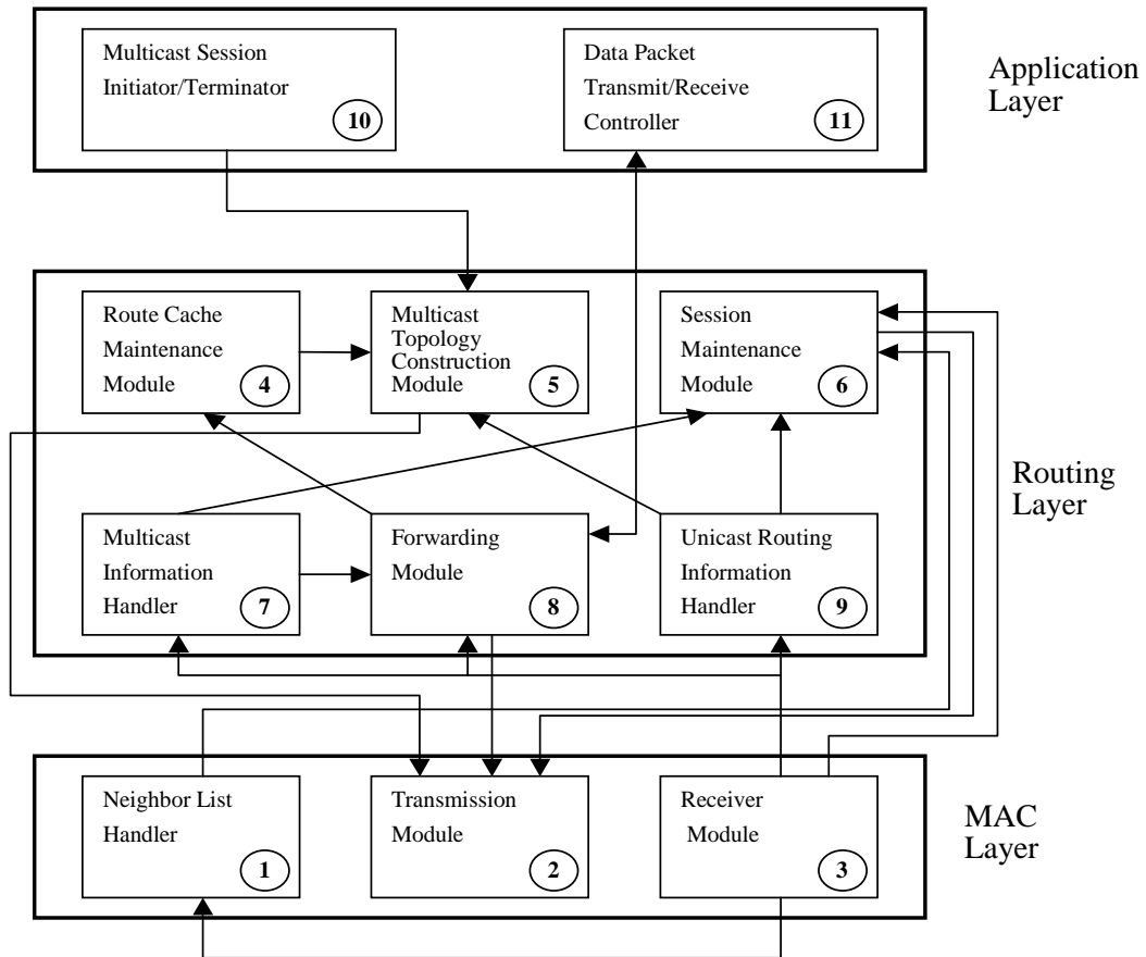
Figure 3.3 Architectural Framework of an Ad hoc Multicast Protocol
