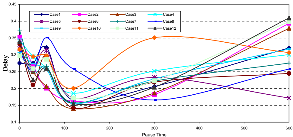
Figure 6.4 End-to-End Delay
