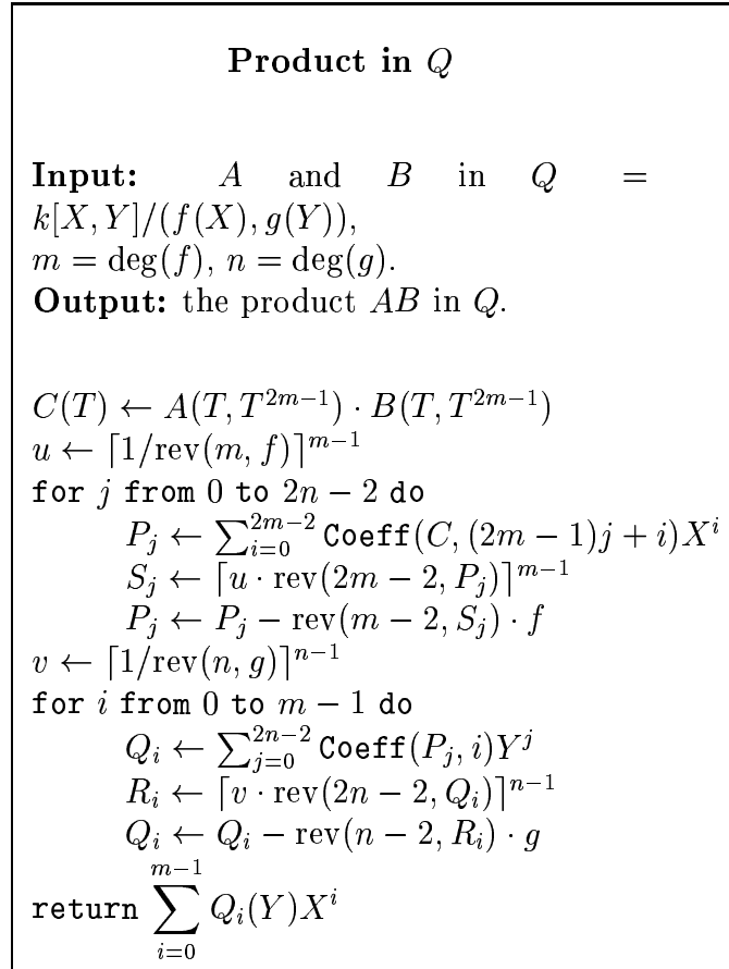
Figure 7.9: Bivariate modular multiplication
