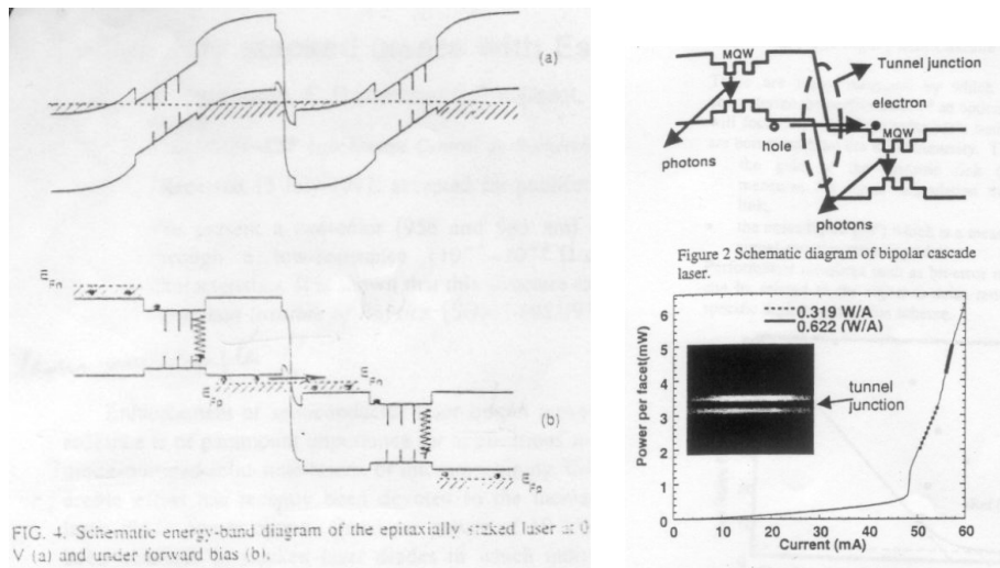
(a) A BCL proposed by Garcia et al. [26]
