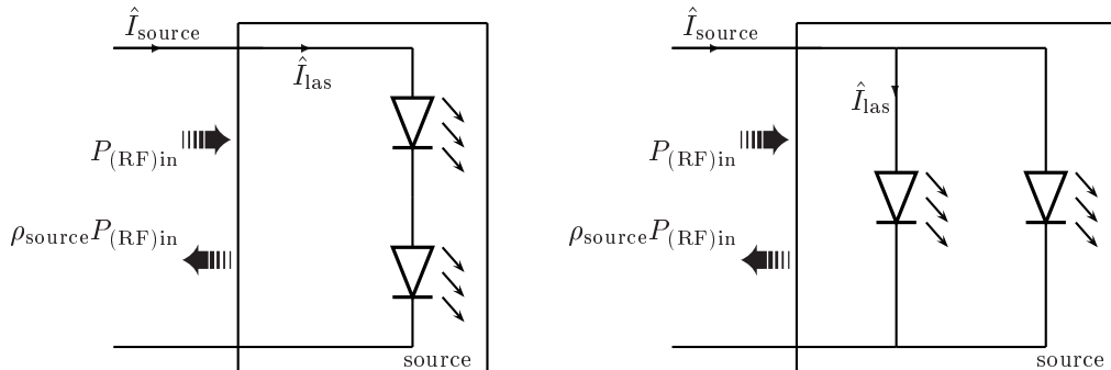
Figure 2.11 Electronic scheme of a (a) series-connected and (b) parallel-connected laser source with no impedance matching
