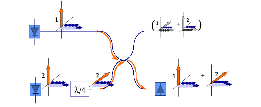
Figure 2.30 Proposed set-up for a more robust implementation in systems [8].
