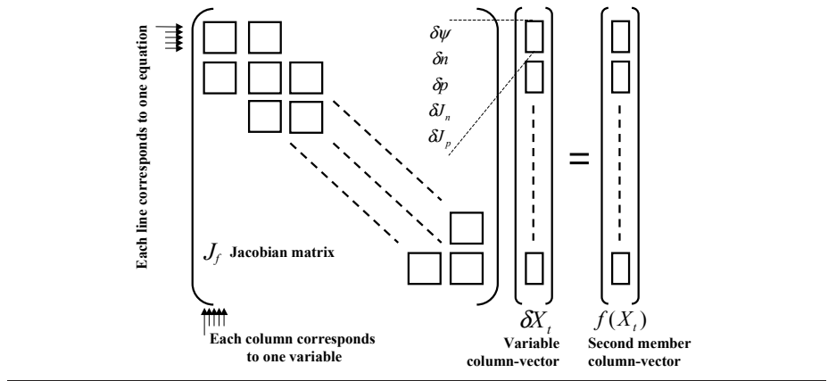
Figure 4.3 Schematical description of the Newton method used for fast convergence.
