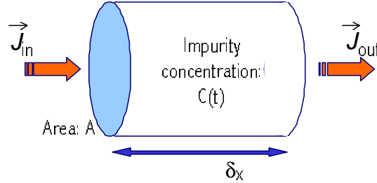
Figure 5.6 Schematic representation of a volume element through which a flow of particles diffuses
