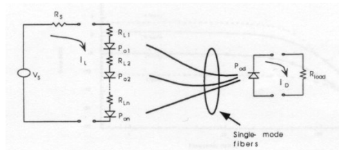
Fig. 1 Directly-modulated analog link with series-connected lasers
