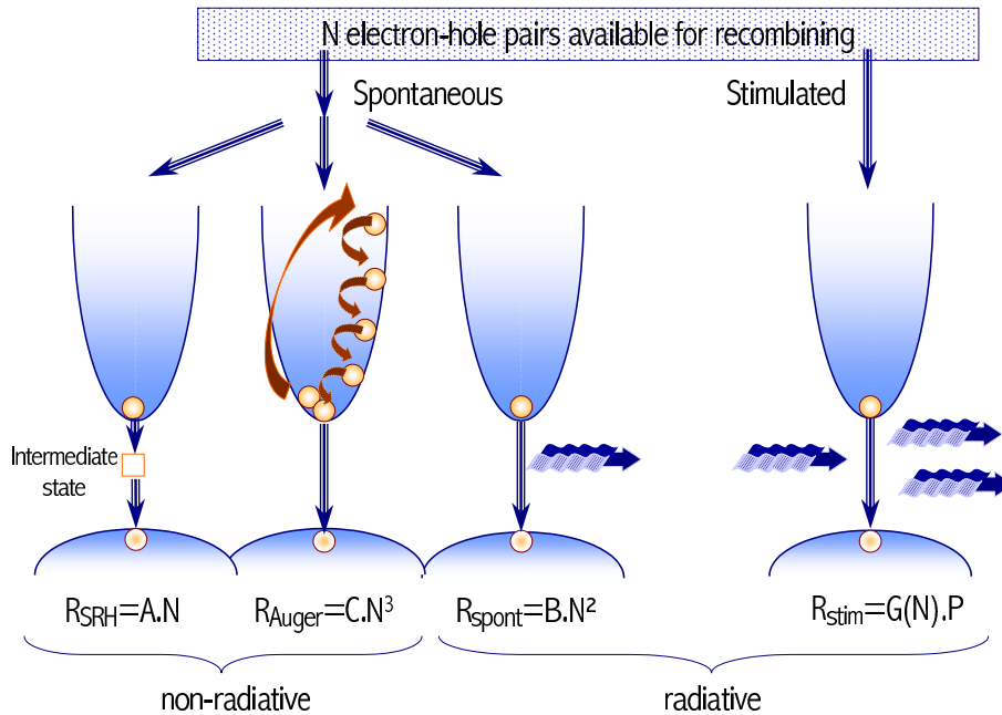
Figure 3.3 Summary of the different type of recombinations in a semi-conductor laser
