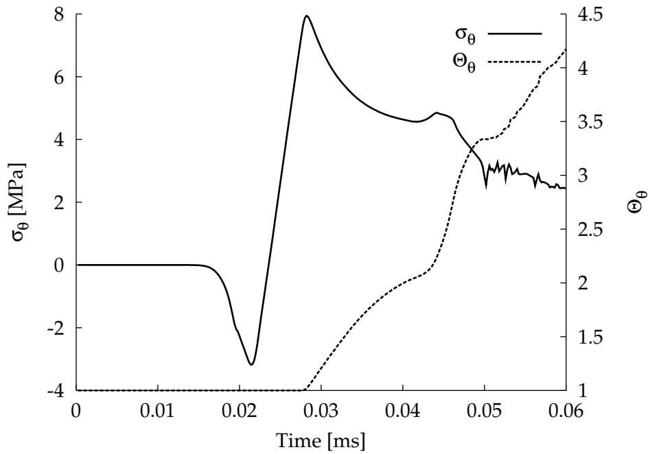
Figure III.10: Tangential stress and tangential damage as a function of time at the medium of sample (A)
