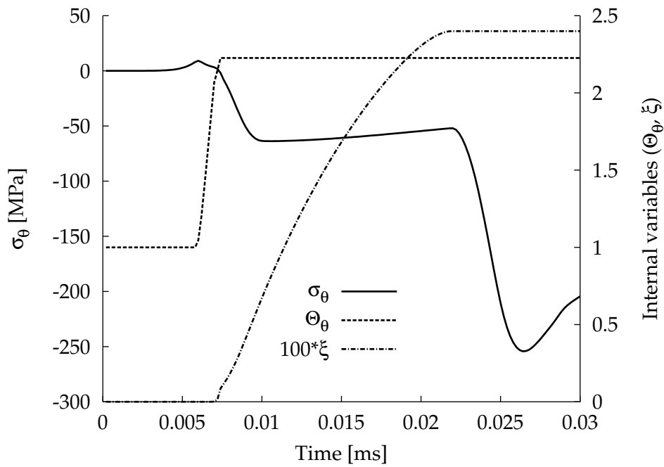
Figure III.9: Tangential stress, tangential damage and the softening variable as a function of time at the inner surface of sample (C)
