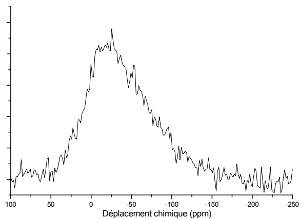
Figure A.IV.2 : Spectre ^{71}\text{Ga} RMN MAS de la hollandite \text{Ba}_{1,28}\text{Al}_{1,64}\text{Ga}_{0,92}\text{Ti}_{5,44}\text{O}_{16} ( B_0=11,75\text{ T} , \nu_R=31500\text{ Hz} ).
