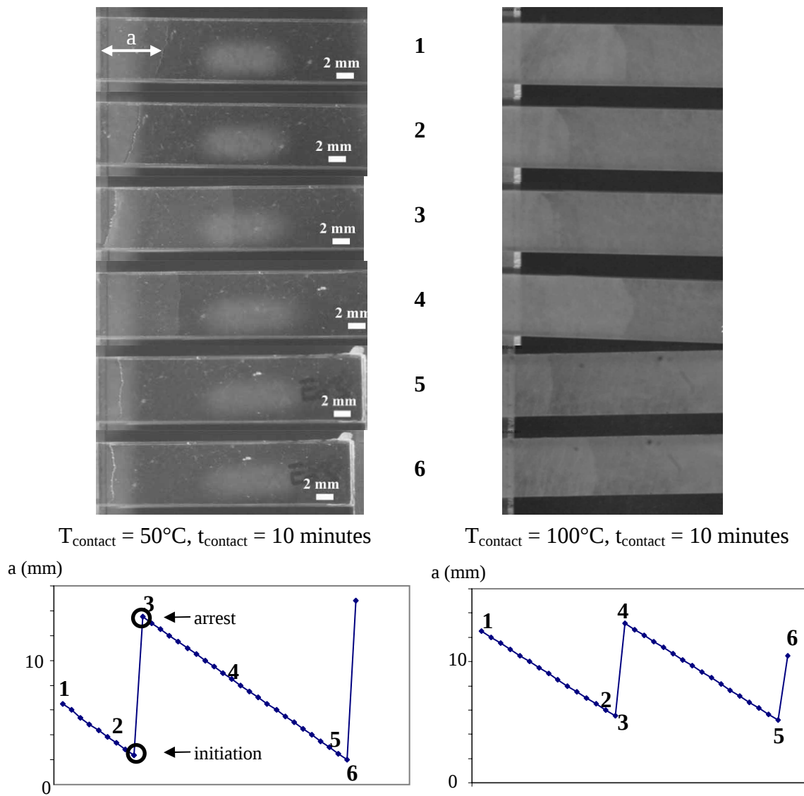
Figure 3.4-9: “unstable” crack growth in the case of a contact at 50°C and 100°C for 10 minutes. Test carried out at 10 °C.
