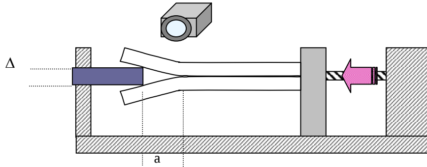
Figure 2.4-11: double cantilever beam test
