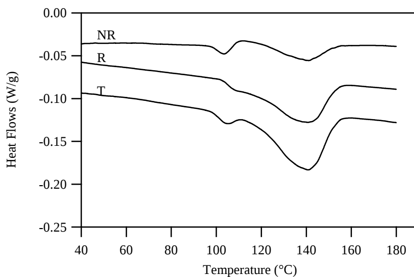
Figure 3.2-8: TM-DSC results for 45PB scan at 5^{\circ}\text{C}.\text{min}^{-1} , with oscillations of 0.796^{\circ}\text{C} every 60s (Heat Only). Total (T), Reversing (R) and non-reversing heat flow vs. temperature.
