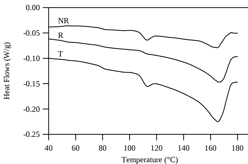
Figure 3.2-7: TM-DSC results for 35PB scan at 5^{\circ}\text{C}.\text{min}^{-1} , with oscillations of 0.796^{\circ}\text{C} every 60s (Heat Only). Total (T), Reversing (R) and non-reversing heat flow vs. temperature.
