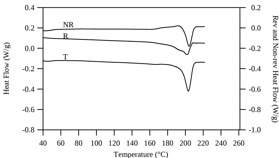
Figure 3.1-6 : MDSC results for 15PB scanned at 5^{\circ}\text{C}.\text{min}^{-1} , with oscillations of \pm 0.796^{\circ}\text{C} every 60 s (Heat Only). Total (T), Reversing (R) and nonreversing heat flows vs. temperature.
