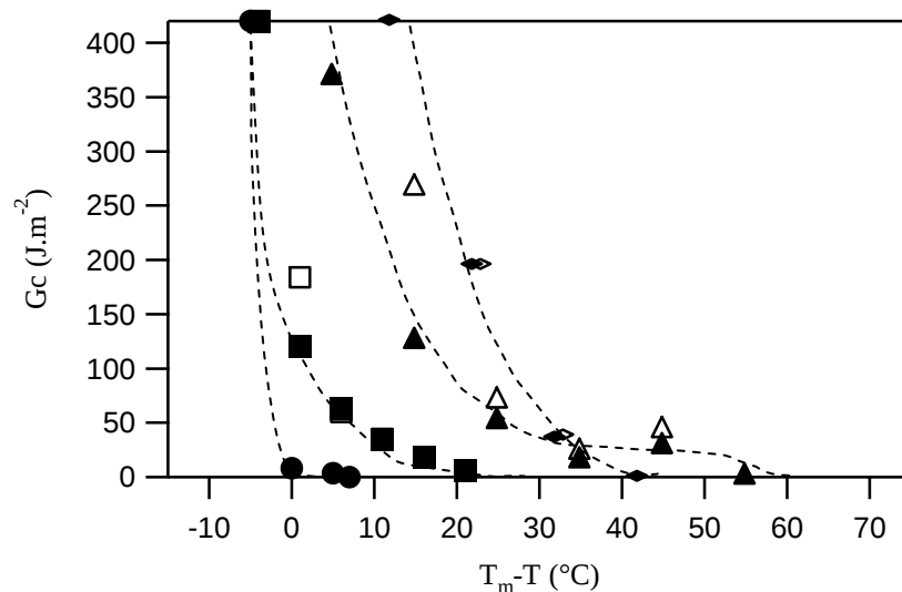
Figure 4.1-3 : fracture toughness as a function of T_m - T for PBT ●, 15PB ■, 35PB ▲ and 45PB ◆ for 10 minutes of contact (full symbols) and 30 minutes of contact (open symbols)
