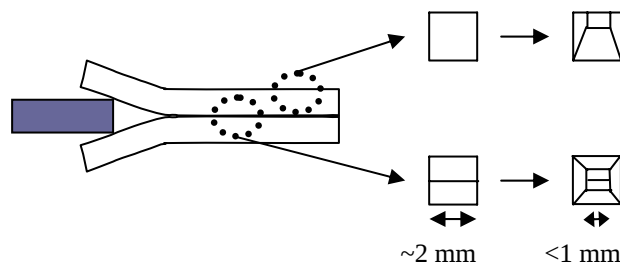
Figure 2.6-1 : sample preparation → surface and interface observations
