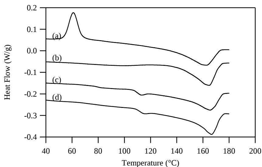
Figure 3.2-5: total heat flow as a function of temperature for 35PB scanned at 5^{\circ}\text{C}.\text{min}^{-1} (a) standard procedure (polymer granule heated at 260^{\circ}\text{C} and cooled at 5^{\circ}\text{C}.\text{min}^{-1} ) (b) from a polymer plate molded at 180^{\circ}\text{C} and cooled at 2.5^{\circ}\text{C}.\text{min}^{-1} (c) from a polymer plate molded, then annealed at 100^{\circ}\text{C} for 25 min. (d) from a polymer plate molded, then annealed at 100^{\circ}\text{C} for 55 min.
