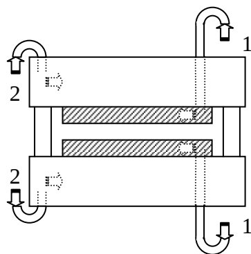
Figure 2.4-2: press primary and secondary coolant circuit 1 \rightarrow \varnothing / water / air ; 2 \rightarrow \varnothing / water
