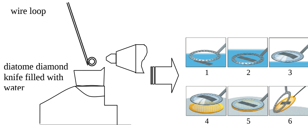
Figure 2.6-4: Ultramicrotome equipped with a diatome diamond knife.
