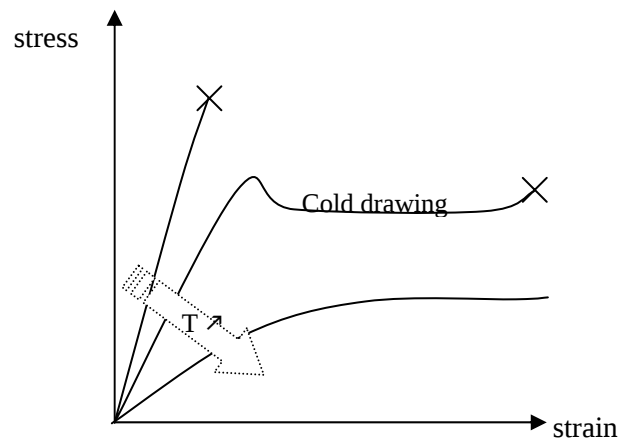
Figure 1.1-14 : schematic stress/strain curves for crystalline polymers
