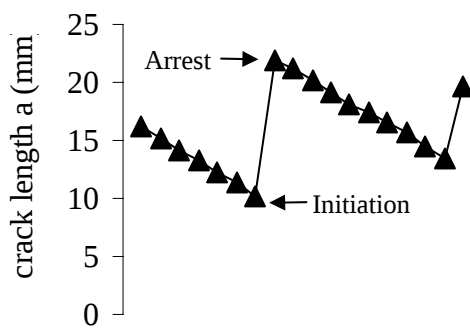
Figure 3.3-20 : Stick slip behavior during the DCB test (carried out at 15^{\circ}\text{C} ).
