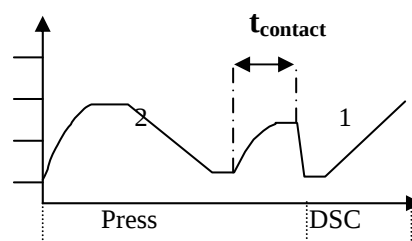
Figure 3.3-2 different thermal histories undergone by the samples before scanning at 5^{\circ}\text{C}.\text{min}^{-1} . The main ramps are 1 : 5^{\circ}\text{C}.\text{min}^{-1} and 2 : 2.5^{\circ}\text{C}.\text{min}^{-1}
