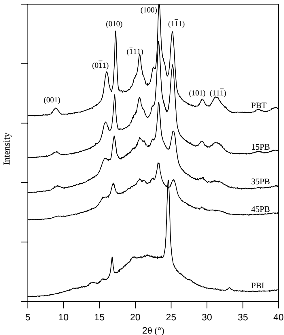
Figure 2.3-9 : Diffraction patterns of melt-crystallized PBT, 15PB, 35PB at a cooling rate of 2.5^{\circ}\text{C}.\text{min}^{-1} and cold crystallized 45PB and PBI at 100^{\circ}\text{C} for 120 min. Miller indices are shown on the diffraction peaks of PBT.
