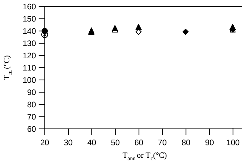
Figure 3.3-11: melting point samples annealed ▲ or assembled ◆ for 10 minutes samples annealed △ or assembled ◇ for 60 minutes sample not annealed ● and standard procedure ⊗
