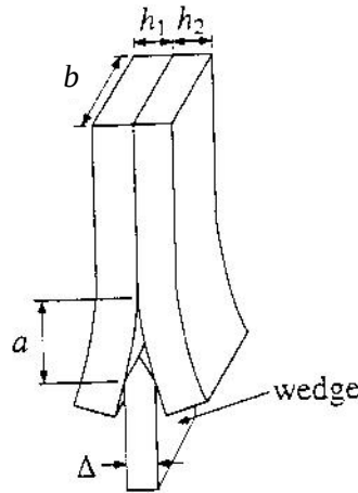
Figure 1.2-7 : the double cantilever beam geometry with a constant opening displacement.
