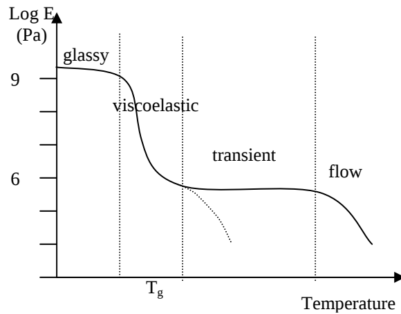
Figure 1.1-4: variation of E for an amorphous polymer
