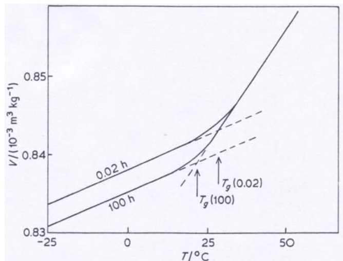
Figure 1.1-2 : variation of the specific volume of poly(vinyl acetate) with temperature taken after two different times (After Kovacs 1 )
