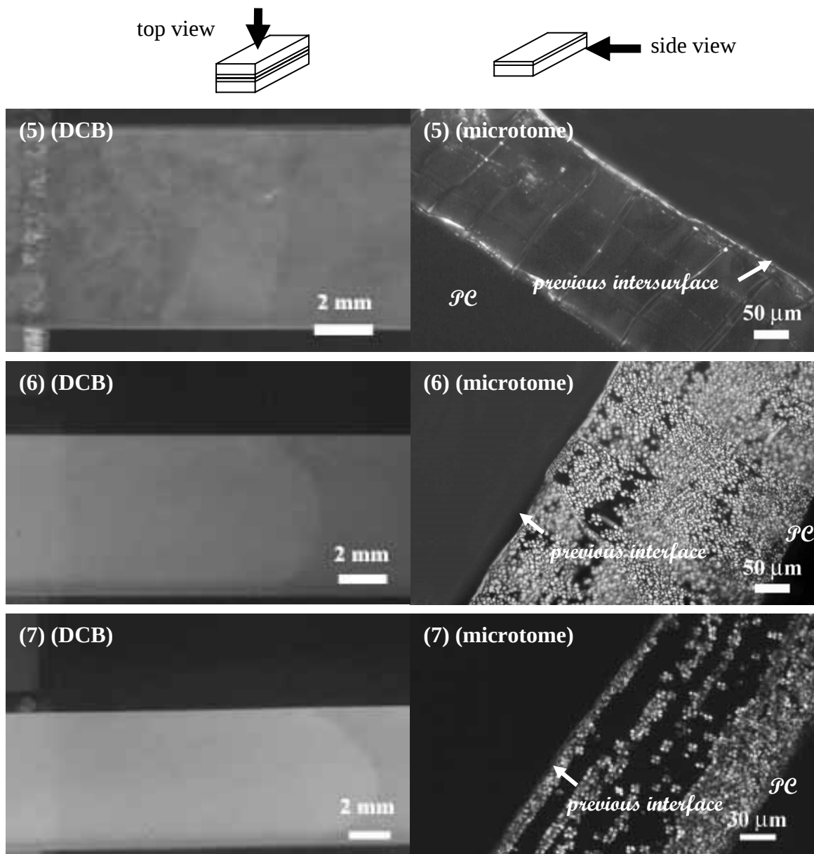
Figure 3.4-7: images from DCB test and optical micrographs of microtomed samples. 1 : molded sample (reference sample) ; 2 : assembled at 60°C for 10 minutes ; 3 : assembled at 70°C for 10 minutes ; 4 : assembled at 70°C for 60 minutes ; 5 : assembled at 90°C for 10 minutes ; 6 : assembled at 90°C for 60 minutes and 7 : assembled at 100°C for 60 minutes.
