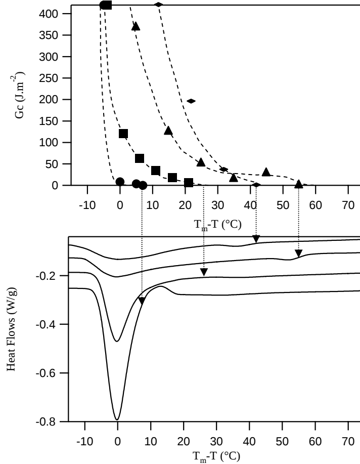
Figure 4.1-1 : fracture toughness as a function of T_m - T for PBT ●, 15PB ■, 35PB ▲ and 45PB ◆, and the corresponding DSC curves, recorded at 5^\circ\text{C.min}^{-1}
