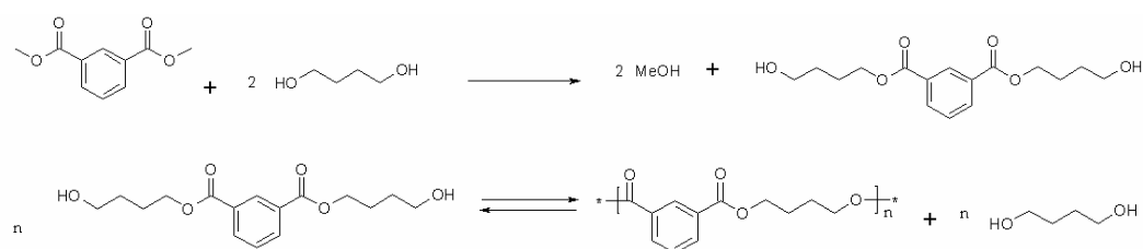
Figure 2.2-1 : two stage polycondensation for the formation of Poly(butylene isophthalate).
