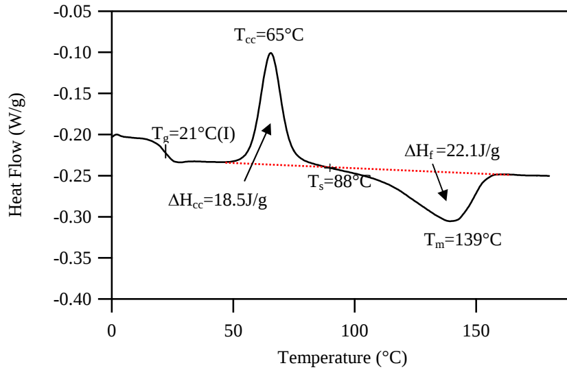
Figure 3.3-5: critical temperatures and characteristic heat capacities for 45PB a annealed at 40°C for 10 minutes.
