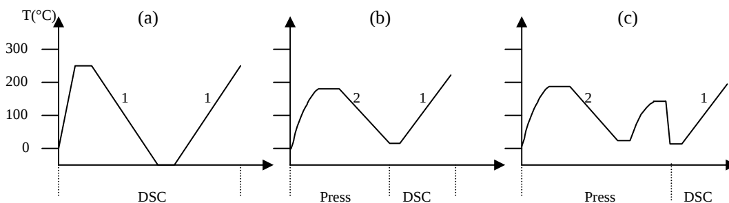
Figure 3.2-4: different thermal history undergone by the samples before scanning in the DSC at 5^{\circ}\text{C}.\text{min}^{-1} . The main ramps are 1 : 5^{\circ}\text{C}.\text{min}^{-1} and 2 : 2.5^{\circ}\text{C}.\text{min}^{-1}
