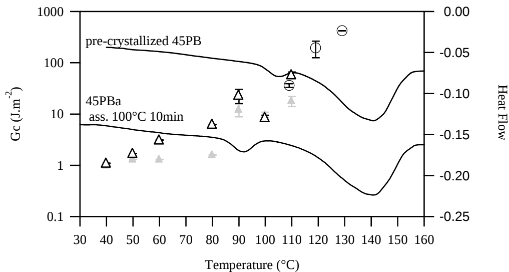
Figure 3.3-23b : DSC curve for 45PB and 45PBa and fracture toughness after 10 minutes contact \blacktriangle and 60 minutes contact \triangle (arrest)
