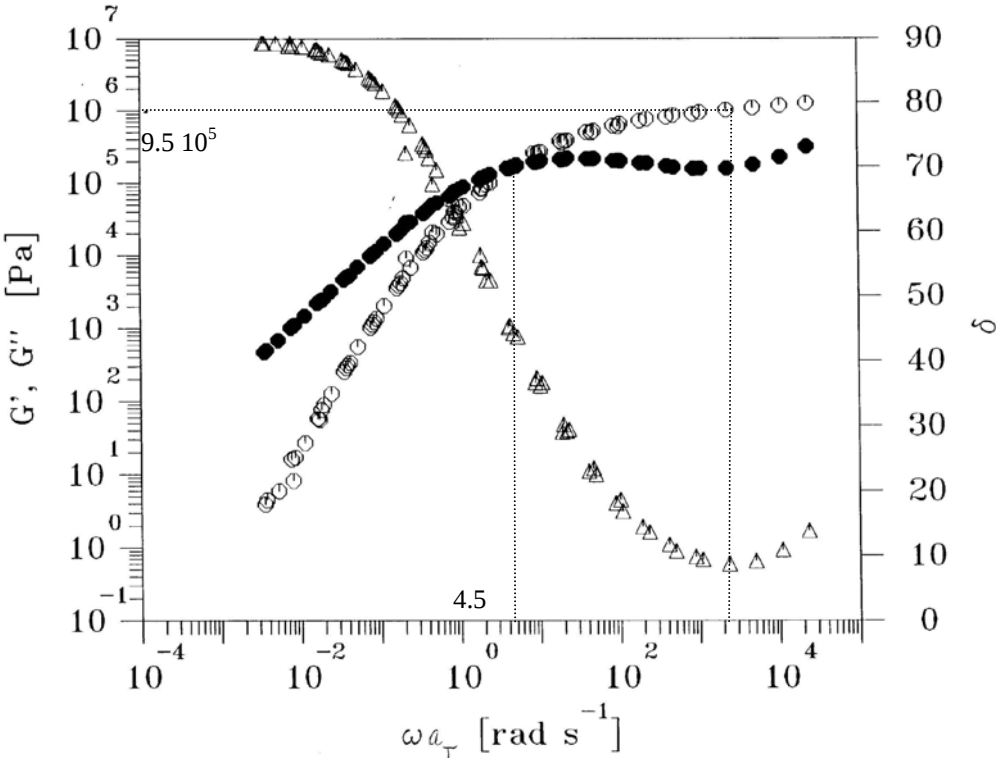
Figure 2.2-5 : time-temperature superposition ( \circ storage modulus G' , \bullet loss modulus G'' and \triangle \tan\delta ) for 45PB ( T_{\text{ref}} = 100^\circ\text{C} ).
