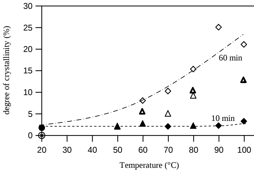
Figure 3.4-4: degree of crystallinity. samples annealed ▲ or assembled ◆ for 10 minutes samples annealed △ or assembled ◇ for 60 minutes samples annealed for 40 minutes ▲ sample unannealed ● and standard procedure ⊗
