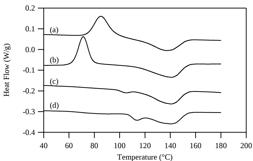
Figure 3.2-6: total heat flow as a function of temperature for 45PB scanned at 5^{\circ}\text{C}.\text{min}^{-1} (a) (b): see Figure 3.2-5 (c) from a polymer plate molded, then annealed at 100^{\circ}\text{C} for 10 min. (d) from a polymer plate molded, then annealed at 100^{\circ}\text{C} for 70 min.
