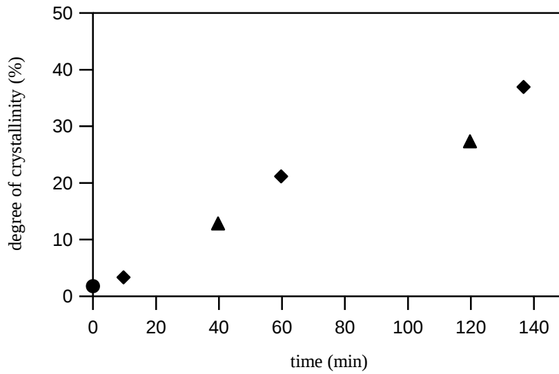
Figure 3.4-5: degree of crystallinity. samples annealed ▲ or assembled ♦ at 100°C sample unannealed ●
