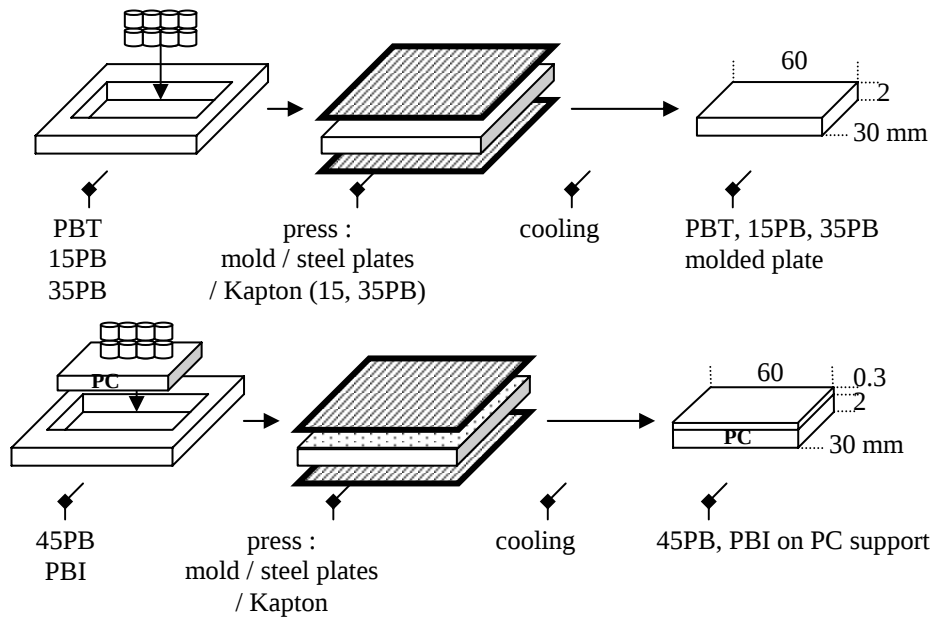
Figure 2.4-3: molding process for each polymer and copolymer
