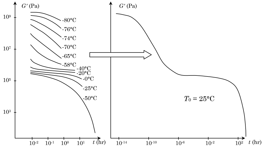
Figure 1.1-5 : Building a master-curve with the time-temperature superposition.
