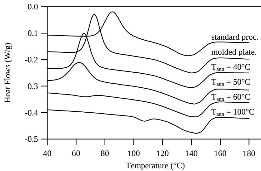
Figure 3.3-3: DSC scans at 5^{\circ}\text{C}.\text{min}^{-1} ; effect of the annealing temperature (annealing time : 10 minutes)
