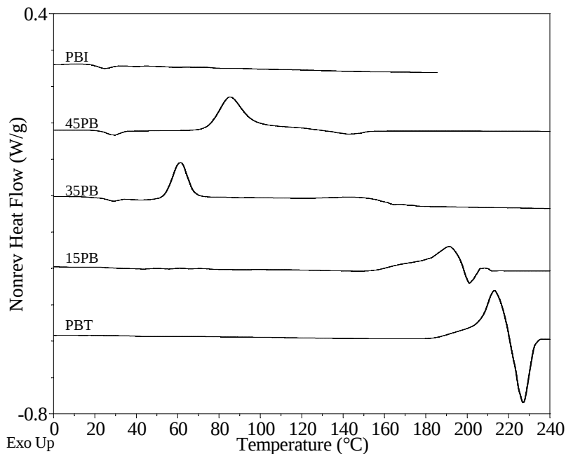
Figure 2.3-4 : nonreversing flow for PBT/BPI samples. Scan ramp : 5^{\circ}\text{C}.\text{min}^{-1} .
