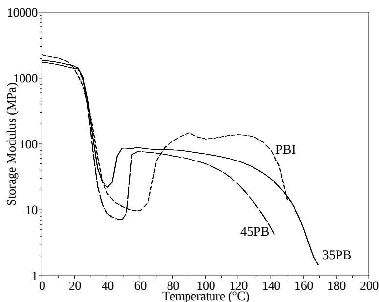
Figure 2.3-8 : storage modulus measured at 1Hz as a function of temperature in the case of quenched samples.
