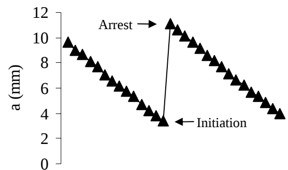
Figure 3.3-20 : Stick slip behavior during the DCB test (carried out at 15^{\circ}\text{C} ).
