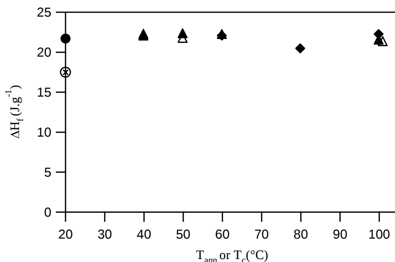
Figure 3.3-12: heat of fusion.
