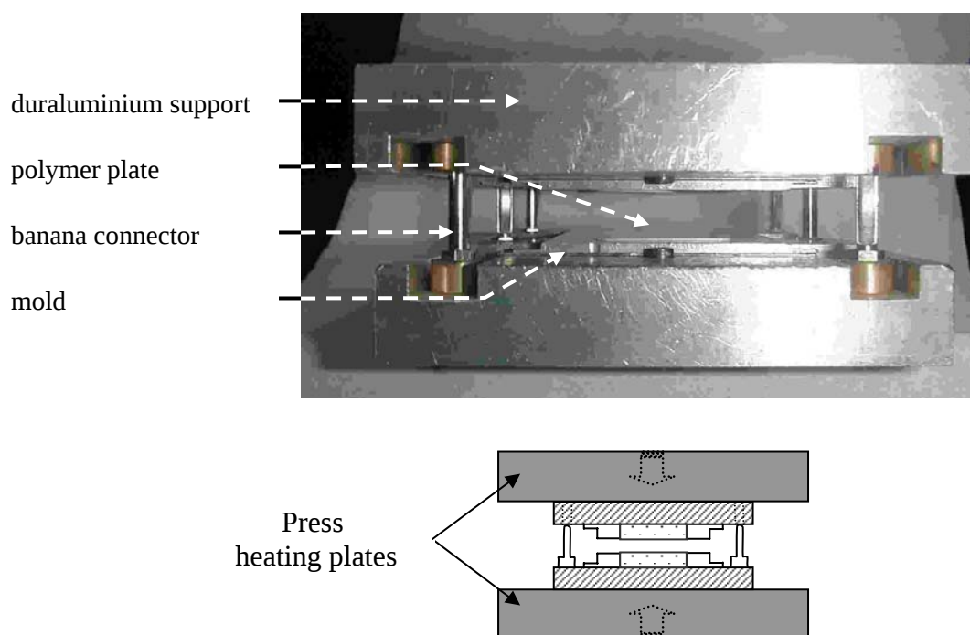
Figure 2.4-6 : home-made set up for assembling under the press
