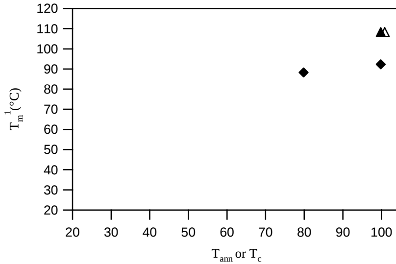
Figure 3.3-10: temperature of the first melting peak. samples annealed ▲ or assembled ◆ for 10 minutes samples annealed △ or assembled ◇ for 60 minutes.
