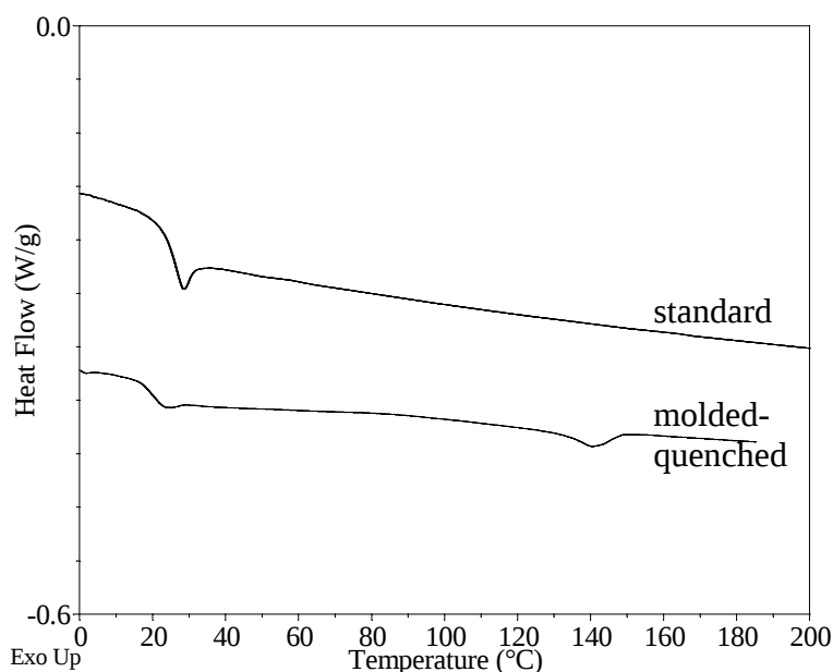
Figure 3.4-1 : DSC scans at 5°C.min -1 : standard procedure and molded-quenched plate (unannealed)
