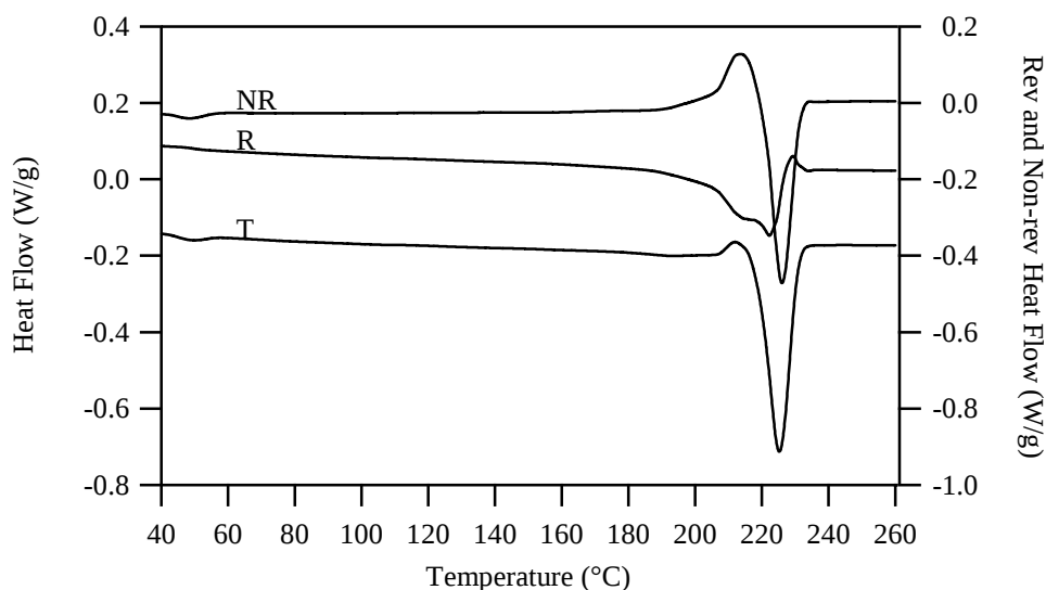
Figure 3.1-5 : MDSC results for PBT scanned at 5^{\circ}\text{C}.\text{min}^{-1} , with oscillations of \pm 0.796^{\circ}\text{C} every 60s (Heat Only). Total (T), Reversing (R) and non-reversing heat flows vs. temperature.
