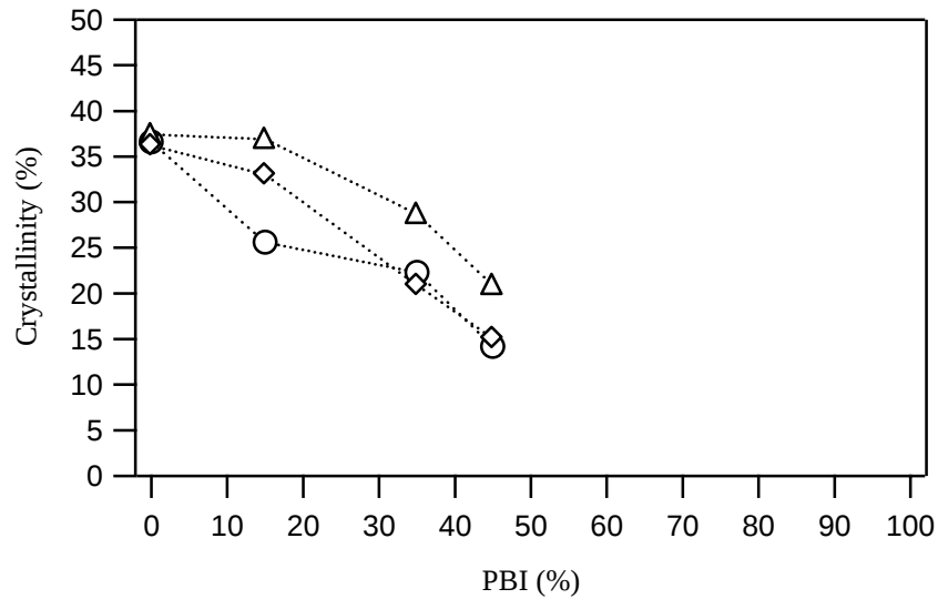
Figure 2.3-11 : degree of crystallinity as a function of PBI content, obtained from X-ray measurements, with the fit function f_1(\diamond) , f_2(\triangle) and obtained by DSC ( \circ )
