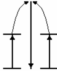
Figure 1. 11. Luminescence coopérative.
