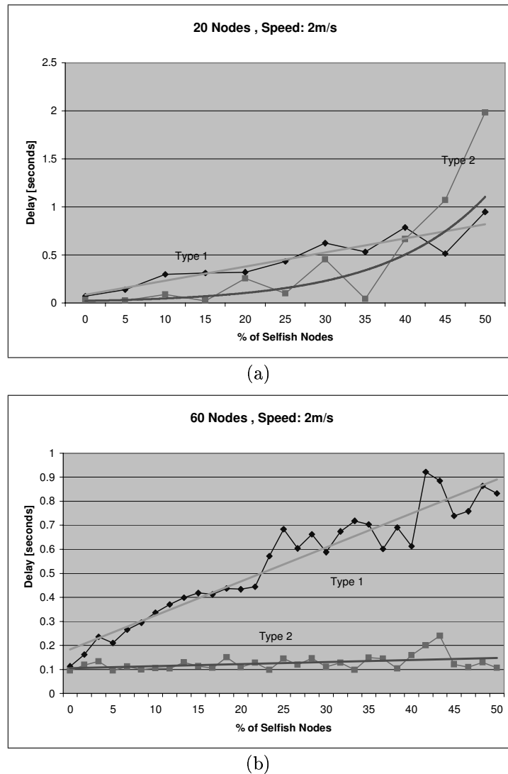
Figure 2.5: d for low and high node density, low mobility
