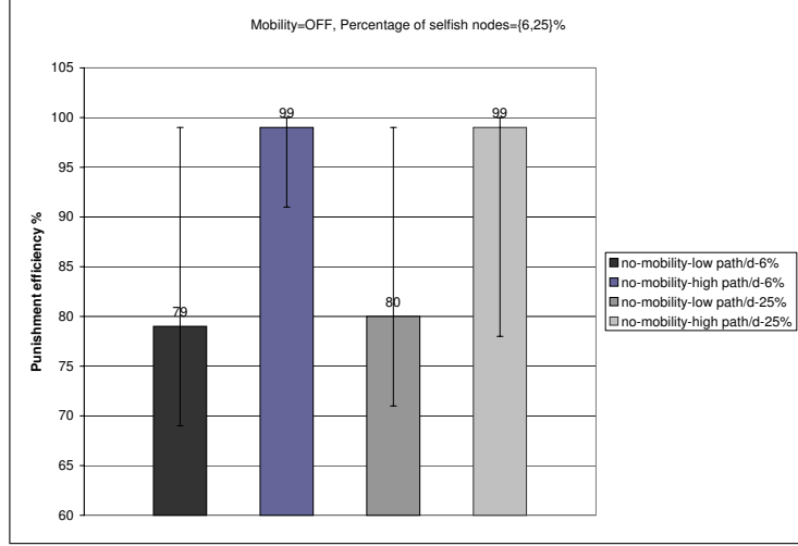
Figure 5.7: p_E for a static network, with measurement errors.
