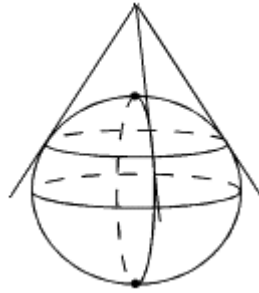
Figure 109: Projection conique
