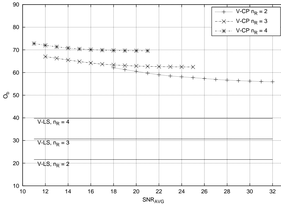
Figure 7.9: O_b as a function of average SNR for V-LS and V-CP (without basis reduction); n_T = 2 , n_R = 2, 3 , and 4 , L = 10 , 16-QAM
