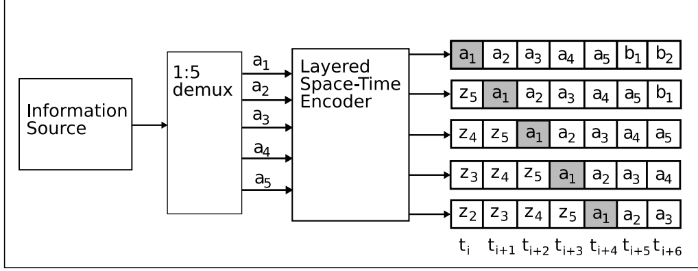
Figure 2.19: Block diagram of a layered space-time coder with five transmit antennas. Seven time intervals are shown. The information stream is demultiplexed into five data streams; here, a_i , 1 \leq i \leq n_T , represent five constellation points. A layered space-time encoder layers each point in space and time; the encoding of point a_1 is highlighted. Symbols z_i represent data from the previous layer, while b_i represent data belonging to the next layer.
