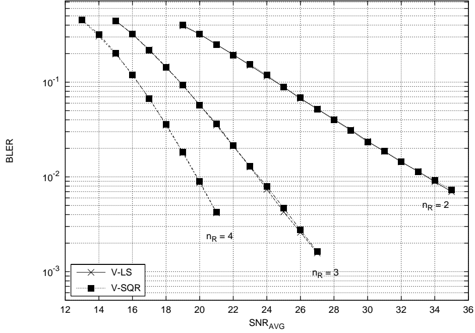
Figure 5.1: BLER as a function of average SNR (dB) for n_T = 2 ; n_R = 2, 3, 4 ; L = 10 ; 16-QAM.
