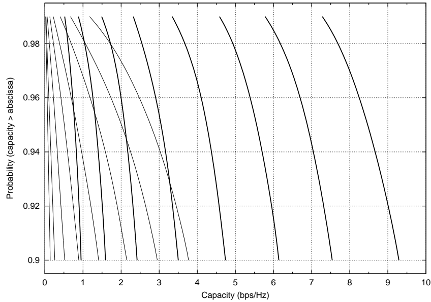
Figure 2.7: Complementary Cumulative Distribution Function of the capacity for n_T = 1 and n_R = 1 (thin lines) and n_T = 2 and n_R = 2 (bold lines). The SNR varies between 0 and 21 dB in increments of 3 dB. Each line represents a different SNR.
