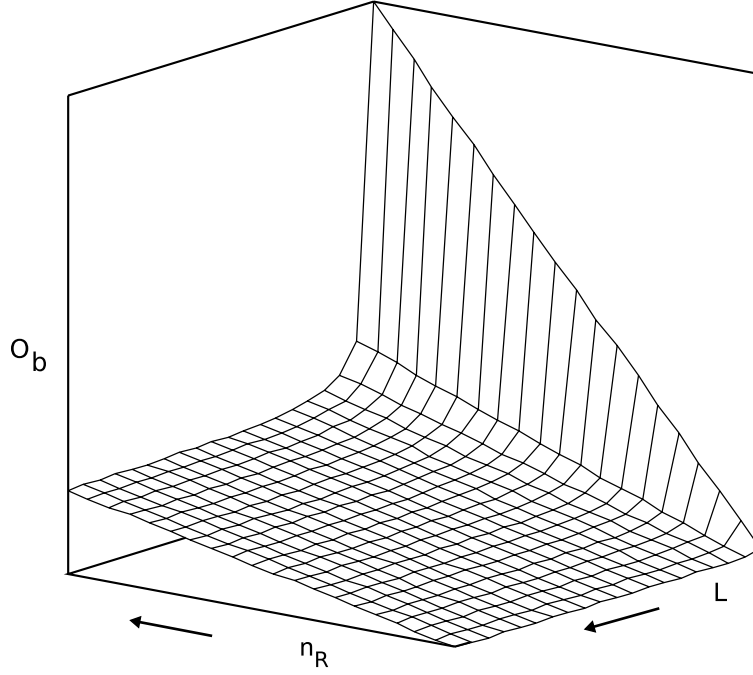
Figure 4.5: Behavior of O_b in V-BLAST as a function of n_R and L . The arrows indicate the direction of growth of n_R and L .
