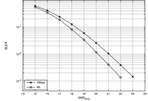
Fig. 1 Comparison between V-BLAST and a lattice-decoder algorithm.
