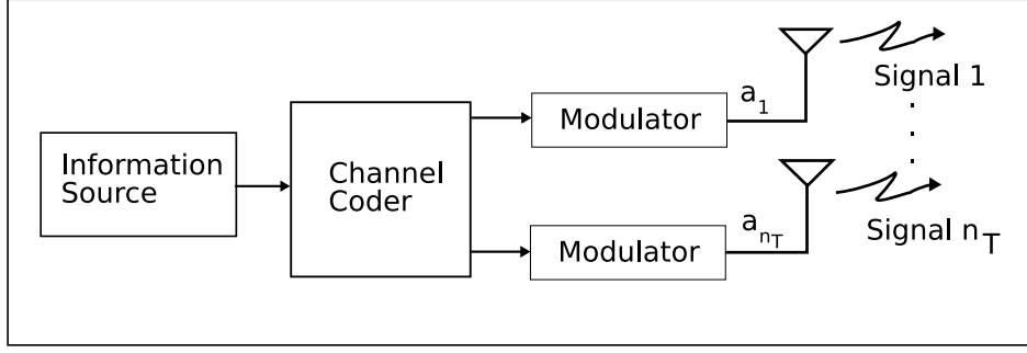
Figure 2.2: Baseband block diagram of a MIMO system.
