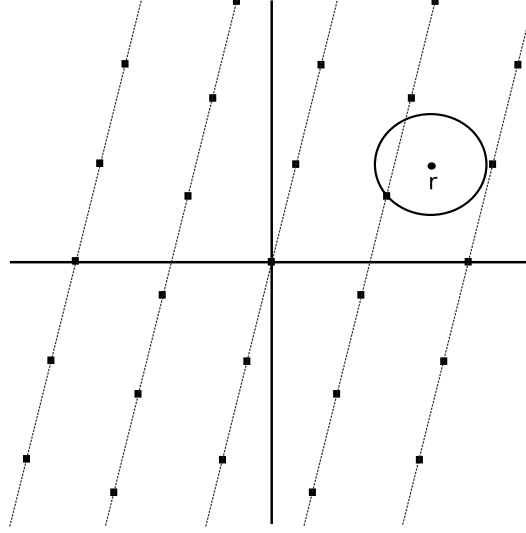
Figure 6.1: A lattice in two dimensions. The solid points represent the lattice points. The straight lines emphasize the periodic arrangement of the points. Also shown is a point \mathbf{r} \in \mathbb{R}^2 , and the closest lattice point.
