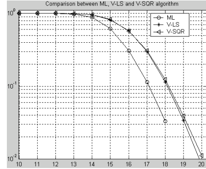
Figure 8: BLER vs SNR_{avg} M = 8 ; N = 12 .
