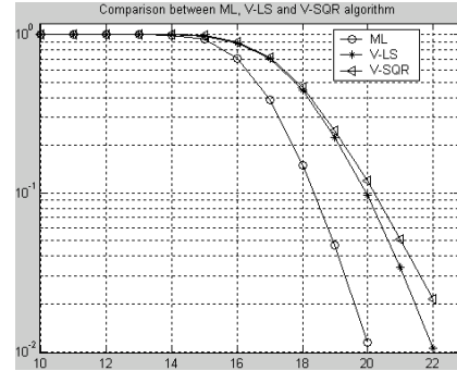
Figure 7: BLER vs SNR_{avg} M = 8 ; N = 10 .
