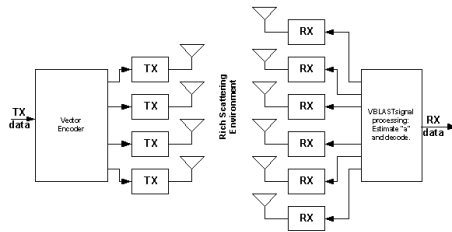
Figure 1: VBLAST architecture.
