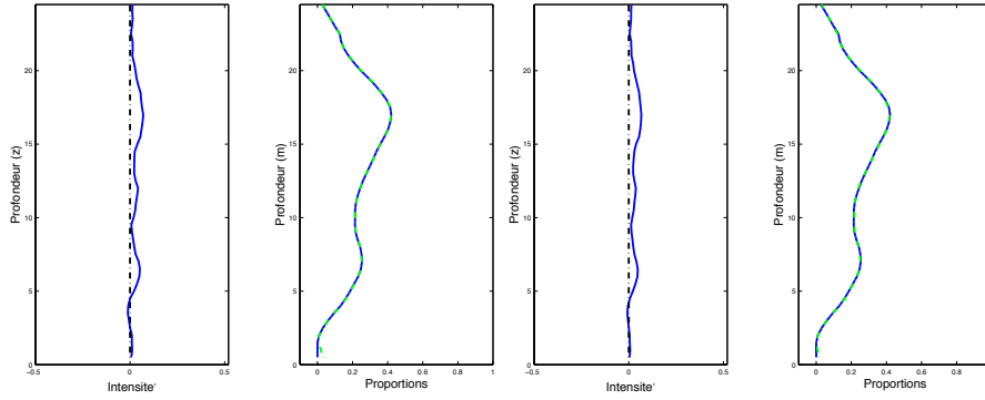
(c) \Gamma = 0.01
