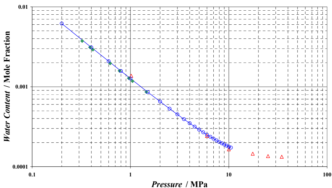
Figure 6.14: Comparison: Water Content in the Vapour Phase of the Water –Methane (○, Water content in Methane), -Ethane (◆, Water content in Ethane) and -MIX1 (△, Water content in MIX1) Systems at 283.1 K
