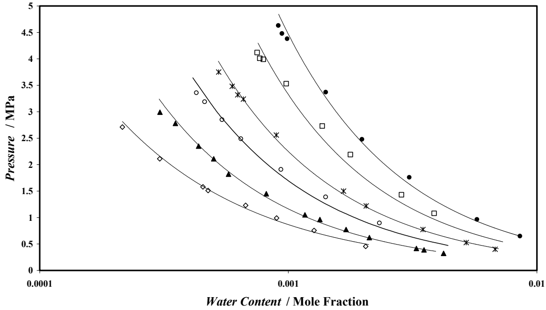
Figure 6.7: Water content in the vapour phase of the ethane - water system \diamond , 278.08 K; \blacktriangle , 283.11 K; \circ , 288.11 K; * , 293.11 K; \square , 298.11 K; \bullet , 303.11 K.
