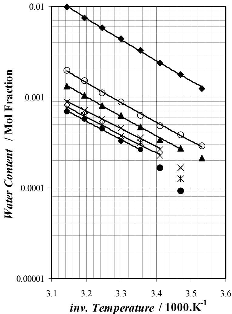
Figure 6.2b: Water content in the gas phase of the water – methane system
