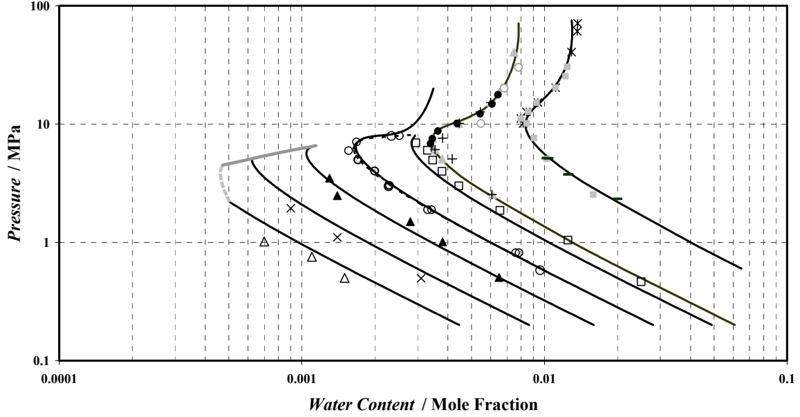
Figure 6.8: Water content in the vapour phase of the carbon dioxide - water system \square , 318.2 K; \circ , 308.2 K; \blacktriangle , 298.2 K; \times , 288.2 K; \triangle , 278.2 K; Literature data: + , 323.15 K from [44]; \blacktriangle , 323.15 K from [45]; \bullet , 323.15 K from [39]; \circ , 323.15 K from [37]; \blacksquare , 348.15 K from [44]; \star , 348.15 K from [45]; — , 348.15 K from [27]; Solid lines, calculated with the PR-EoS and Classical mixing rules with parameters from Table 6.4 at 278.22, 288.26, 298.28, 308.21, 318.22, 323.15 and 348.15 K. Grey solid line, water content calculated at \text{CO}_2 vapour pressure with model 1. Grey dashed line, water content calculated at \text{CO}_2 hydrate dissociation pressure
