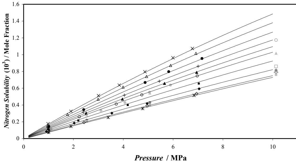
Figure 6.23: Nitrogen mole fraction in water rich phase as a function of pressure at various temperatures. New solubility data: \times , 274.2 K; \triangle , 278.2 K; \bullet , 283.1 K; + , 288.1 K; \blacktriangle , 293.1 K; \circ , 298.1 K; \blacksquare , 308.2 K; \blacklozenge , 323.1 K; \diamond , 343.0 K; * , 363.0 K; Literature data: \blacktriangle , 298.1 K from Wiebe et al. [119]; \bullet , 303.1 K from Smith et al. [123]; \bullet , 323.1 K from Wiebe et al. [119]; \blacksquare , 348.1 K from Wiebe et al. [119]; \circ , 273.1 K from Goodman and Krase [118]; \square , 298.1 K from Goodman and Krase [118]; \triangle , 324.6 K from O'Sullivan et al. [124]; \diamond , 338.1 K from Saddington and Krase [121]; Solid lines, calculated with the VPT-EoS and NDD mixing rules with parameters from Table E.1. [B12]
