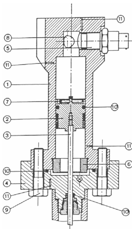
Figure 4.33: Equilibrium Cell
