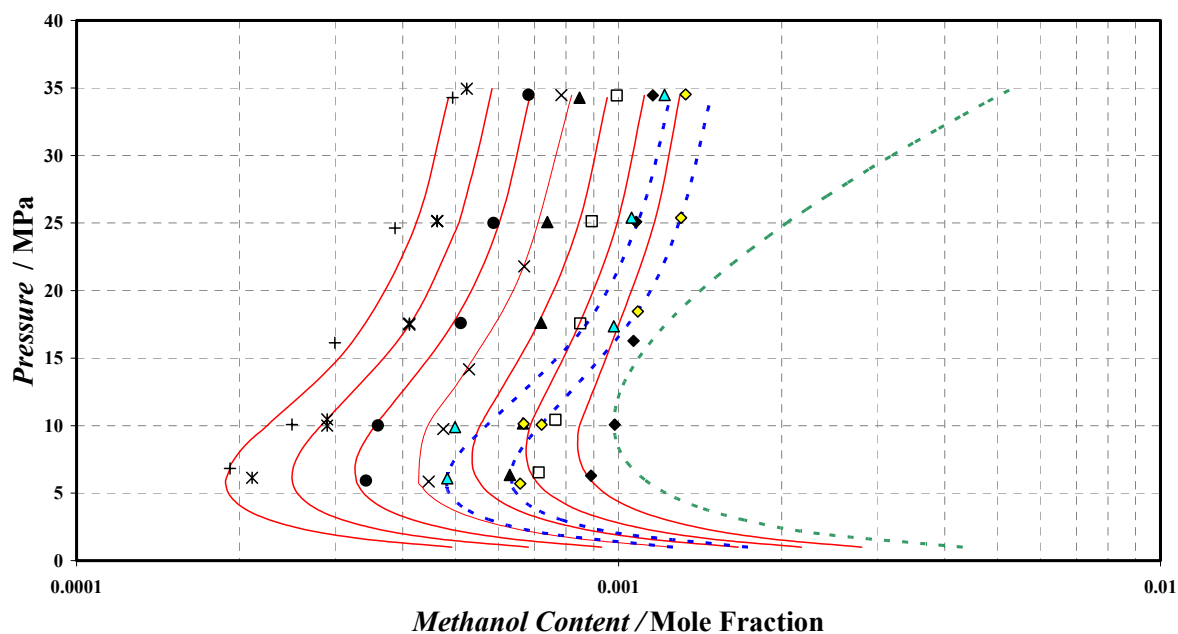
Figure 6.16b: Methanol content in the gas vapour phase of the MIX1- Water – X wt % Methanol system. X = 24: ◆, 298.1 K; □, 293.1 K; ▲, 288.1 K; ✕, 283.1 K; ●, 278.1 K; *, 273.1 K; +, 268.1 K; X = 49 : ○, 273.1* K; △, 268.1 K; Red solid line, \phi - \phi approach (HWHYD) at 24 wt. %; Blue dashed line, \phi - \phi approach (HWHYD) at 49 wt.%. Green dashed line, Methanol content in the vapour phase of the MIX1 – Methanol at 273.1 K (no water).
