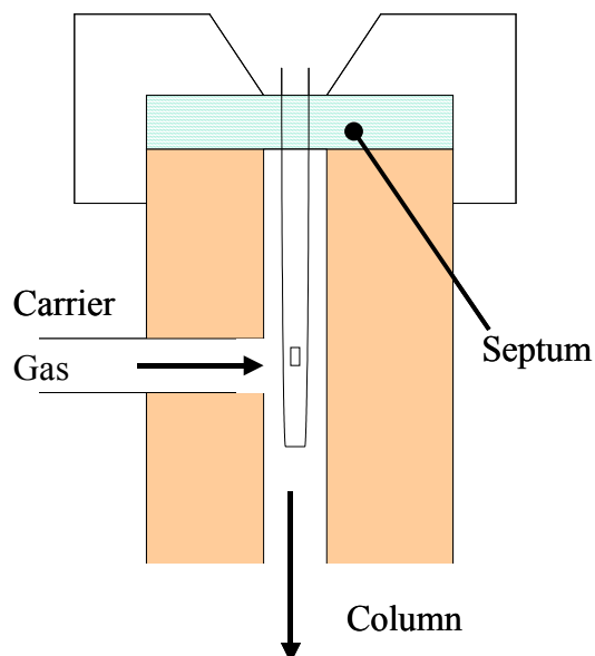
Figure 4.15: Simplified flow diagram of the injector
