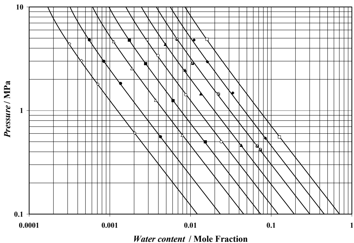
Figure 6.9: Water content in the vapour phase of the nitrogen - water system \diamond , 283.0 K; \bullet , 293.1 K; \triangle , 304.4 K; \blacksquare , 313.2 K; \circ , 323.0 K; \blacktriangle , 332.5 K; * , 342.3 K; \blacklozenge , 352.0 K; \square , 363.0 K. Solid lines, water content predicted at experimental temperatures with model 1.
