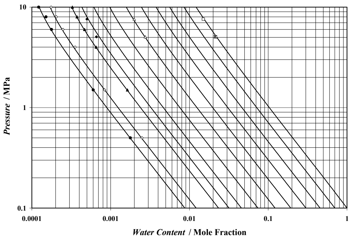
Figure 6.10: Water content in the vapour phase of the nitrogen - water system. \bullet , 278.15 K from Althaus [15]; \diamond , 283.15 K from Althaus [15]; \blacktriangle , 293.15 K from Althaus [15]; 298.15 K from Maslennikova et al. [47]; \triangle , 323.15 K from Maslennikova et al. [47]; \square , 373.15 K from Maslennikova et al. [47]; * , 373.15 K from Sidorov et al. [44]. Solid lines, water content calculated at 278.15, 283.15, 293.15, 298.15, 303.15, 313.15, 323.15, 333.15, 343.15, 353.15, 363.15 and 373.15 K with model 1.
