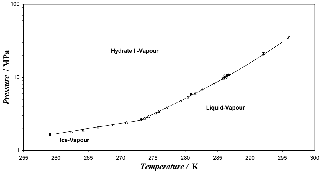
Figure 6.1: Pressure –Temperature diagram for methane and water
