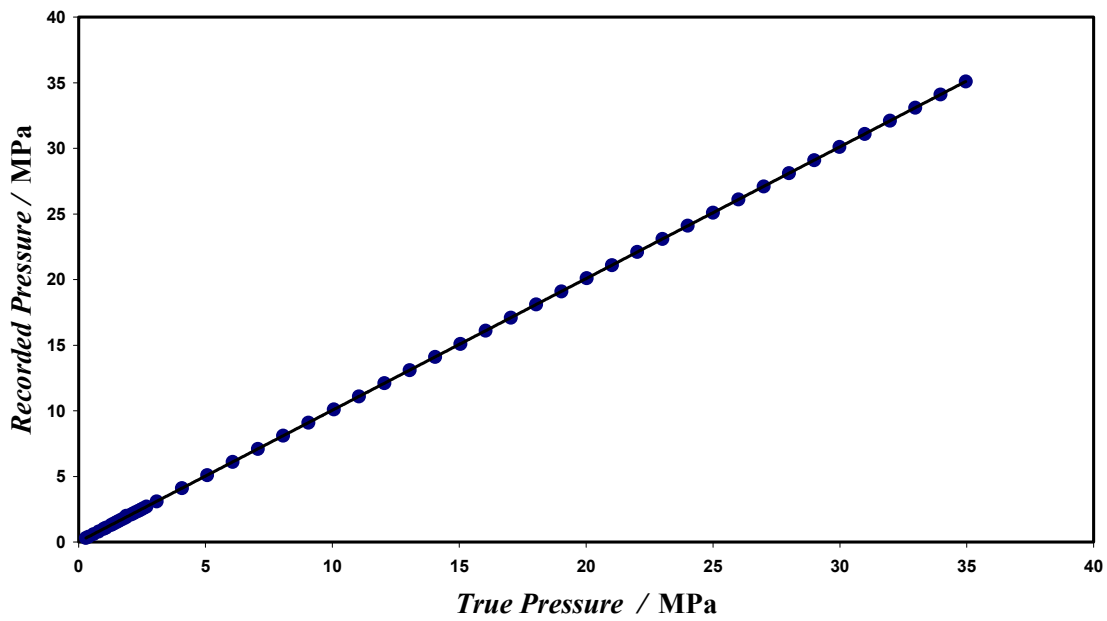
Figure 4.11: Pressure Transducer Calibration Curve 0-30 MPa
