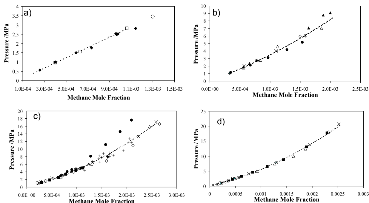
Figure 6.19: Comparison of Experimental Methane Solubilities in Water a) \square , 275.11 K; \circ , 274.15 K from [66]; \diamond , 274.29 K from [82]. b) \diamond , 283.13 K; \bullet , 283.15 K from [84]; \Delta , 283.2 K from [82]; * , 283.2 K from [86]; \blacktriangle , 285.65 K from [82]. c) \Delta , 298.15 K; \times , 298.15 K from [54]; \Delta , 298.15 K from [78]; + , 298.1 K from [83]; \bullet , 298.15 K from [68]; \diamond ; 298.2 K from [18]; \blacksquare , 298.15 K from [80]; \circ , 298.15 K from [81]; \blacklozenge , 298.15 K from [80]; \diamond , 298.15 K [87]; d) \circ , 313.11 K; \times , 310.93 K from [73]; \blacksquare , 310.93 K from [78]; \Delta , 313.2 K from [79]; Dashed lines, calculated with the VPT-EoS and NDD mixing rules with parameters from Table E.1 (Annex E).
