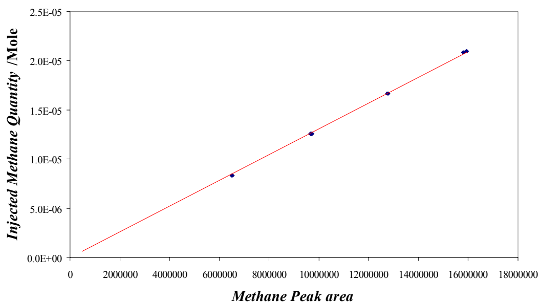
Figure 4.16: FID / methane calibration curve
