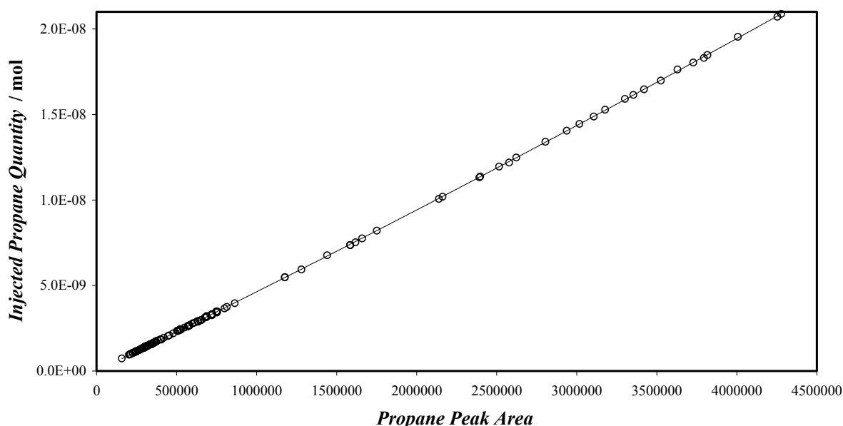
Figure 4.30: FID/Propane Calibration Curve. (peak area are in \mu V^2 )
