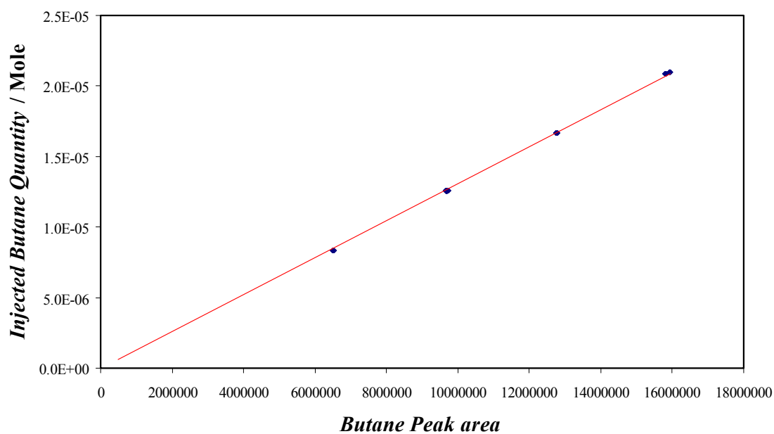
Figure 4.18: FID / n-butane calibration curve
