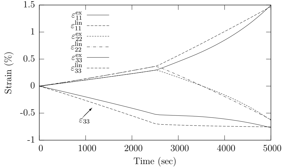
Figure 4.4: Comparison between some components of the strain history of the exact and approximate secant materials when subjected to the same non radial stress history. On the figure, exponent “ex” refers to the exact secant material and exponent “lin” refers to the approximate linearised material.
