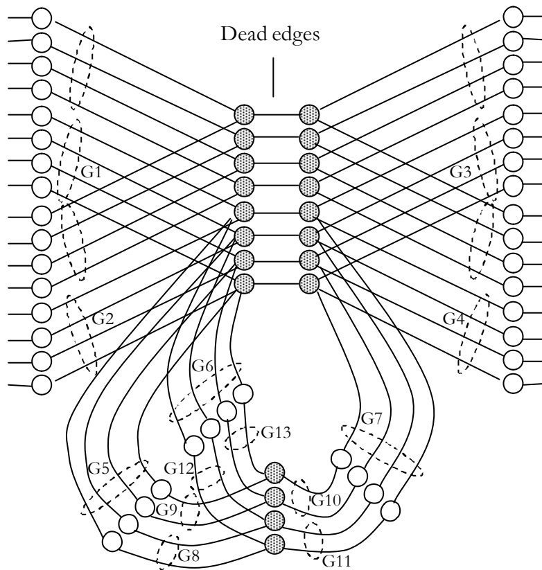
Figure 16: HXC graph model with dead edges to avoid negative costs.
