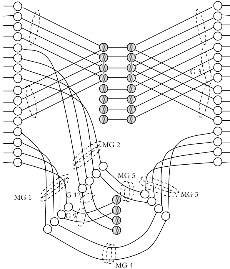
Figure 18: Example showing the wavelength switching operation in the MGGM.
