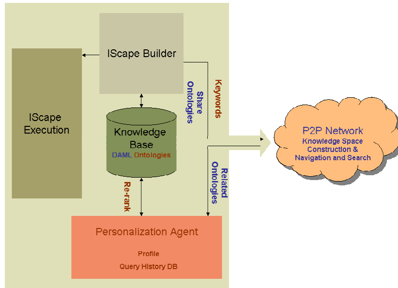
Figure 2.4 : Architecture d'un pair InfoQuilt [Arumugam et al. , 2002]
