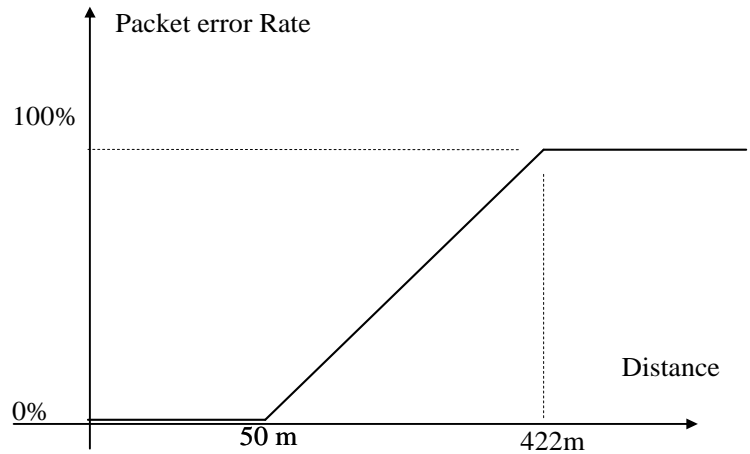
Figure V-4 IEEE802.11 propagation model in Gemini2
