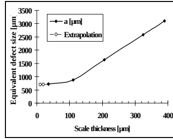
Figure II-41: Scale thickness influence on equivalent defects of size \bar{a} . Extrapolation to thin scales.
