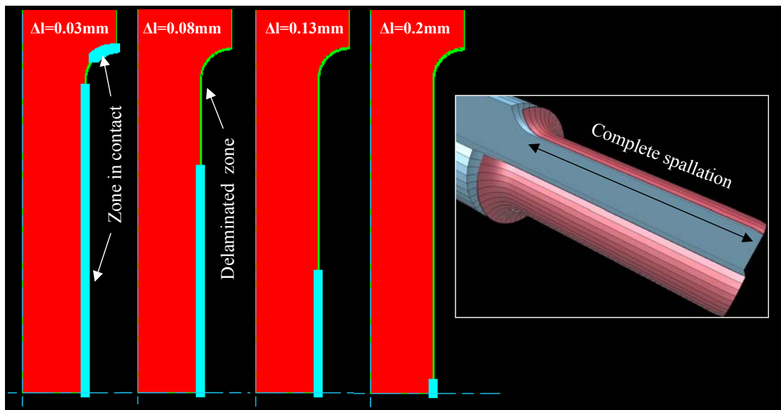
Figure V-22: Simulation of hot tensile test deformed at high temperature ( T=1000^\circ\text{C} ). Evolution of delamination process.
