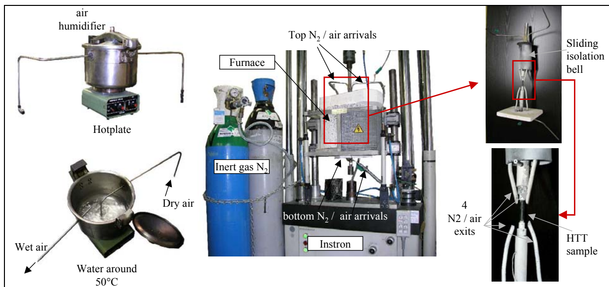
Figure V-9: HTT experimental device.
