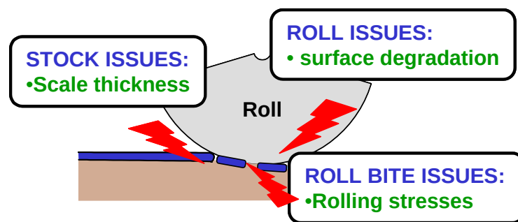
Figure V-1: Schematic representation of the complex interaction involved in rolled-in scale.
