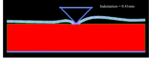
Figure III-21: Descaling; Strong coupling: \sigma_{nc} decreases by 40% of its original value \sigma_{nc0} .
