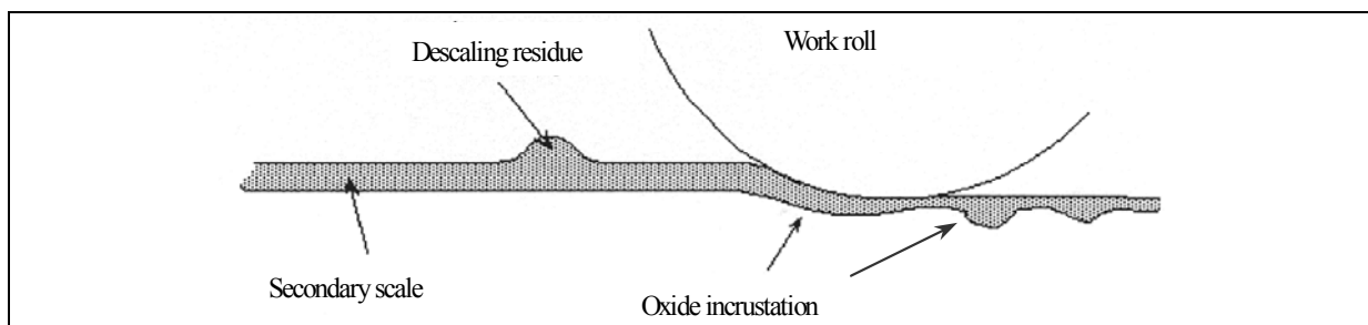
Figure I-35: Embedding of descaling residues in a FM stand.
