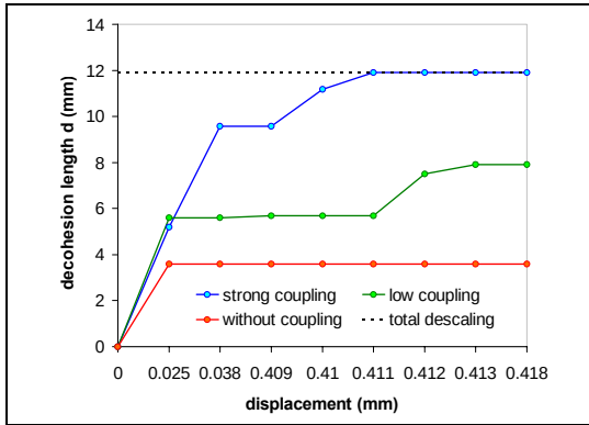
Figure III- 22: Influence of coupling on interface decohesion.
