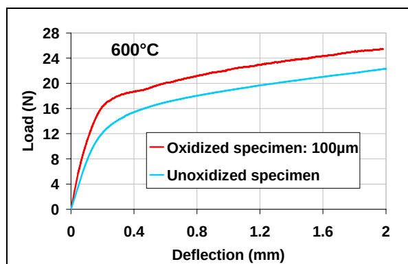
Figure IV-27: Example of curves obtained during unoxidized and oxidized tests at 600°C.
