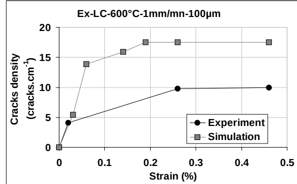
Figure IV-86: Crack density obtained experimentally and numerically using the developed damage model.
