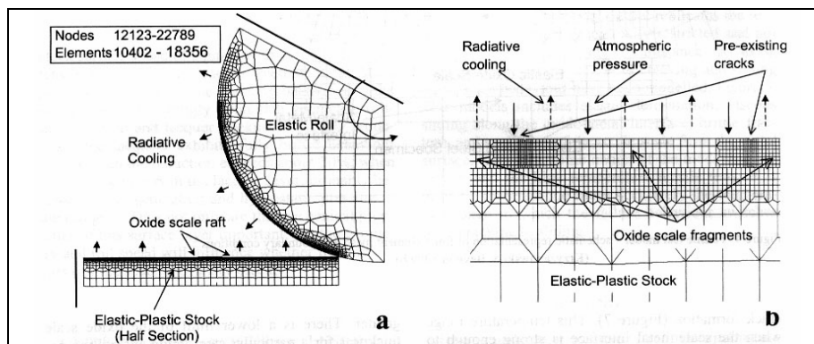
Figure VI-1: Macro and micro views of hot flat rolling model. Schematic view of FE mesh [Krz1].
