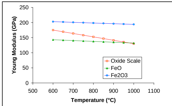
Figure II-29: Temperature dependence of iron oxides Young modulus [Sch1].
