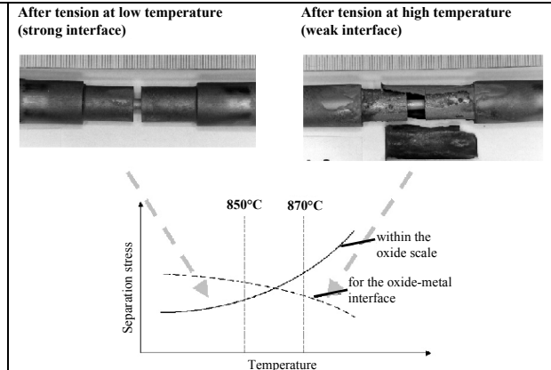
Figure V-3: Two different modes of oxide failure in tension during measurement of separation loads [Krz1,Krz2,Krz4].
