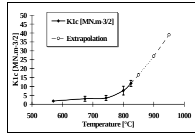
Figure II-42: Temperature influence on the toughness. Extrapolation to higher temperatures.
