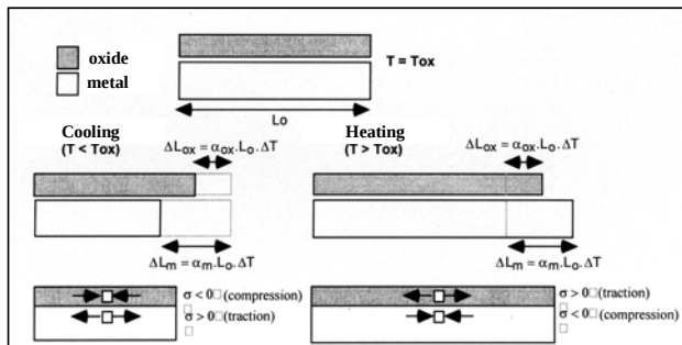
Figure II-39: Kind of stress obtained by differential dilatation.
