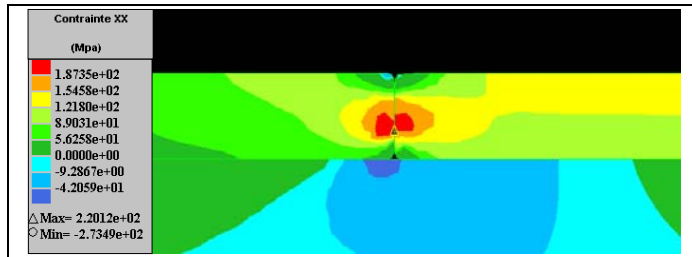
b) Critical-cracking stress reached in a node of the interface of two scale pieces.
