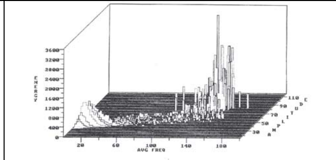
Figure IV-13: Analysis of the AE signals of the oxide scale on TiAl after oxidation and deformation at 900°C with respect to cumulative energy, average frequency and signal amplitude. Pre-oxidation time: 25 hours.
