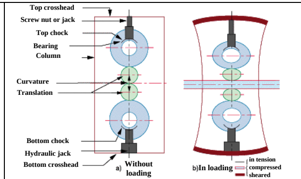
Figure I-6: 4 high stand elastic deformation [Ber].
