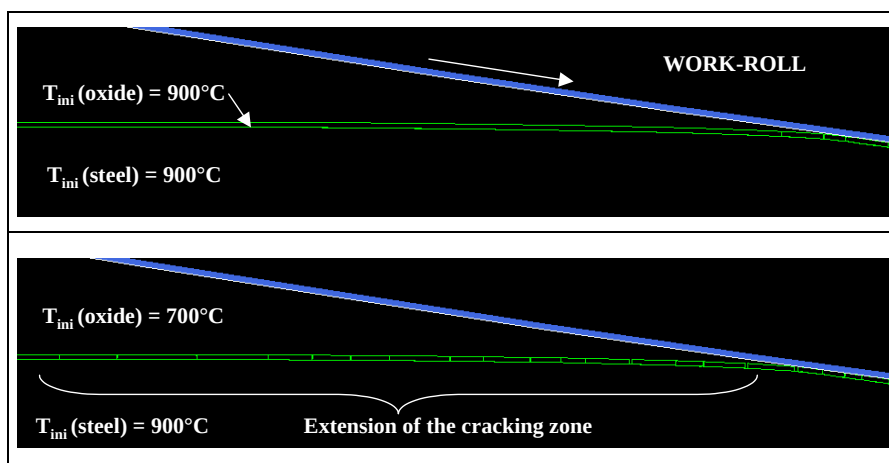
Figure VI-21: Strip cross section at the entry of the roll bite. Oxide thickness: 50 µm; reduction 35%; roll / scale contact: \mu = 0.3 ; initial temperature of the oxide scale : 700°C and 900°C.
