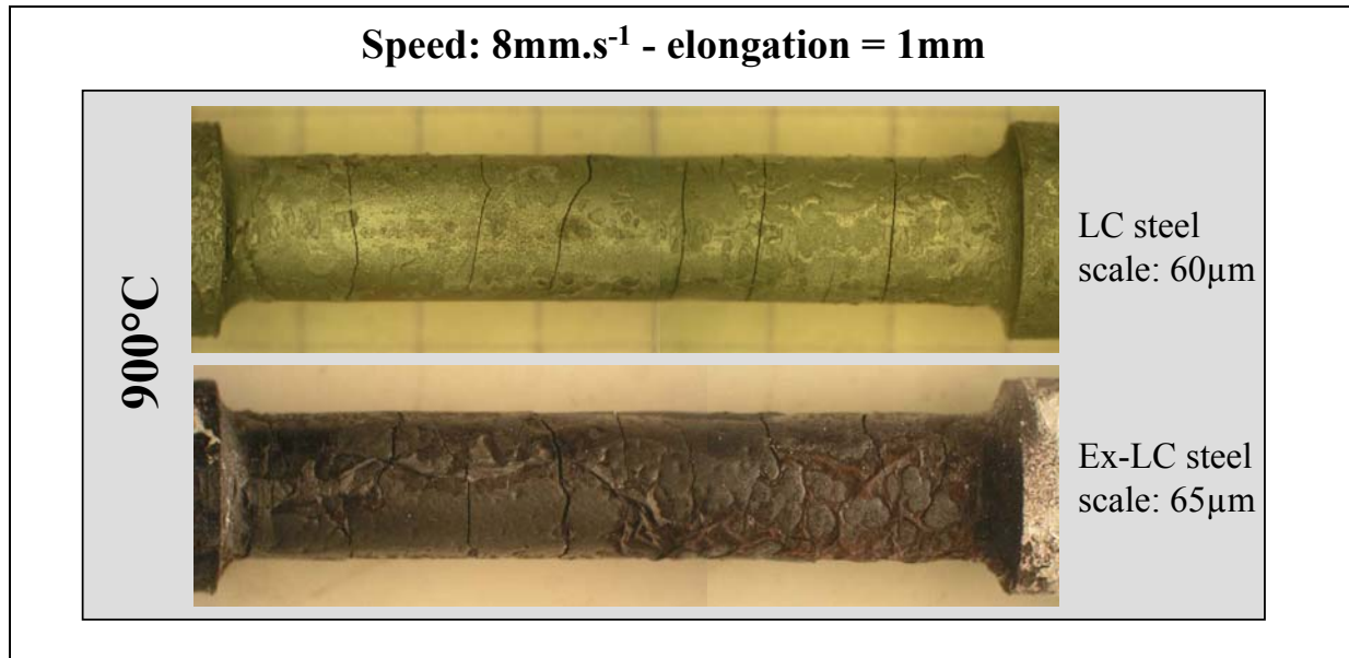
Figure V-16: Comparison between LC and Ex-LC steel grades deformed using HTT.
