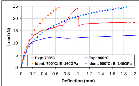
Figure IV-78: Superposition of experimental Ex-LC load-deflection curves (1mm/mn) and numerical curves obtained from purely elastic oxide scale behaviour.
