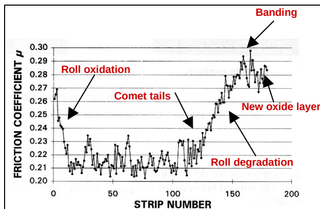
Figure I-26: Friction coefficient evolution in function of strip number and roll evolution. Stand F2. [Uijt2]
