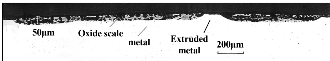
Figure V-31: Micrographic cross section of a deformed specimen after a PSCT. Steel grade: DDS, Temperature of deformation: 800°C, specimen reduction: 50%, velocity: 5 mm/s, initial scale thickness: 60 µm. Oxide scale reduction ~8%.
