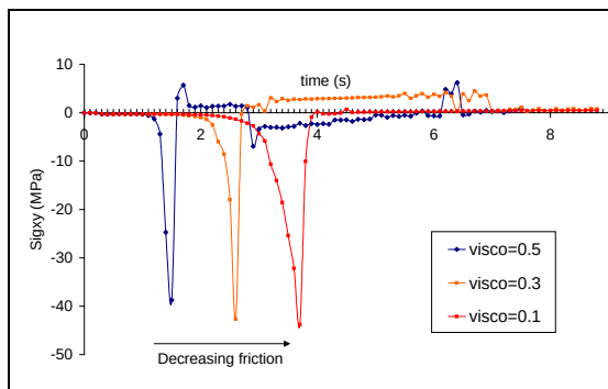
Figure III-14: Shear stress for node n°223.
