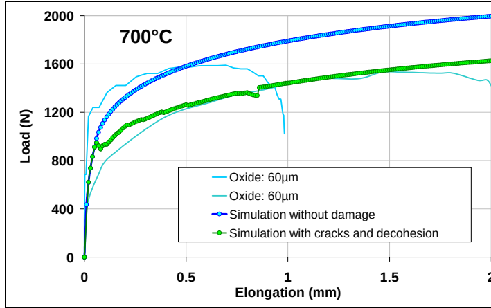
Figure V-21: Superposition of experimental and numerical load-elongation curves of HTT performed using oxidized specimens (oxide: 60 \mu\text{m} ) at 700°C.
