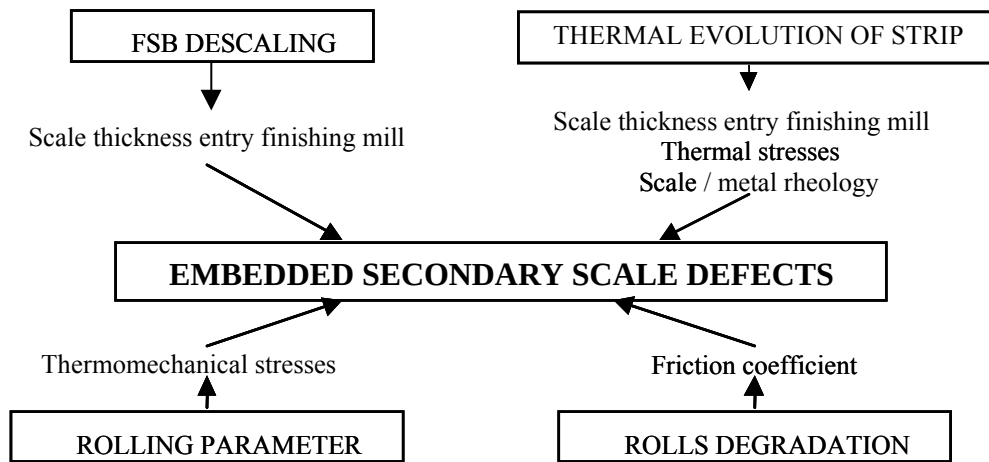
Figure I-41: Factors intervening in the rolled-in scale defect initiation.
