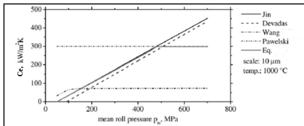
Figure I-21: Relationship between IHTC and mean roll pressure. [Zhou]
