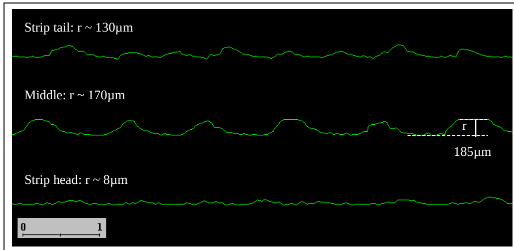
Figure VI-20: Interface roughness due to scale parts embedding. Surface aspect after descaling. Initial scale : 200 µm thick; reduction 45%; roll / scale friction: \mu = 0.6 ; Strip initial temperature: 900°C.
