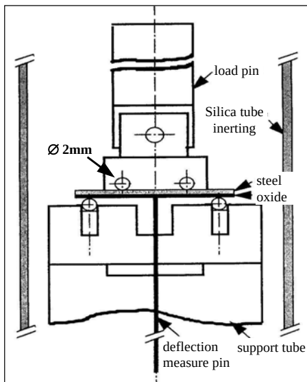
Figure IV-22: Schematic representation of the 4-point bending test device.
