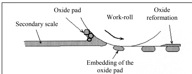
Figure I-40: « Pad » formation at the roll gap entry
