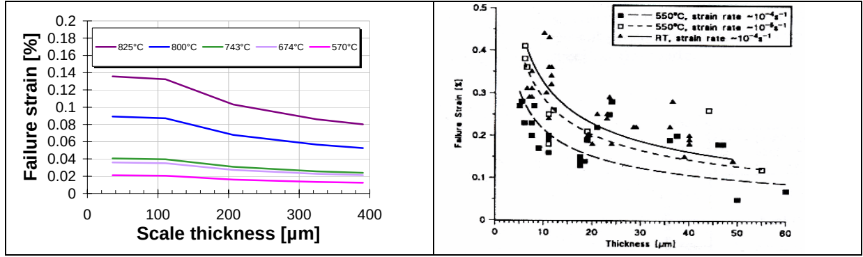
Figure II-44: Critical strain as a function of scale thickness. Left: [Han]; Right: [Nag1]
