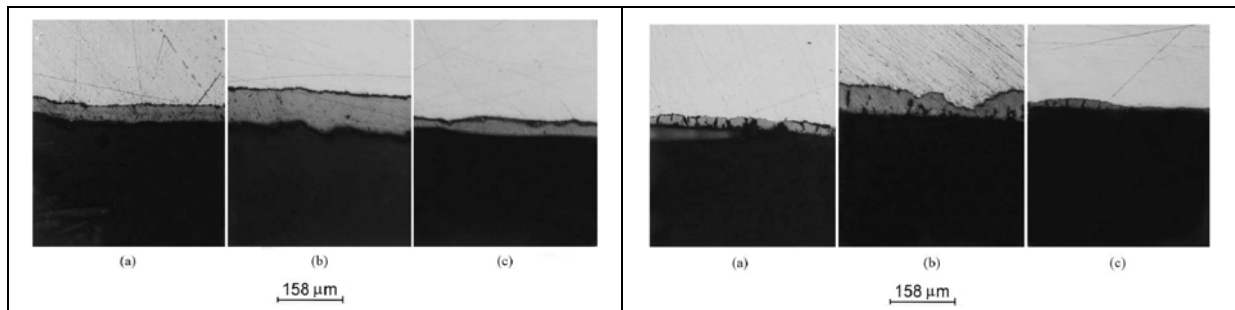
Figure I-58: 1) Thickness of the scale before the entry of the roll gap. Oxidation around 1100°C.
