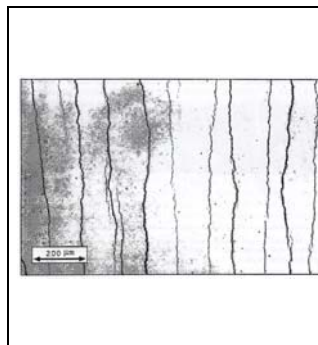
Figure IV-10: SEM image (BSE) of through-scale cracks in the oxide scale on Nickel substrate. Same test as Figure IV-9. Strain is 1.6% in the specimen center.
