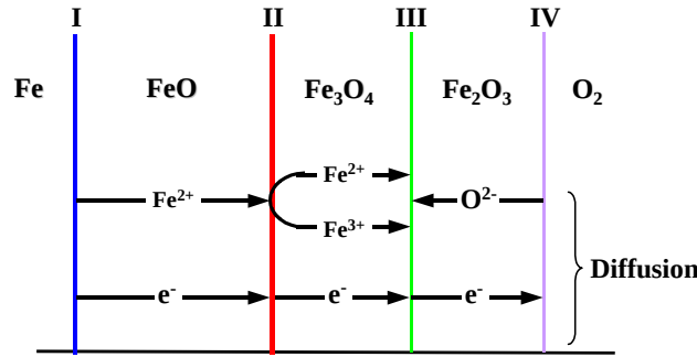
Figure II-6: Diffusion mechanisms of iron oxidation at T > 570^\circ\text{C} .
