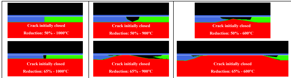
Figure V-38: Influence of bimaterial temperature and reduction on steel extrusion. Initial scale thickness 100 \mu\text{m} – V=50 mm/s.
