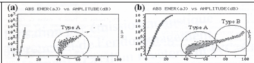
Figure IV-17: Absolute energy of events ( 1 \text{ aJ} = 10^{-18} \text{ J} ) vs. amplitude (dB) for two levels (a and b) of load. The associated load curve is plotted also (in arbitrary scale) [Dalm].
