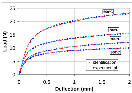
Figure IV-72: Ex-LC load-deflection curves. Superposition of experimental and numerical curves.
