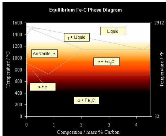
Figure I-10: Fe-C Phase diagram.
