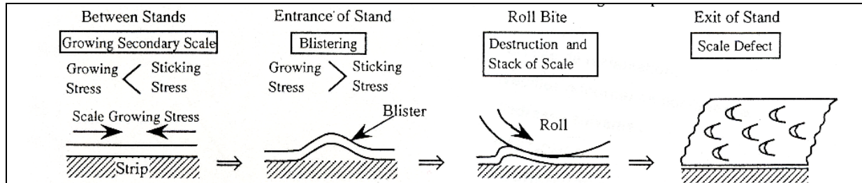
Figure I-37: Formation of secondary scale defect by oxide growth [Tom]
