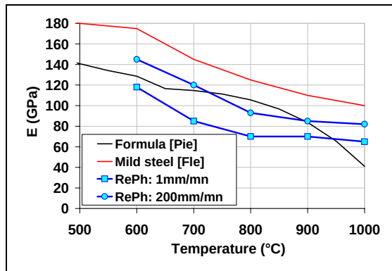
Figure IV-37: Strain rate influence.
