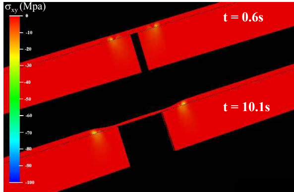
Figure III-16: shear stress field at two different time steps and for \tau_c=150\text{MPa} and \eta=0.1
