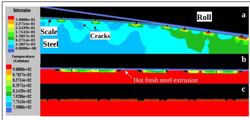
Figure VI-17: Fracture of the oxide layer before the roll bite and subsequent micro-extrusion.
