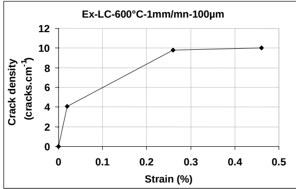
Figure IV-56: Crack density in the oxide scale as a function of strain for Ex-LC samples schematically represented in Figure IV-48.
