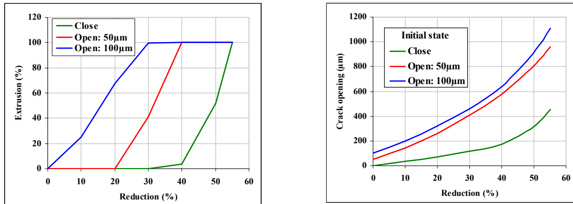
Figure V-37: Compression test: 800°C - V_{comp}=50 mm/s. Extrusion and crack opening vs total reduction. (No extrusion: 0% - Total extrusion: 100%).
