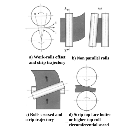
Figure I-8: Possible incidents [Mon1].
