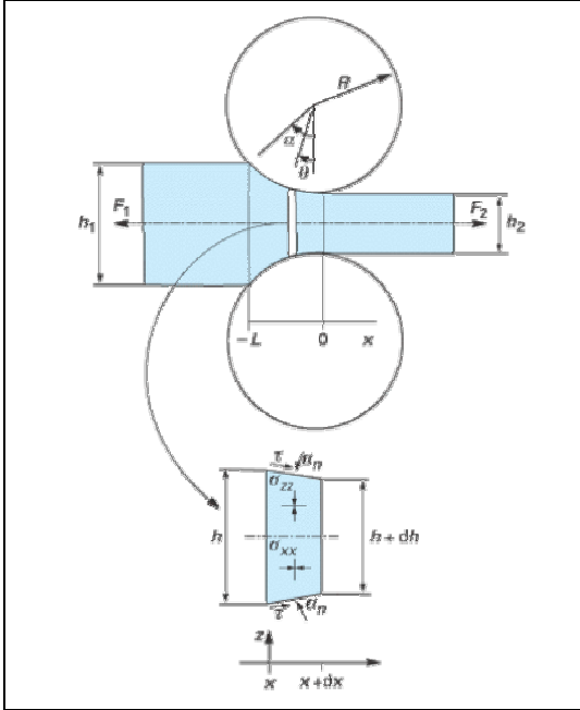
Figure I-13: Slab method: Roll gap divided in verticals slabs of infinitesimal width dx.
