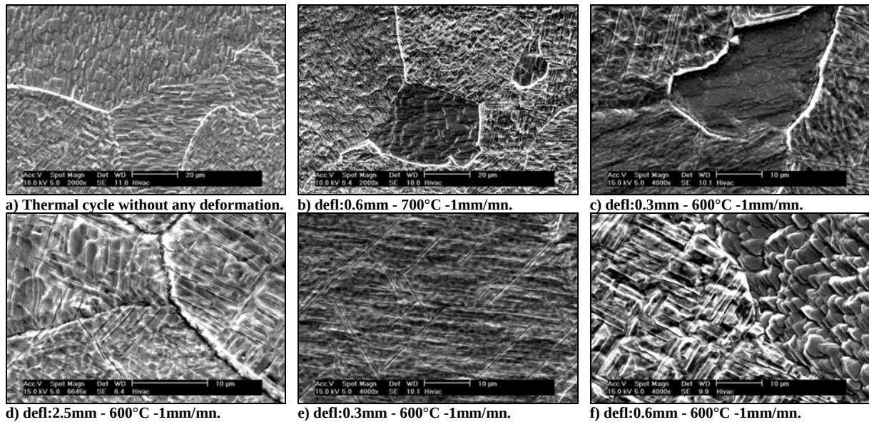
Figure IV-44: Ex-LC steel specimens: SEM micrographs of the oxide scale surface aspect. Oxide:100µm Eprouvette d'ExDx: micrographies MEB d'aspects de surface de la calamine. Oxyde:100µm
