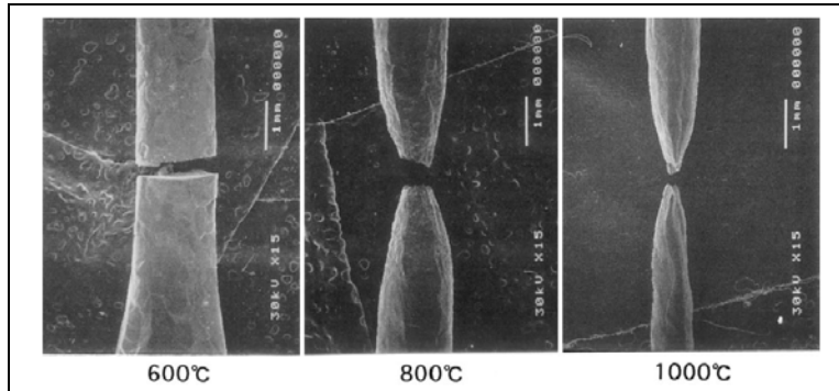
Figure II-30: Scanning electron micrographs (SEM) of FeO specimens after tensile tests at 2.10^{-4} \text{ s}^{-1} and at various temperatures.
