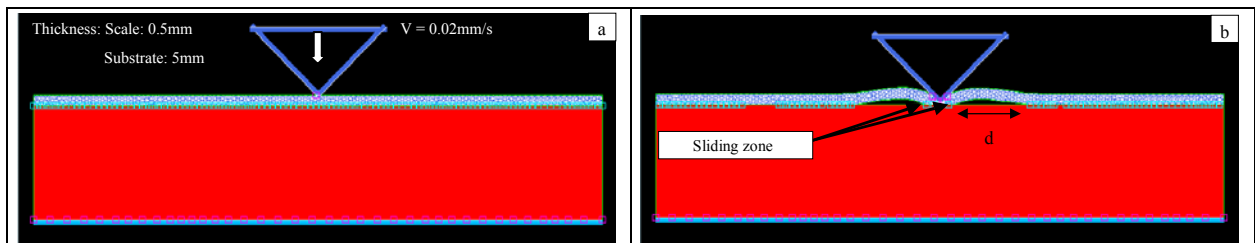
Figure III-19: Indentation simulation. a) Initial configuration: d=0\text{mm} b) d=3,28\text{mm} : decohesion
