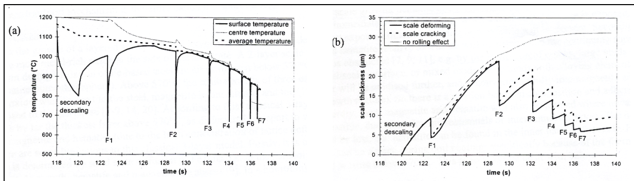
Figure I-16: a) Results of model calculations on the evolution of surface, center and average temperatures of a strip in a 7-stand finishing hot strip mill at the Corus Port Talbot works b) Calculated resulting scale growth on the same strip. [Li1]
