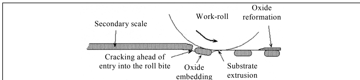
Figure I-38: Cracking at entry of roll gap followed by extrusion of steel. Tensile stresses at entry and exit. Compressive stresses under the rolls.
