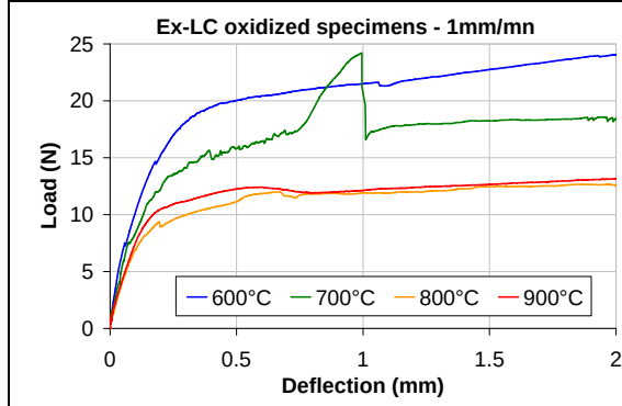
Figure IV-45: Load-deflection curves of oxidized Ex-LC steel. Oxide:100 \mu m – 1mm/min
