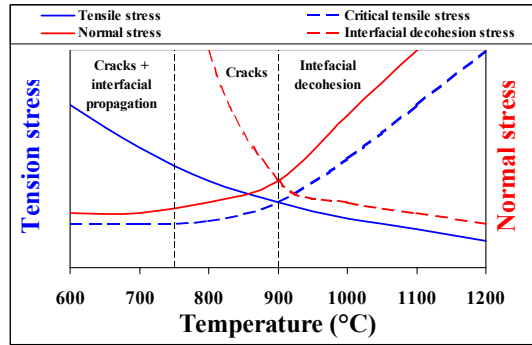
Figure V-11: Schematic representation of competition between damage processes depending on temperature. Interfacial propagation of cracks is not represented.
