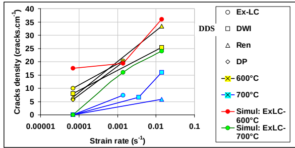
Figure IV-90: Crack density obtained experimentally and numerically.
