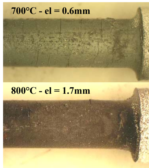
Figure V-14: HTT: samples deformed at 0.045 \text{ mm.min}^{-1} .
