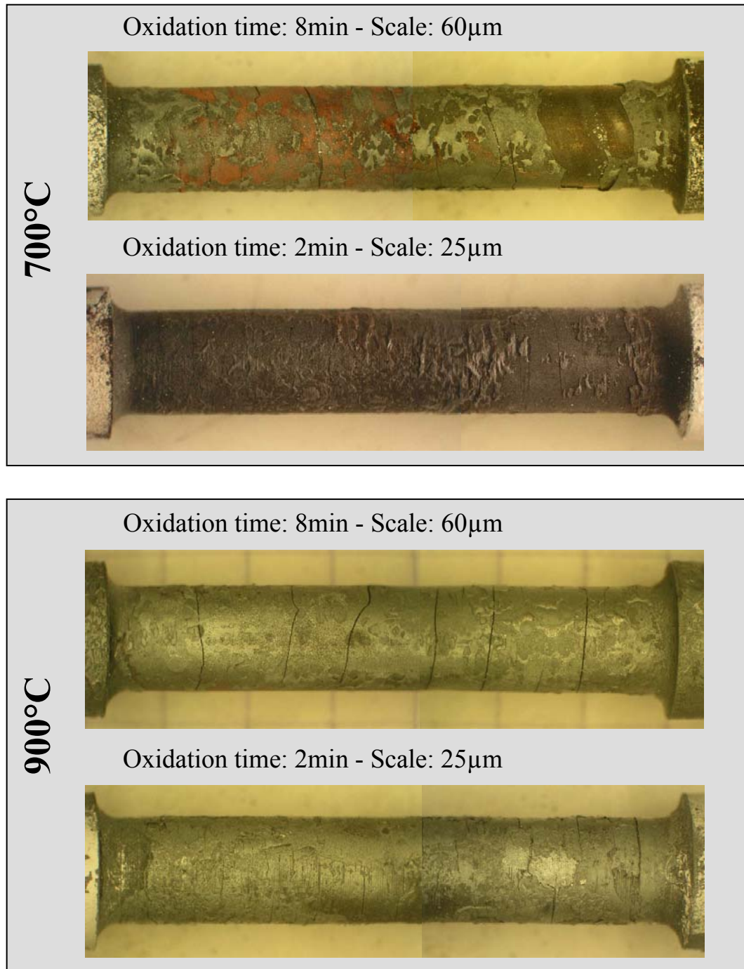
Figure V-15: Influence of scale thickness in HTT.
