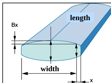
Figure I-7: Strip crown [Ber].
