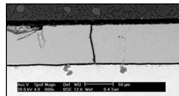
Figure IV-47: Micrograph of ReP specimen cross-section: defl: 3mm – 1mm/min – oxide: 70 \mu m – 1000°C.
