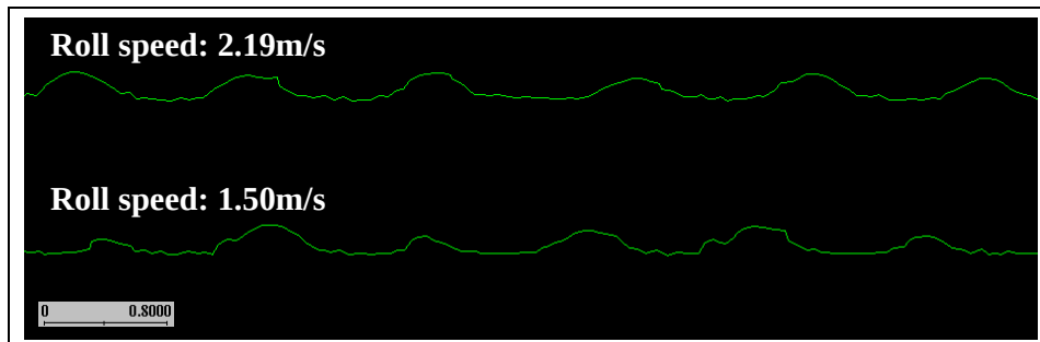
Figure VI-27: Speed influence. Surface roughness at the roll bite exit. Roll / scale friction: \mu = 0.3 ; reduction 45%; scale: 200 \mu\text{m} .
