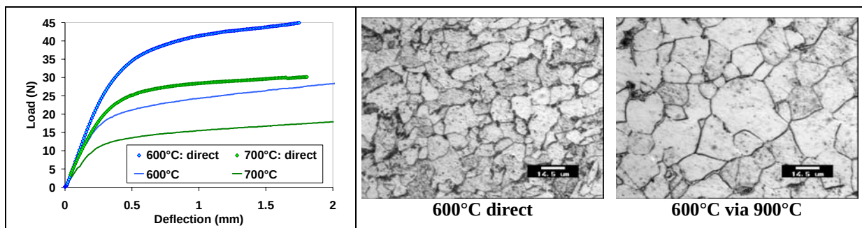
Figure IV-31: Thermal cycle influence on load-deflection curves.
