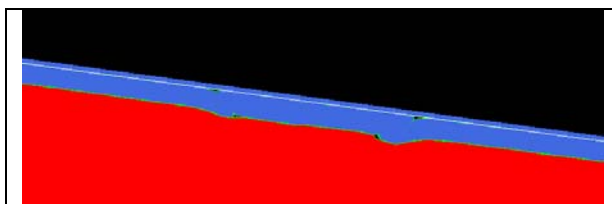
Figure VI-35: A negligible defect.
