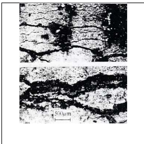
Figure I-47: Surface of steel slab after hot rolling. Photo above: scale thickness 210µm, reduction 18.9%. Below: scale thickness 240µm, reduction 38.7%.
