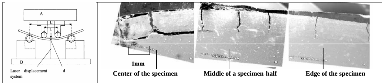
Figure IV-7: SEM cross section of functionally graded material specimens in four-point bending test [Zhou]
