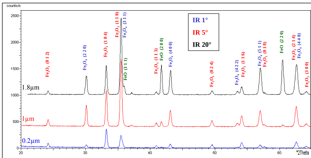
Figure II-16: XRD spectra superposition in grazing incidence. Angle between the beam and the oxide scale surface is 1^\circ , 5^\circ and 20^\circ .
