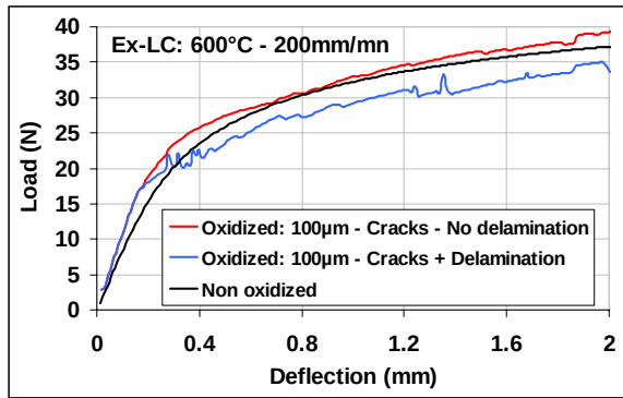
Figure IV-91: Specimen deformed at 200 mm/min and 600°C. Numerical load-deflection curves with and without decohesion.
