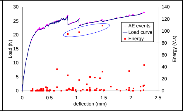
Figure IV-67: Test n°2. To each high energy event corresponds a load drop.
