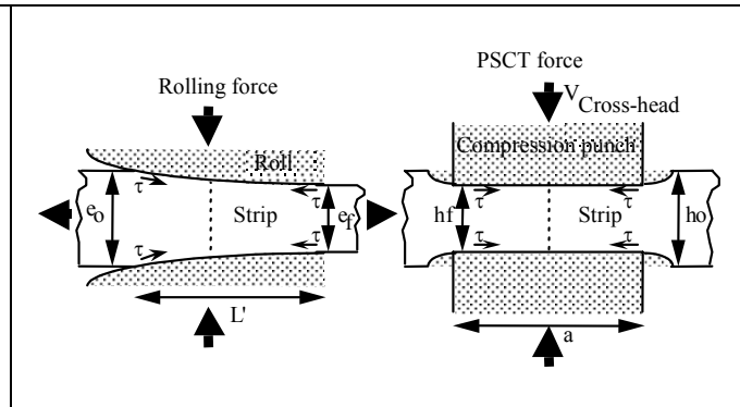
Figure V-25: Flow similarity in hot rolling and PSCT.
