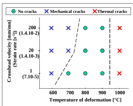
Figure IV-55: Schematic representation of oxide scale damage in 4-PHBT as a function of temperature and strain rate. Strain ~ 0.5%.
