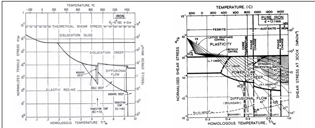
Figure IV-35: Iron deformation map [Ashby].
