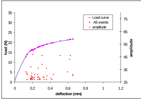
Figure IV-63: AE of test n°3 at 600°C – 1 mm/min – 100 μm – deflection = 0.7 mm
