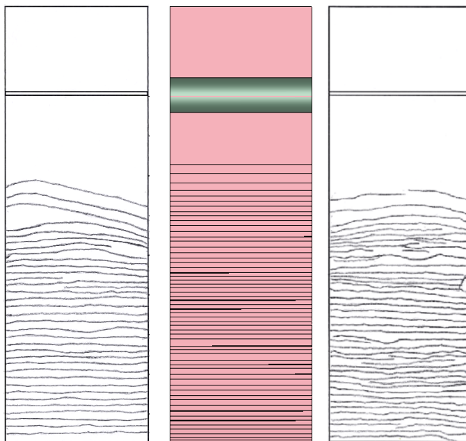
Figure IV-89: Sample deformed at 600°C and 200 mm/min. Middle: Ex-LC simulation. On either side: crack mapping for DDS (left) and ReN (right), already represented Figure IV-54
