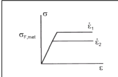
Figure IV-1: Ideal elastic-viscoplastic behavior [Echs].
