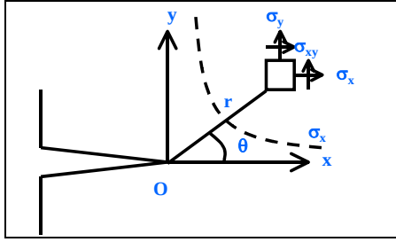
Figure II-35: Crack tip singularity.
