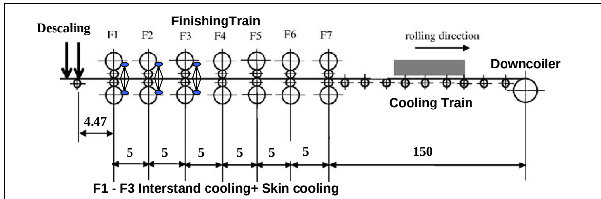
Figure I-4: Schematic view of a 7-stands finishing mill.
