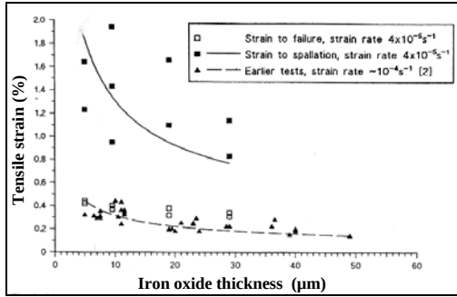
Figure II-48: Strain causing cracks and spallation vs. scale thickness. Tests at room temperature [Nag2].
