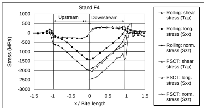
Figure V-27: Summary of stresses on surface, in rolling and PSCT. History of a material point.
