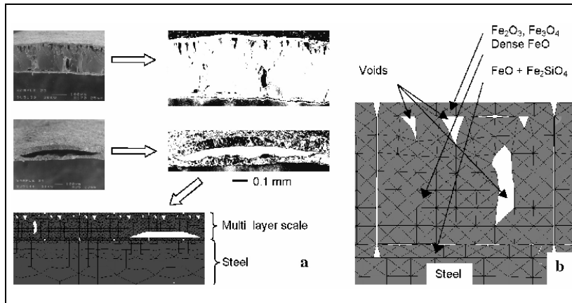
Figure V-7: Schematic representation of characteristic morphological features of the oxide scale into the FE model (a) and detailed FE mesh representing the three-layers oxide scale (b) [Krz2].
