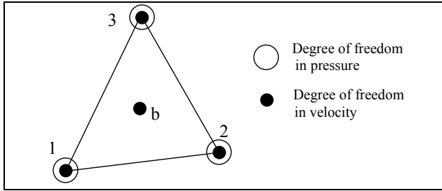
Figure III-5: P1^+/P1 triangular element.
