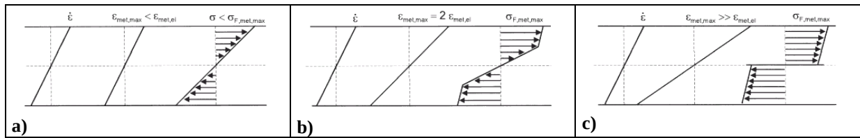
Figure IV-2: Stress-strain dependence during the 4-PBT [Echs].
