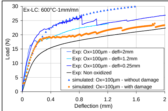
Figure IV-85: Ex-LC deformed using 4-PHBT: 600°C – 1 mm/min - oxide: 100 \mu\text{m} . Experimental and numerical load-deflection curves.
