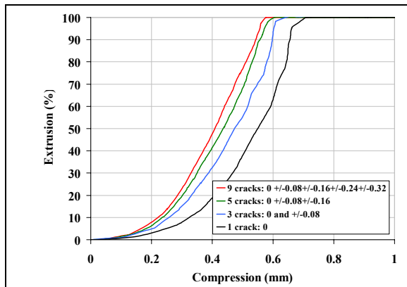
Figure V-46: Evolution of steel extrusion in PSCT as a function of crack number. Cracks of 40 µm width and distant of 80 µm.
