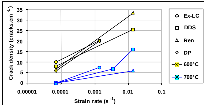
Figure IV-57: Evolution of several steel grades crack density versus strain rate at 600 and 700°C.
