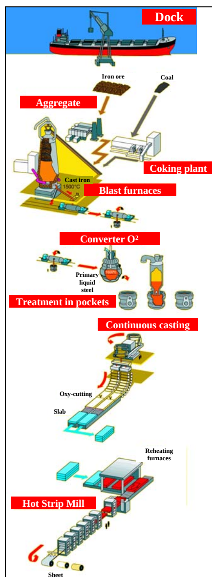
Figure I-1: Schematic representation of Fos sur Mer HSM.
