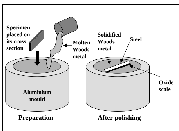
Figure II-13: Method described in [Hig1] for EBSD analysis.
