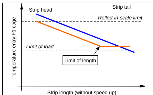
Figure II-20: Temperature at the FM entry.
