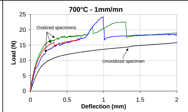
Figure IV-46: Several oxidized Ex-LC steel specimens deformed at 700°C. Oxide:100 \mu m – 1mm/min
