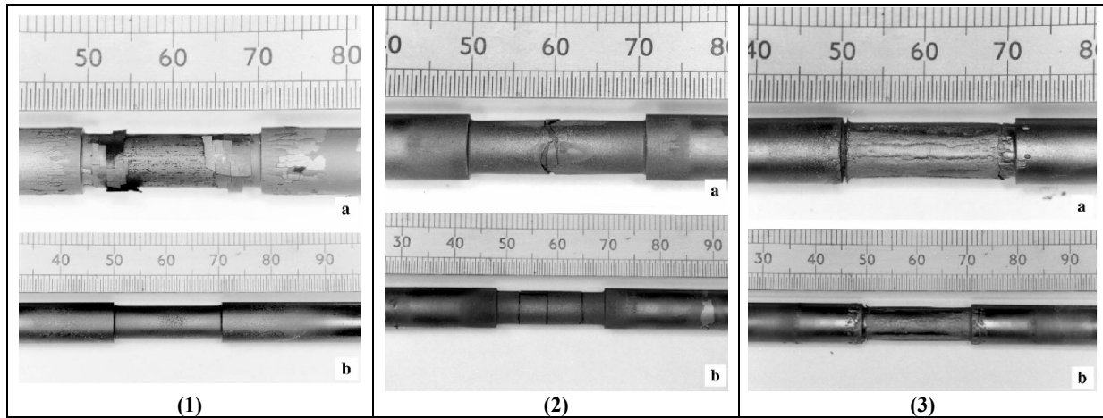
Figure V-4: Oxide scale on the tensile specimen after testing. (a) steel 1; (b) steel 2. (1) T=830^{\circ}\text{C} , \varepsilon=2\% , \dot{\varepsilon}=0.2\text{s}^{-1} . T_{\text{ox}}=830^{\circ}\text{C} , t_{\text{ox}}=800\text{s} (60 \mu\text{m} ). (2) T=975^{\circ}\text{C} , \varepsilon=5\% , \dot{\varepsilon}=2\text{s}^{-1} . T_{\text{ox}}=975^{\circ}\text{C} , t_{\text{ox}}=800\text{s} (178 \mu\text{m} ). (3) T=1150^{\circ}\text{C} , \varepsilon=5\% , \dot{\varepsilon}=4\text{s}^{-1} . T_{\text{ox}}=1150^{\circ}\text{C} , t_{\text{ox}}=100\text{s} (172 \mu\text{m} ) [Krz1, Krz3].
