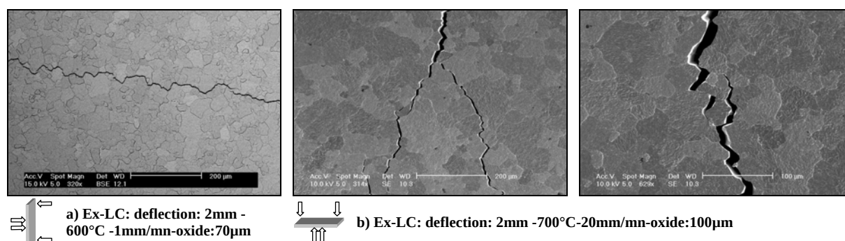
Figure IV-39: intergranular crack propagation.
