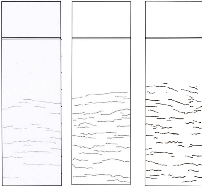
Figure IV-48: Ex-LC deformed using 4-PHBT: 600°C - 1mm/min - oxide: 100µm. Crack mapping of oxidized half-samples; From the left to the right : deflection = 0.25 mm, 1.2 mm, 2 mm.
