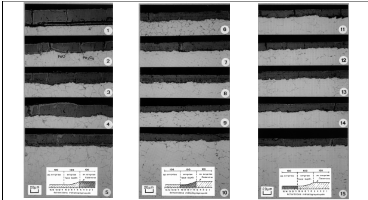
Figure I-42: Strip rolled in the Seremange roughing mill.
