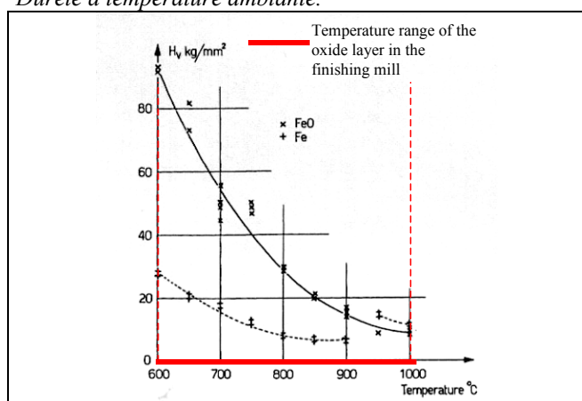
Figure II-28: FeO and Fe Vickers hardness vs. temperature
