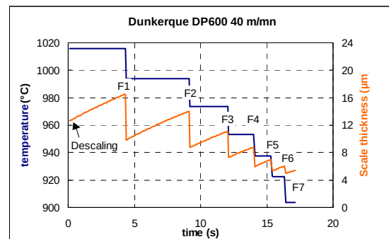
Figure II-23: DP 600 steel: Maximal scale thickness in stand F1.
