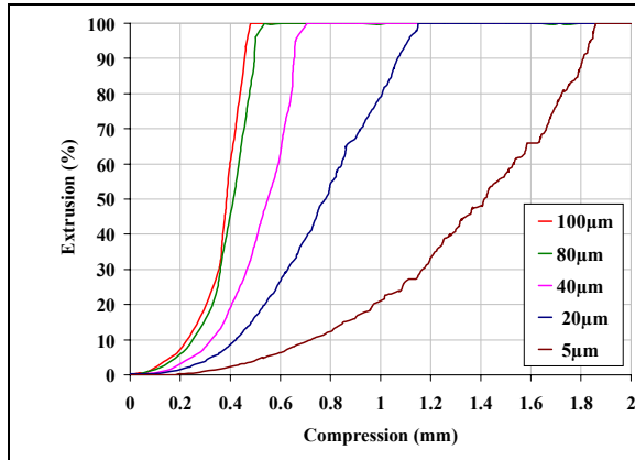
Figure V-44: Evolution of steel extrusion in PSCT as a function of cracks width.
