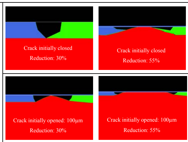
Figure V-36: Extrusion evolution depending on strain and crack initial state.
