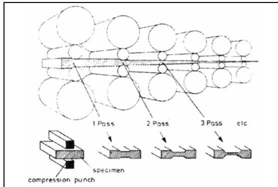
Figure V-24: Principle of HSM simulation using PSCT [Paw].
