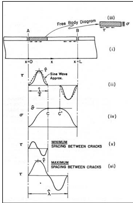
Figure II-45: Determination of critical crack spacing L_c . [Agr]
