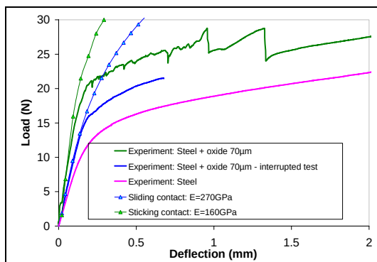
Figure IV-77: Young's modulus identification on experimental Ex-LC load-deflection curves (1mm/mn-600°C). Contact influence.
