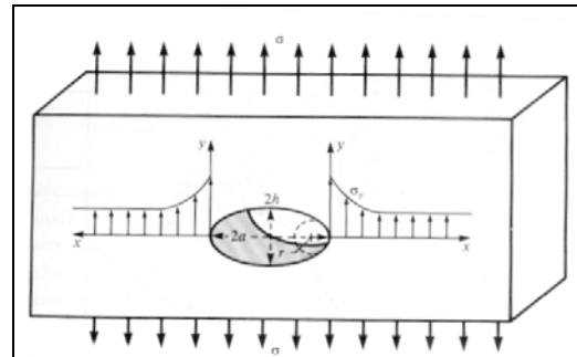
Figure II-34: Stress concentration zone for an initial ellipsoidal defect.
