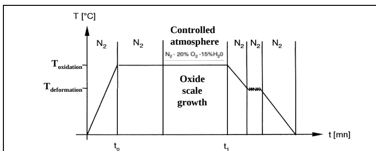
Figure II-11: Thermal cycle used for mechanical tests, mimicking those in the FM.
