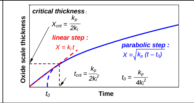
Figure II-8: Mathematical representation of the transition between the linear and the parabolic step.
