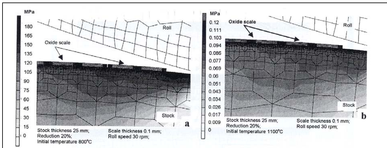
Figure VI-3: \sigma_x stress predicted at the moment of the entry into the roll gap. Initial temperature: a) 800°C b) 1100°C (no cracking) [Krz1,Krz4].
