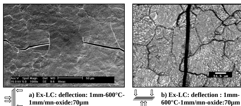
Figure IV-40: Transgranular cracks propagation.
