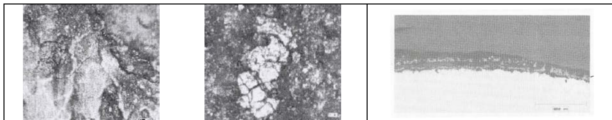
Figure I-55: Rolled-in scale defect. Left picture: commercial hot band. Right picture: Experimental hot band (same picture enlargement) [Til].
