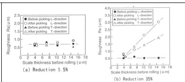
Figure I-54: Influence of scale thickness before rolling on the surface roughness [Oka].
