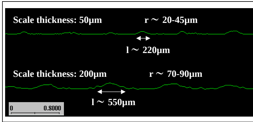
Figure VI-26: Scale thickness influence. Strip cross sections at the roll bite exit, in the middle of the stock length. Roll / scale contact: \mu = 0.3 ; reduction 35%.
