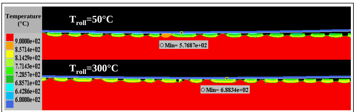
Figure VI-23: Influence of the work-roll average temperature. Strip cross section inside and at the exit of the roll bite. Initial scale thickness: 200 \mu\text{m} ; reduction 45%; roll / scale contact: \mu = 0.3 ; initial strip and scale temperature: 900°C.
