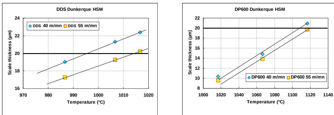
Figure II-21: A low maximal slab temperature to avoid rolled-in scale defect for DDS steel.
