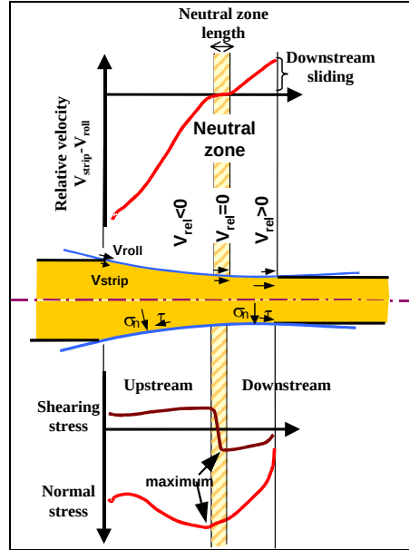
Figure I-9: Schematic representation of velocities and stresses in a stand.
