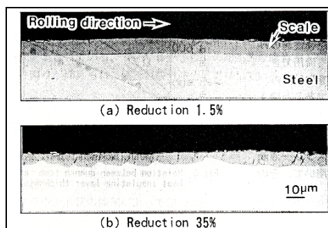
Figure I-53: Cross sectional images of scale/metal interface roughness depending on reduction [Oka].
