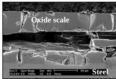
Figure IV-25: Preparation problem for cast extra low carbon steel specimen.
