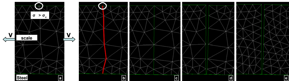
Figure III- 24: Successive steps for through thickness crack creation in Forge2®
