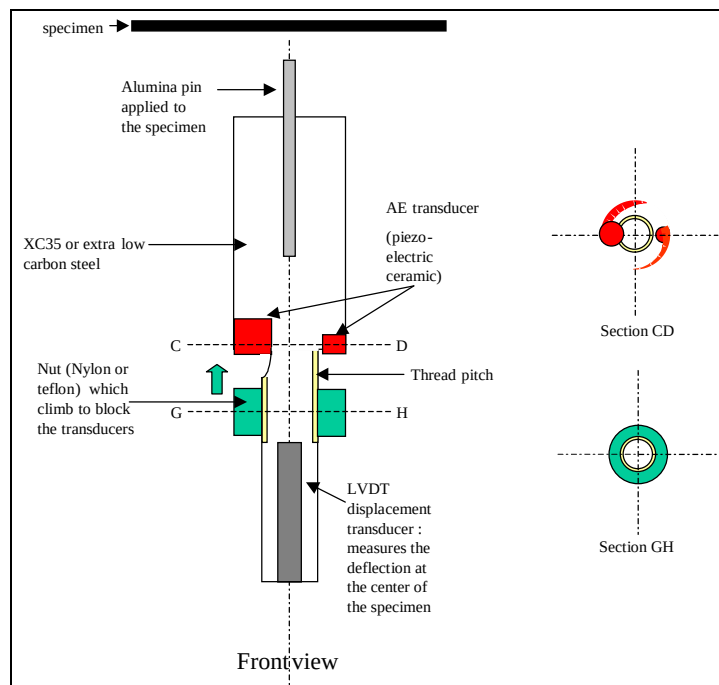
Figure IV-30: Device modifications to fix the AE transducers.
