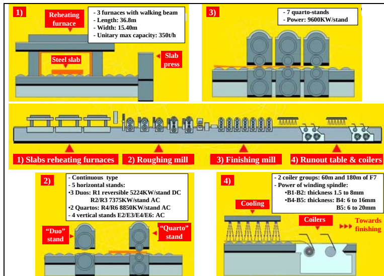
Figure I-2: General view of a HSM (Sollac – Fos sur mer) [Fos]
