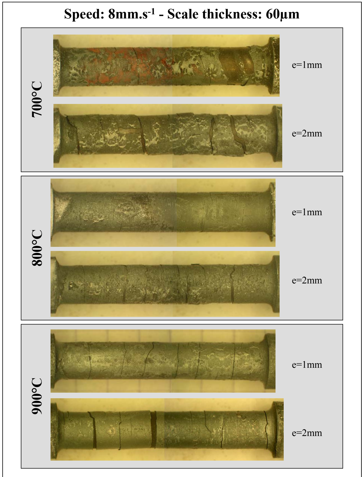
Figure V-12: Specimens covered by an oxide scale 60\mu\text{m} thick using HTT. Test speed: 8\text{mm.s}^{-1} .
