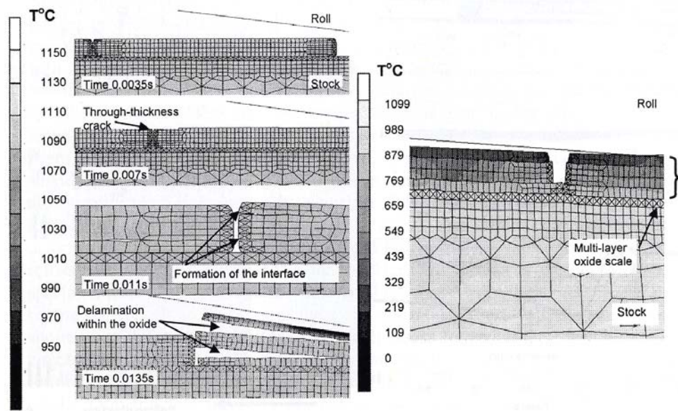
Figure VI-6: Left: Development of through-thickness cracks and delamination within the multi-layer Si-Mn steel oxide scale. Right: Adherence of the inner scale layer with uninterrupted shape [Krz4, Tan].
