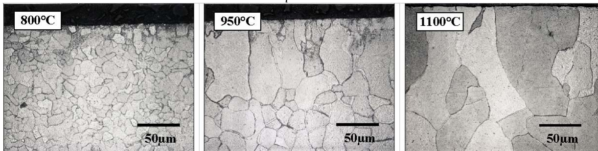
Figure IV-33: Optical micrographs of Ex-LC steel. Grain size difference depending on the high temperature dwell (idem for dwell time). Nital etching.
