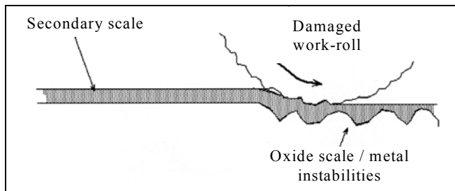
Figure I-39: Metal/scale interface instabilities
