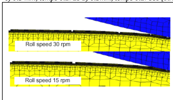
Figure VI-5: Different scale crack patterns formed at entry into the roll gap for the different roll speeds ; roll diameter 136.6 mm, reduction 20%, initial stock thickness 25 mm, temperature 800°C and oxide scale thickness 0.1 mm [Krz3].
