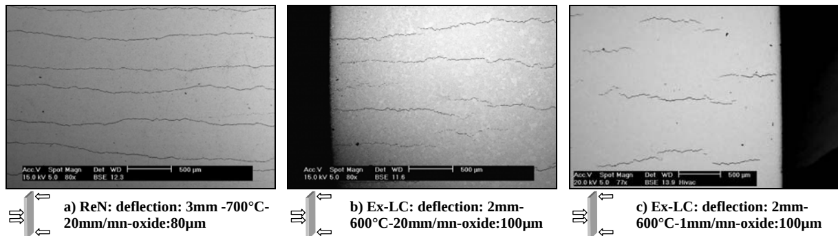
Figure IV-38: Equidistant crack network.
