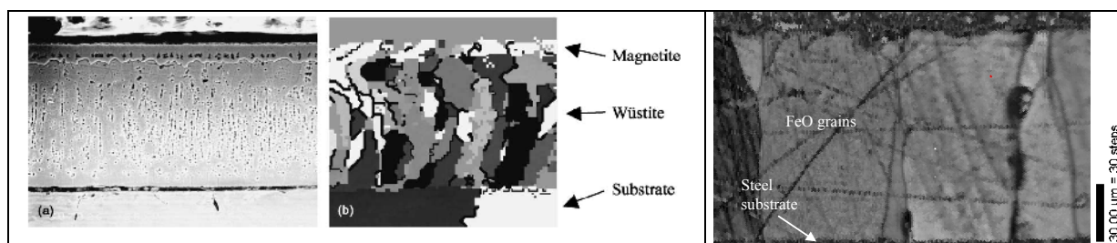
Figure II-19a) An electron micrograph of the oxide scale (70 \mu\text{m} thick, T_{\text{ox}}=760^\circ\text{C} , t_{\text{ox}}=2\text{h} ) grown on an IF steel substrate and its EBSD map showing the different oxides [Hig1].
