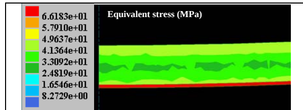
Figure IV-6: 4-PBT simulation using Forge2® of a steel specimen covered by a thin oxide scale on its lower side.
