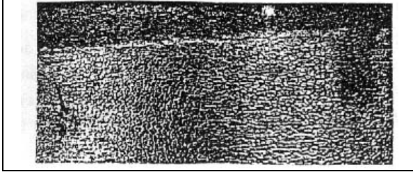
Figure I-23: fire-cracking
