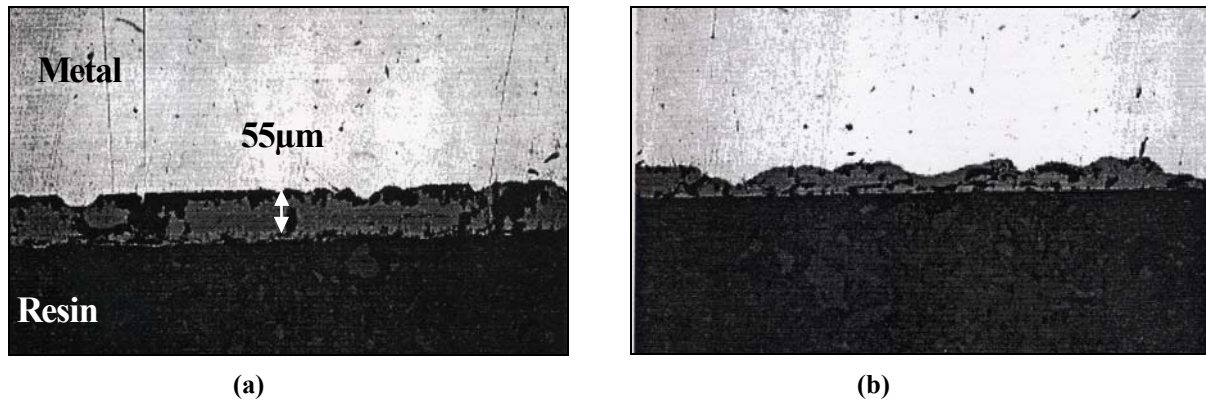
Figure V-30: Micrographs of a DDS specimen cross section after a PSCT. Temp: 800°C, reduction: 50%, velocity: 5 mm/s, initial scale thickness: 55 µm, (a) outer free zone (b) inner compressed zone.
