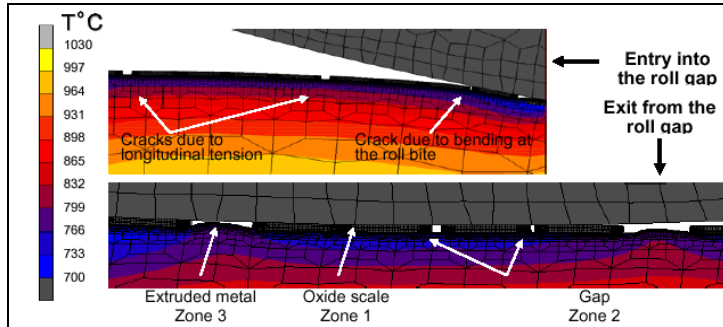
Figure VI-2: Temperature and crack distribution at the oxidized stock-roll interface during hot rolling [Krz3].
