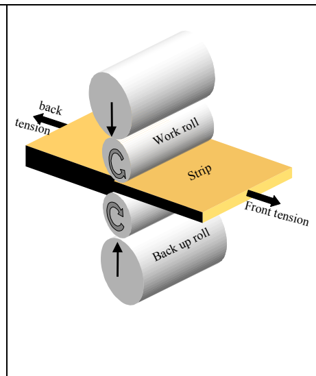
Figure I-3: 4 high stand
