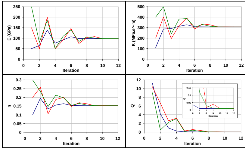
Figure IV-71: Parameters identification on load-deflection curve of Ex-LC steel deformed at 600°C and 1 mm/mn. Three different initial parameters sets (three different colors).
