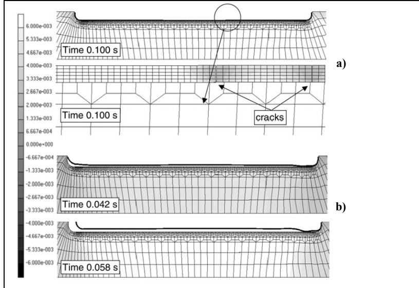
Figure V-6: Distribution of \varepsilon_x strain component predicted for steel at the different time moments during tension under T=975^\circ\text{C} , \varepsilon=5\% , \dot{\varepsilon}=0.2\text{s}^{-1} and \delta_{ox}=170\mu\text{m} . a) Steel 2 b) steel 1 [Krz1, Krz3].
