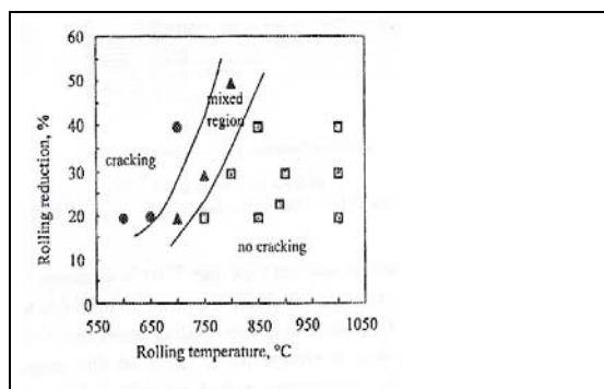
Figure I-46: Hot sandwich rolling results; Scale thickness: 100µm, Speed: 0.14m/s.
