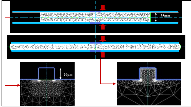
Figure V-42: Simulation of PSCT to study extrusion in cracks. Dimensions used reproduced as close as possible industrial F2 finishing mill stand.
