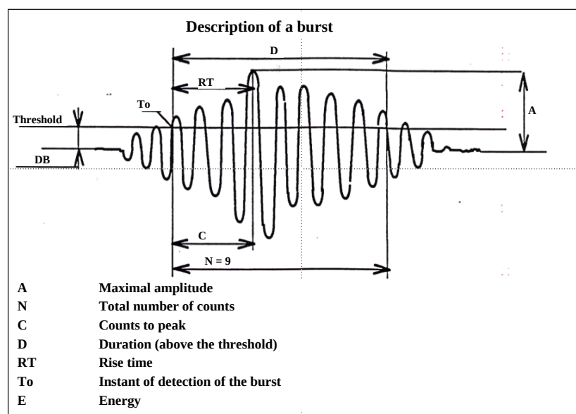
Figure A3-1: Characteristic parameters of a single transient AE wave.
