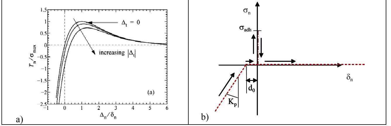
Figure III-12: illustration of the normal stress – displacement relations. (a): CZM-like model of [Abdu] (b) : present strategy, with contact penalty associated with stress-based transitions. In (b): standard contact penalty technique and the added bilateral to unilateral transition; arrows follow a typical separation process.
