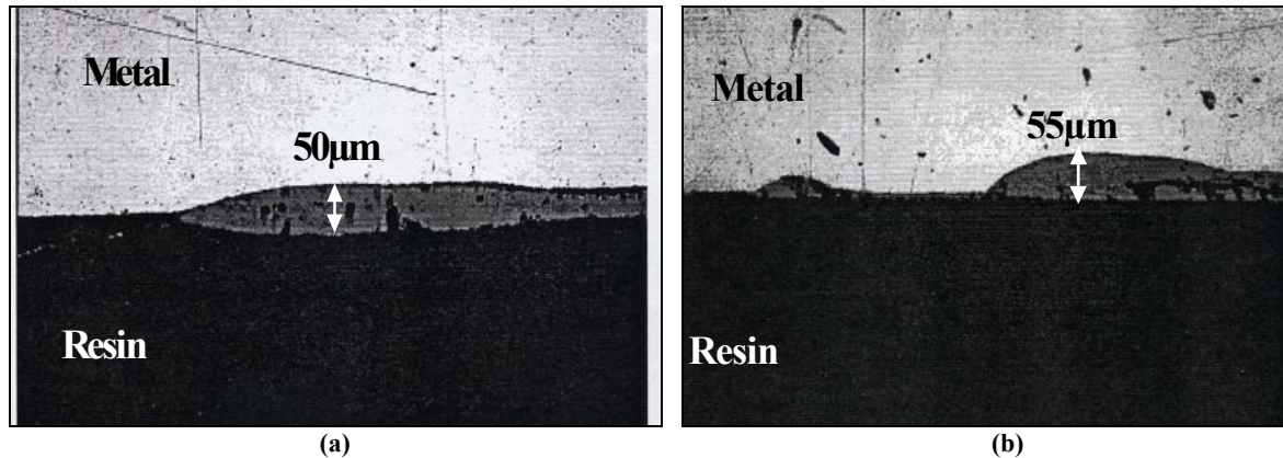
Figure V-32: Micrographs of a deformed specimen cross section after a PSCT. Steel grade: DDS, Temperature of deformation: 800°C, reduction: 30%, velocity: 5 mm/s, initial scale thickness: 50 µm. (a) Free zone (b) Compressed zone.
