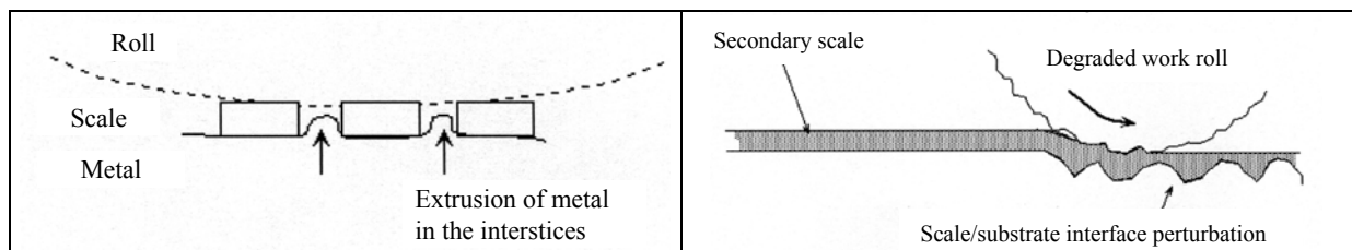
Figure I-33: a) Cracking and extrusion of metal because of its lower hardness compare to these of oxide scale.
