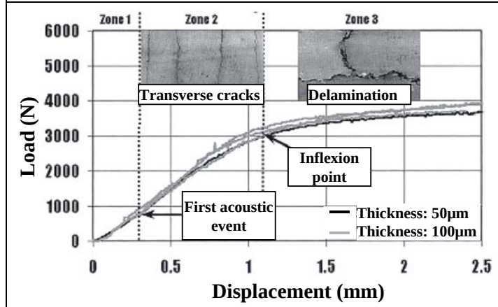
Figure IV-15: Load-displacement curves of specimens covered by two coatings of different thickness [Dalm].
