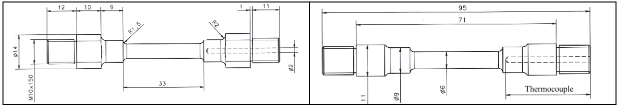
Figure V-10: Schematic representation of tension samples.
