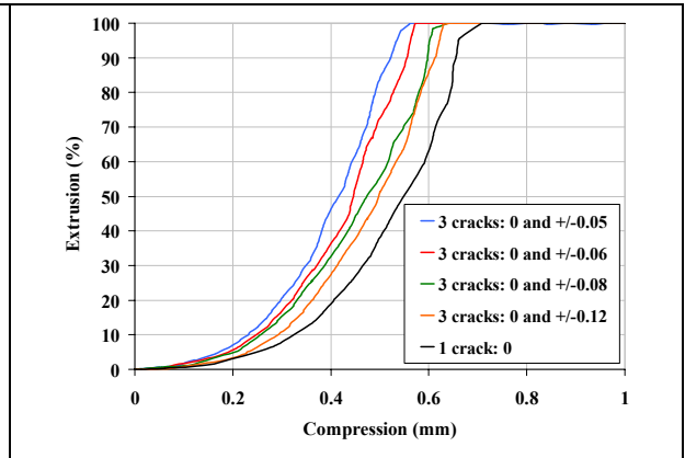
Figure V-45: Evolution of steel extrusion in PSCT as a function of distance between cracks. Crack width: 40 µm.
