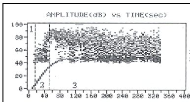
Figure IV-16: Amplitude of events (dB) vs. time (s) + associated load curve (in arbitrary scale) [Dalm].
