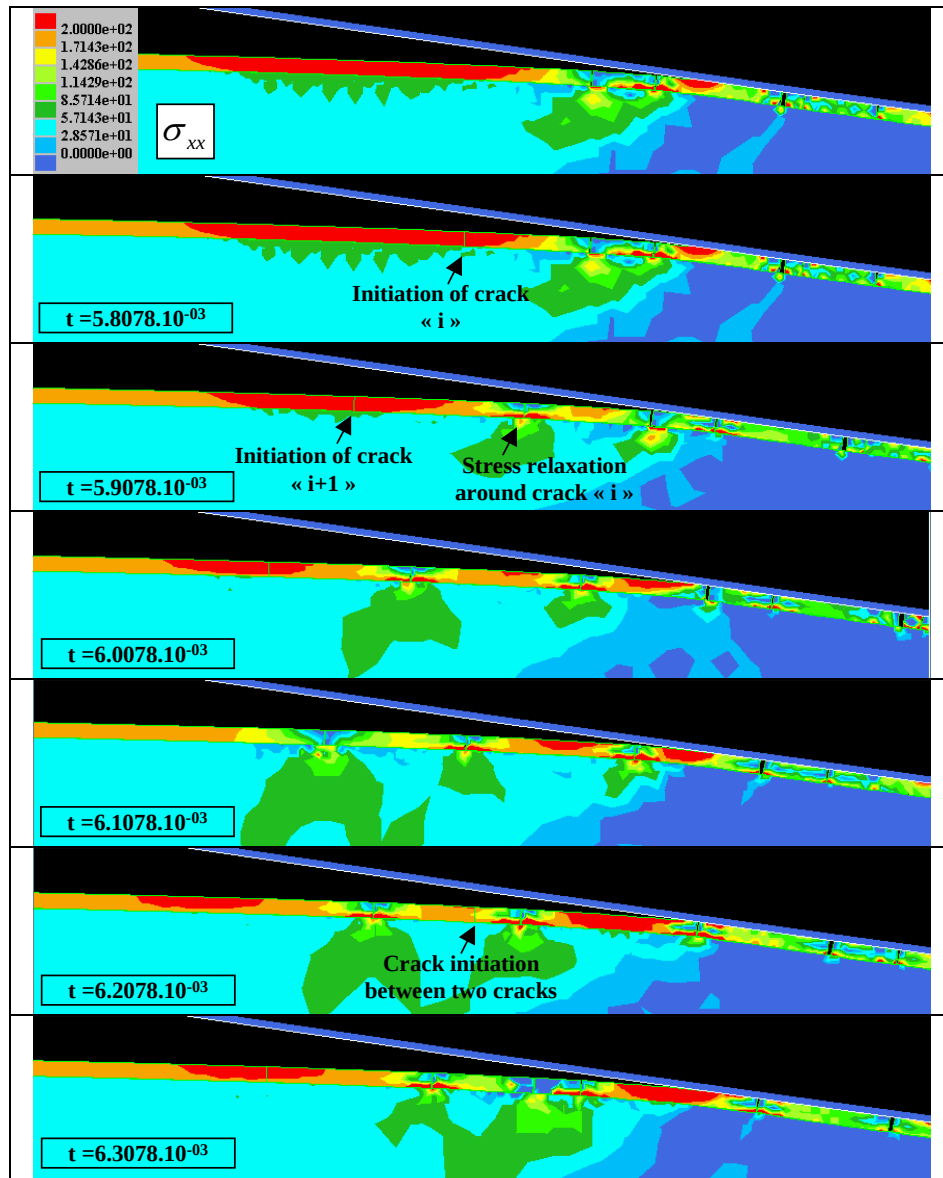
Figure VI-18: F2 conditions. Scale thickness: 50 \mu m.
