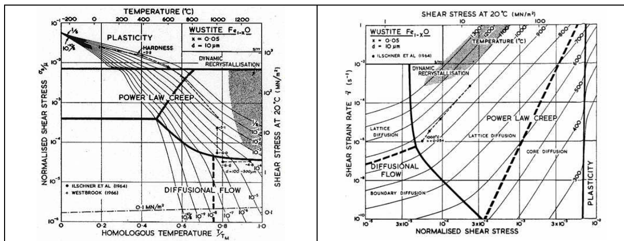
Figure II-32: \text{Fe}_{1-x}\text{O} deformation-mechanism map [Ash2].
