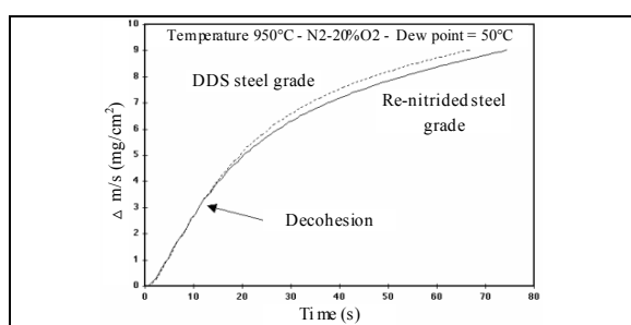
Figure II-27: Evaluation of adherence loss by thermo-gravimetry : the ReN grade is less adherent than the DDS ones.
