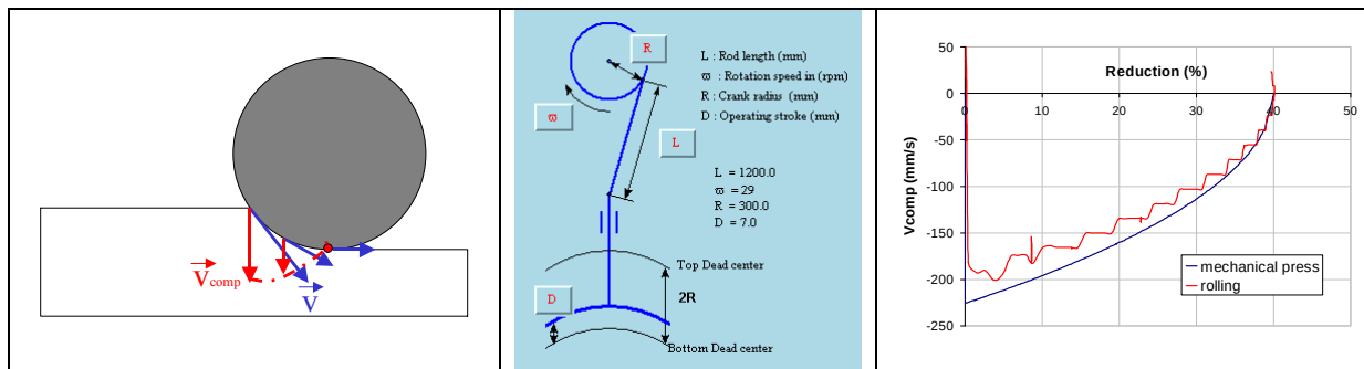
Figure V-43: Identical vertical velocity in rolling and PSCT. Use of the “mechanical press” option of Forge2®.
