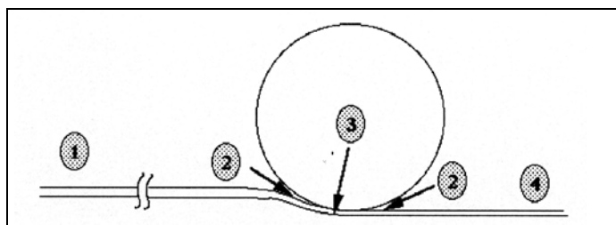
Figure I-32: Stresses developed in the secondary scale during hot rolling.
