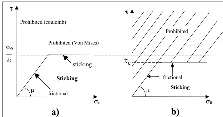
Figure III-9: Representation of Coulomb’s law with von Mises plasticity limit :
