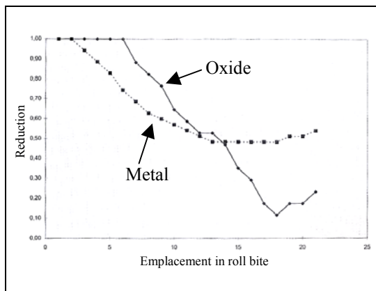
Figure I-45: Reduction in F1 stand
