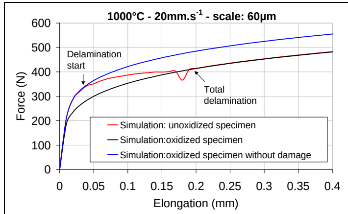
Figure V-23: Load-elongation curves obtained from hot tensile test simulation at 1000°C. Red curve represents simulation seen Figure V-22.
