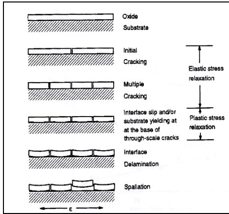
Figure II-47: Delamination and spallation [Nag2]
