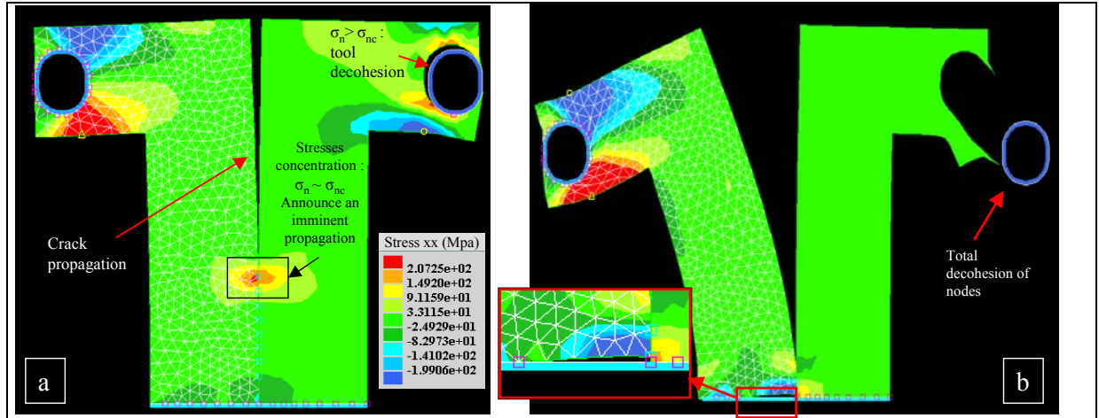
Figure III-18: Simulation at different calculation times.
