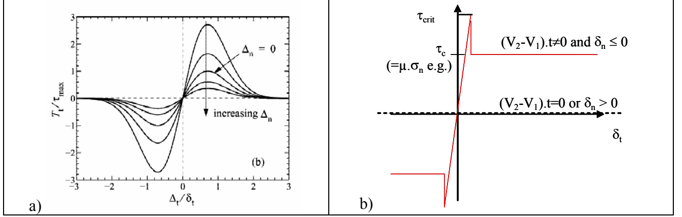
Figure III-11: Illustration of tangential stress – displacement relations. (a): CZM-like model of [Abdu]. (b) : present strategy, with contact penalty associated with stress-based transitions.
