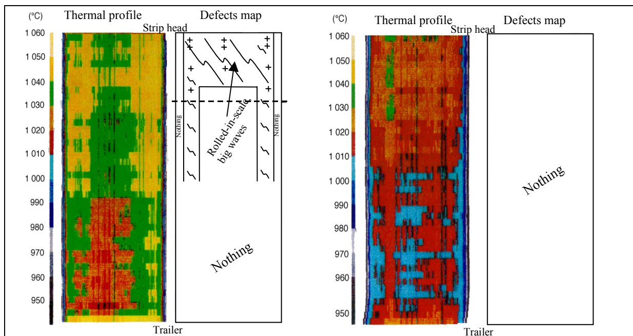
Figure II-24: Defects initiation in hot zones
