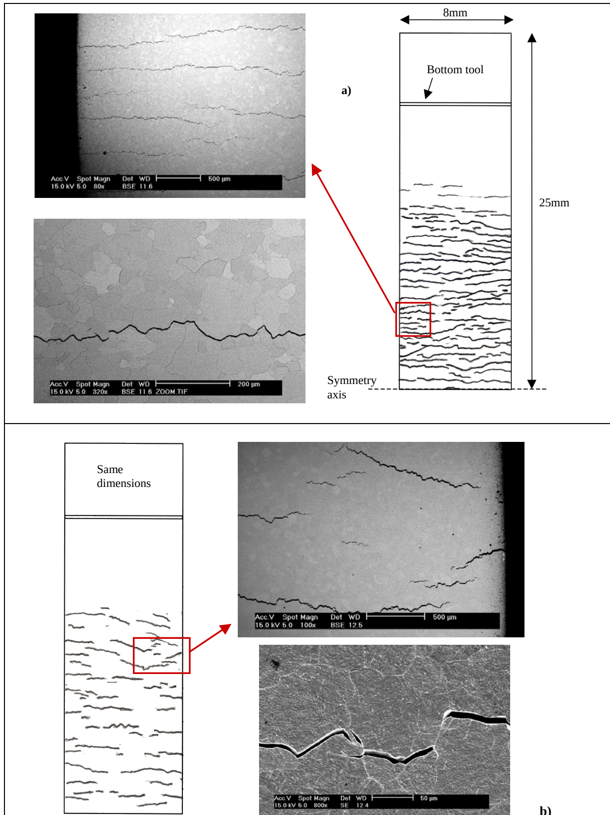
Figure IV-58: Crack maps of half specimens after deformation : T=600^{\circ}\text{C} ; scale thickness = 100\mu\text{m} ; deflection= 2\text{mm}
