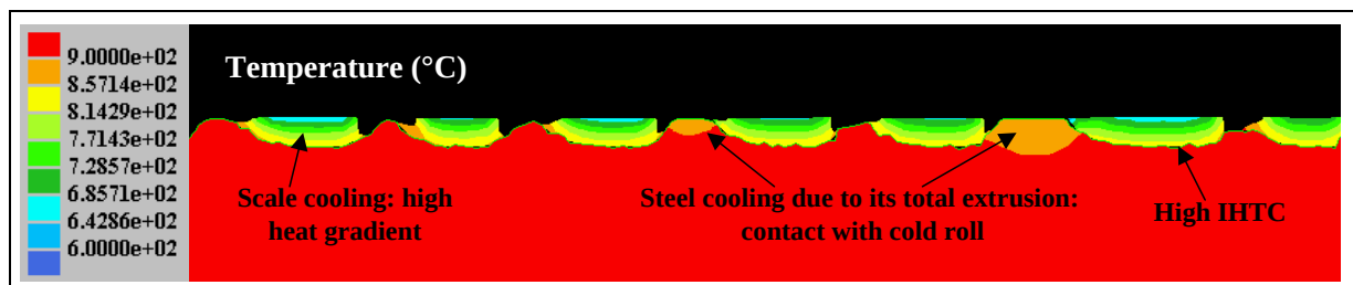
Figure VI-19: Interface cross section at the exit of the roll bite, in the middle of the stock length. Initial scale thickness: 200 \mu m; reduction 45%; \mu = 0.6 ; roll velocity: 2.19 m/s; Strip initial temperature: 900°C.
