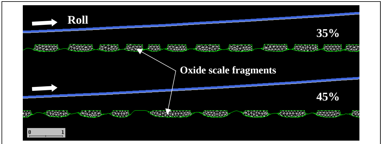
Figure VI-24: influence of reduction. Strip cross sections at the roll bite exit, in the middle of the stock length. Initial scale thickness: 200 \mu\text{m} ; roll / scale contact: \mu = 0.3 .
