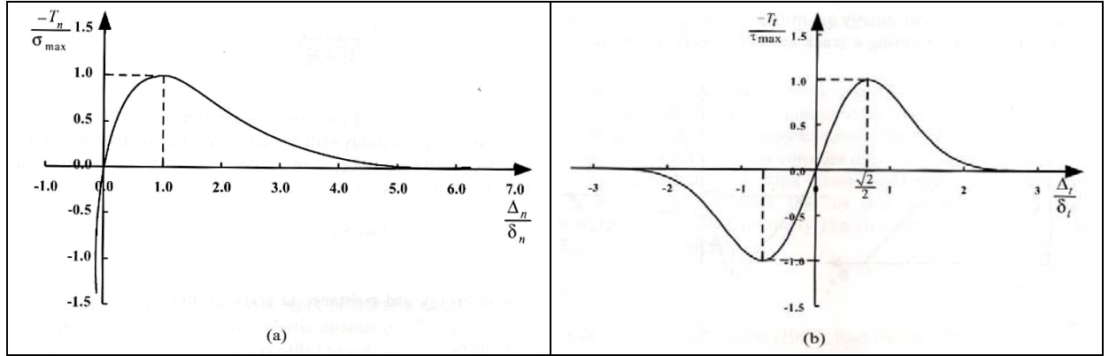
Figure III-8: a) Variations of normal traction, T_n , with \Delta_n for \Delta_t=0 b) Variations of shear traction, T_t , with \Delta_t for \Delta_n=0 .
