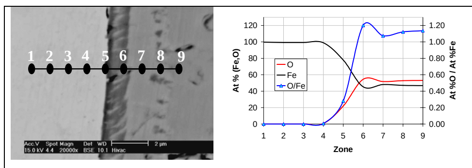
Figure II-18: WDS interface line scan. The % of O increases at the interface.
