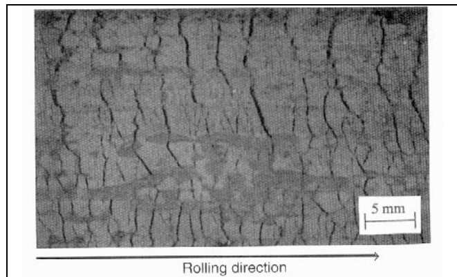
Figure I-27: Transversal cracks after hot rolling [Li5]
