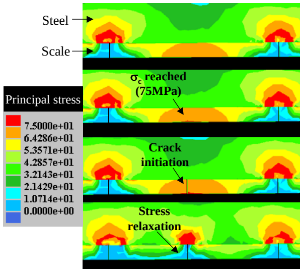
Figure IV-87: Crack initiation halfway between two existing cracks: principal tensile stress is maximal. Simulation at 600°C and 200mm/mn.
