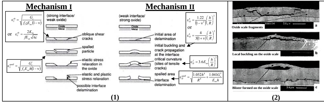
Figure II-50: 1) Schematic diagram of compressive failure mechanisms [Nag4] 2) SEM images illustrating decohesion on compression side of steel rod during bending [Krz1] a) cracked oxide scale b) buckling c) blister formed during oxidation
