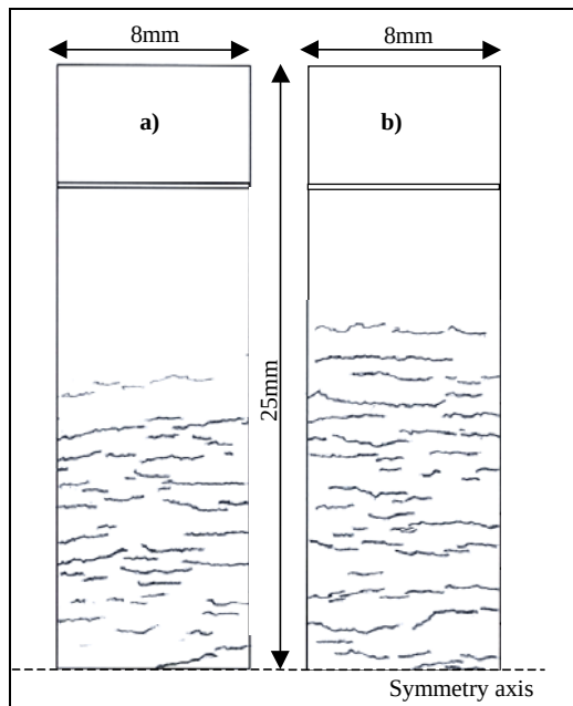
Figure IV-62: Crack maps of half-specimens after deformation : T=600^{\circ}\text{C} ; scale thickness = 70\mu\text{m} ; v=1\text{ mm/min} a) Test n°3 : deflection= 0.7\text{ mm} b) Test n°4 : deflection = 2\text{ mm}
