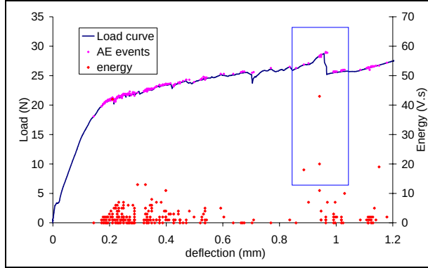
Figure IV-66: Test n°4. Highly energetic events near the load drop.
