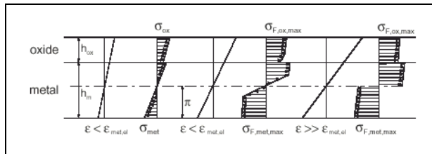
Figure IV-5: Schematic Stress-strain distribution in the cross section of an oxidized bent bar [Echs].
