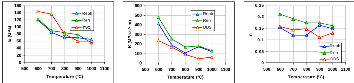
Figure IV-76: Graphical representation of parameters evolution with temperature for the three steel grades.
