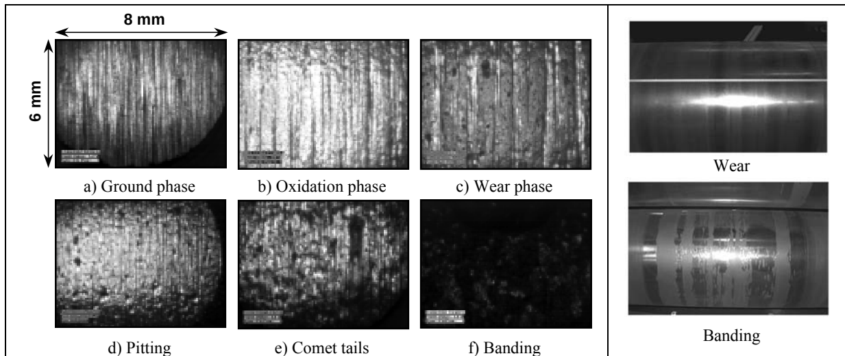
Figure I-24: Roll surface evolution during its lifetime.
