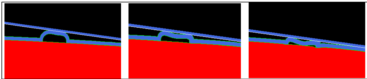
Figure VI-34: Evolution of the blister shape at the entry in the roll bite.
