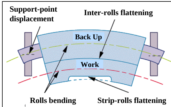
Figure I-5: Rolls bending and flatness [Ber].
