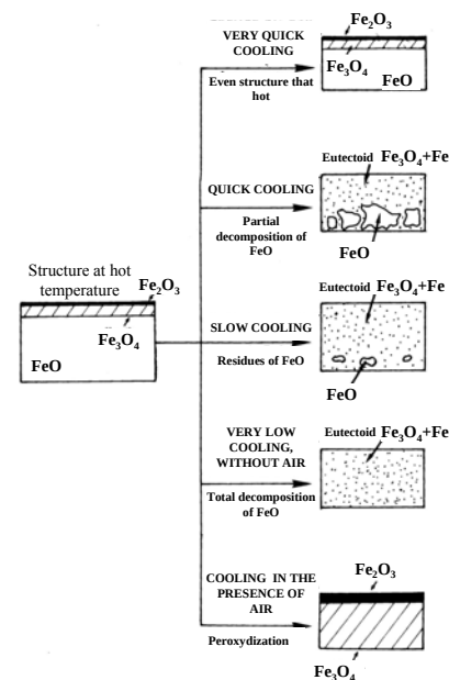
Figure II-5: Oxide decomposition depending on cooling speed.
