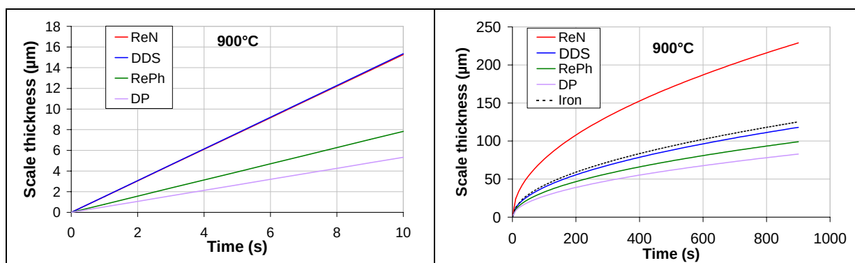
Figure II- 9a: Linear growth at 900°C for the four steel grades.
