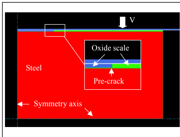
Figure V-35: Numerical simulation of compression test: 800°C - V_{comp}=50 mm/s. Pre-crack closed. Initial scale thickness: 100 \mu\text{m} .
