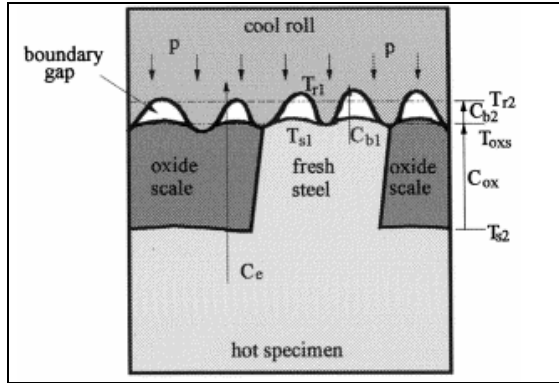
Figure I-19: Consequences of the oxide layer damage on the IHTC [Li3].
