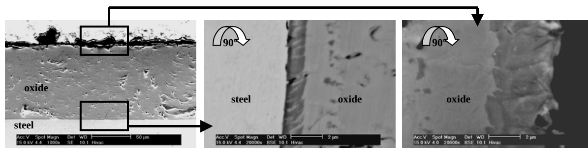
Figure II-14: SEM micrographs of specimen cross section. Presence of two different phases in scale.
