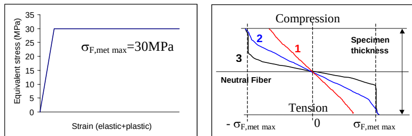
Figure IV-3: Computation using Forge2®. Left: Ideal plastic behavior. Right: Stress-strain dependence during the 4-PBT.
