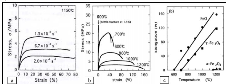
Figure II-31: a) FeO behavior at various strain rate b) FeO behavior at various temperature and at 2.10^{-4} \text{ s}^{-1} c) Elongation of iron oxides in function of the temperature at 2.10^{-4} \text{ s}^{-1} .
