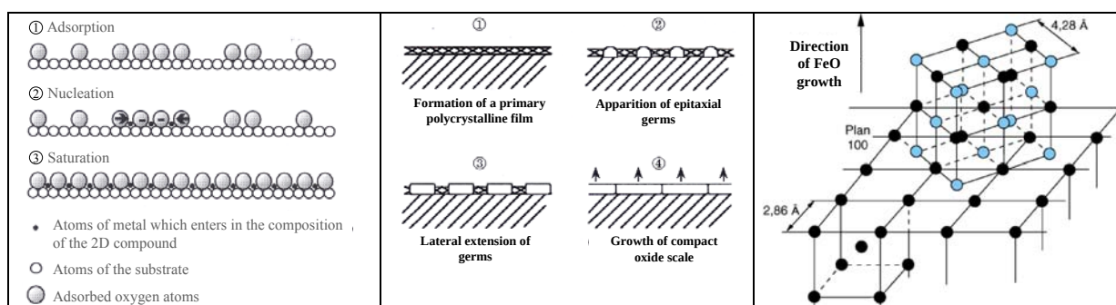
Figure II-1: Mechanism of surface saturation [Bar]
