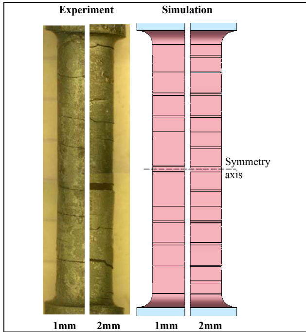
Figure V-19: Samples deformed at 900°C and 10 mm.s -1 using HTT. Experiment / simulation comparison.
