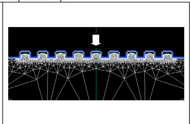
Figure V-48: Simulation of compression tests: extrusion in 9 cracks corresponding to the red curve plotted Figure V-46. Stroke = 0.52 mm.
