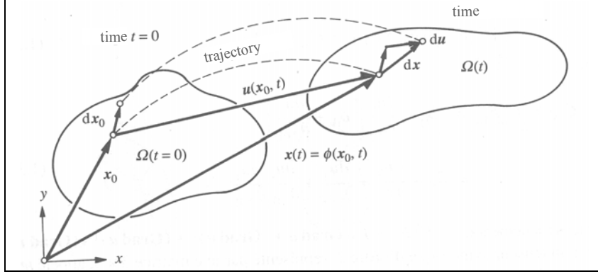
Figure III-6: Updated Lagrangian small time steps.
