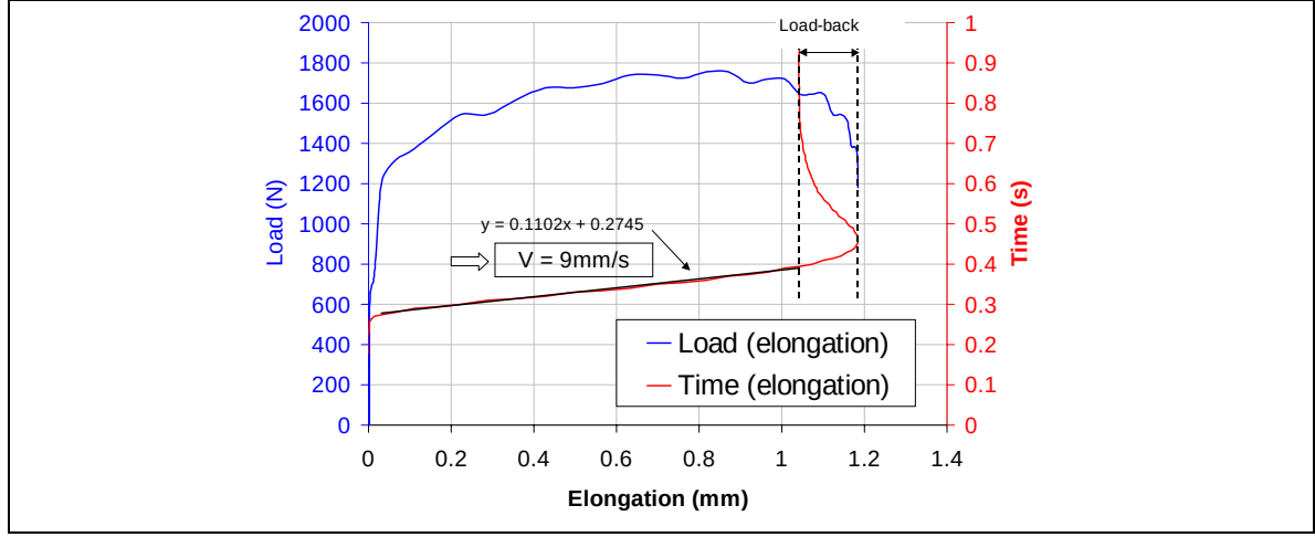
Figure V-18: Representation of HTT load-elongation curve shape. HTT performed at 800°C.
