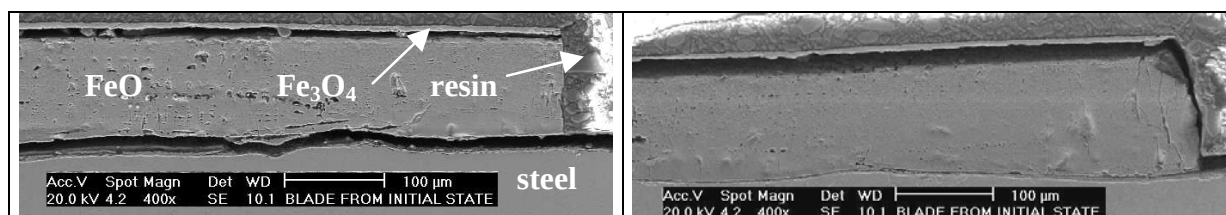
Figure II-12: Decohesion induced during the specimen preparation. Resin shrinkage.
