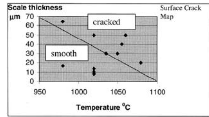
Figure I-57: Surface crack map for low and ultra low carbon steel [Ti1].
