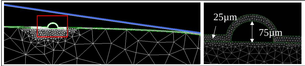
Figure VI-33: Numerical representation of an initial blister defect.
