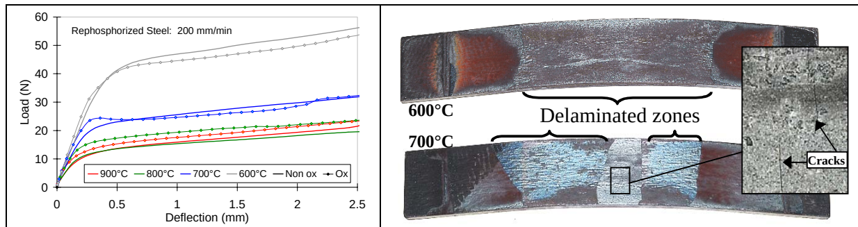
Figure IV-49: ReP: 4-PHBT curves obtained at 200mm/mn. deflection: 3mm - oxide:90µm
