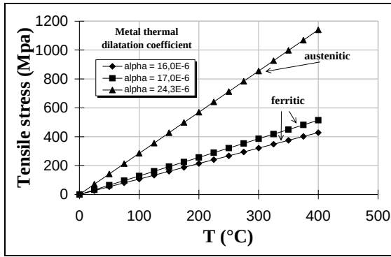
Figure II-40: Thermal stresses developed in FeO scale for different values of steel thermal dilatation coefficient. E_{ox}=150\text{GPa} ; \alpha_{ox}=11.10^{-6} ; \nu=0.3 .
