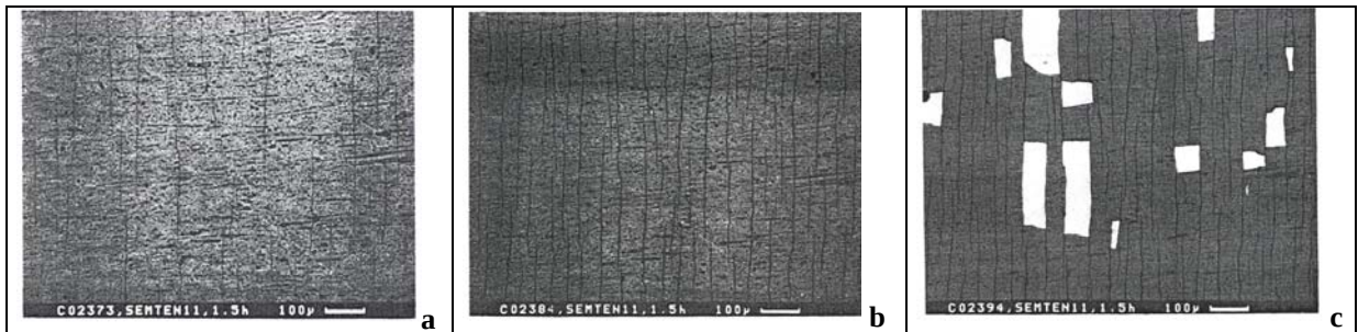
Figure II-49: SEM micrographs showing through-thickness cracks during tensile tests at room temperature. Scale thickness: 9.5μm. Strains: a) 0.54% b) 1.21% c) 2.3% [Nag3].
