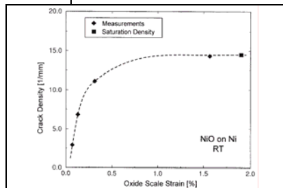
Figure IV-11: Crack densities in the oxide represented just above.
