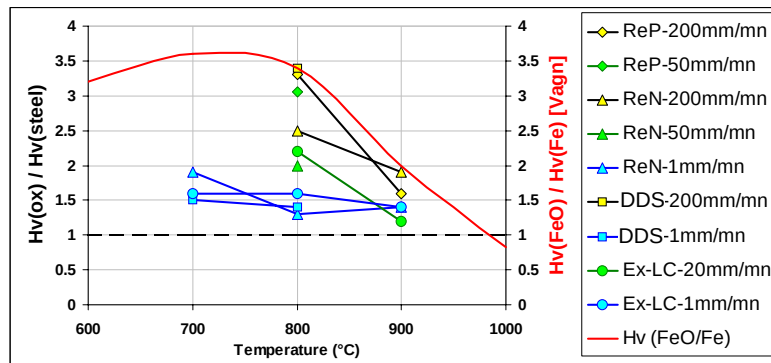
Figure IV-79: hardness ratio between oxide scales and their respective steel. Evolution as a function of steel grade, temperature and strain rate.
