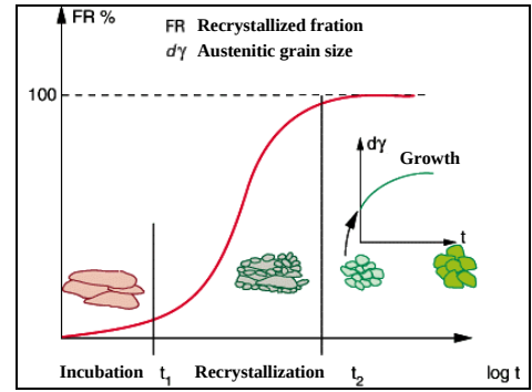
Figure I-12: Kinetics of static recrystallization.
