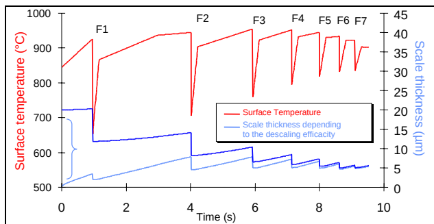
Figure I-15: example of thermal calculation and the corresponding thickness evolutions of a scale in an industrial FM (IRSID).
