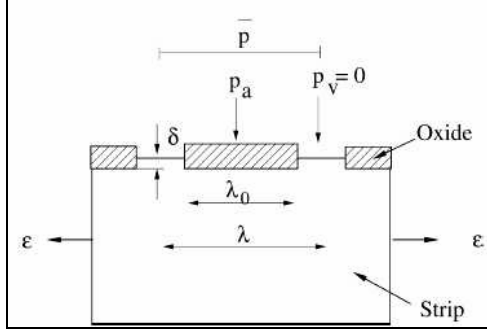
Figure II-53: Metal extrusion through the oxide cracks [Le]
