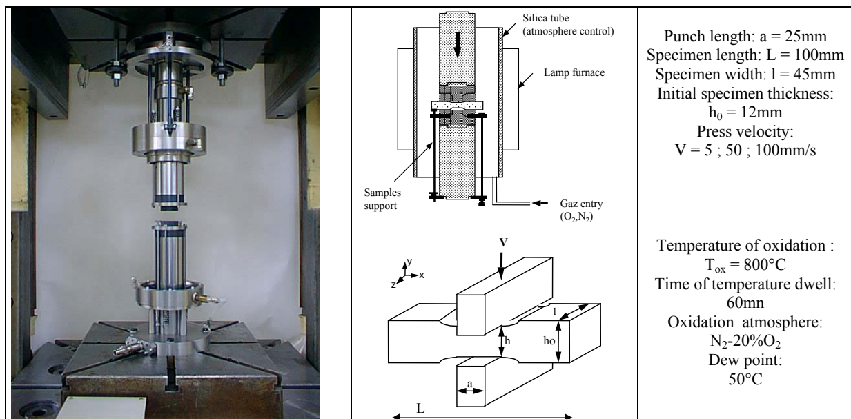
Figure V-29: The PSCT fixture and its schematic representation. Description of PSCT thermal and chemical cycles.
