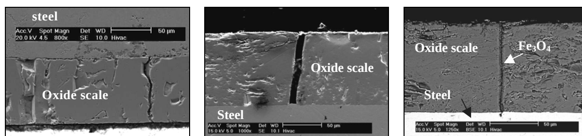
Figure IV-41: Micrographs of through-thickness cracks: Ex-LC: deflection: 2mm - 600°C -1mm/mn-oxide:100µm. Left and middle : micrographs in SE mode / Right : micrograph in BSE mode: FeO is decomposed in Fe 3 O 4 ⇒ mechanical crack.
