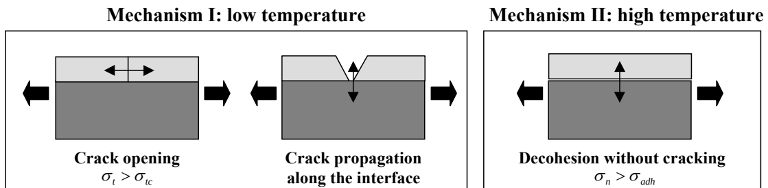
Figure V-8: Stress criteria of damage mechanisms at low and high temperature cannot be compared to a same separation stress. \sigma_t is the tensile stress within the oxide and \sigma_{ic} its critical value. \sigma_n is the normal stress at the interface and \sigma_{adh} its critical adherence.
