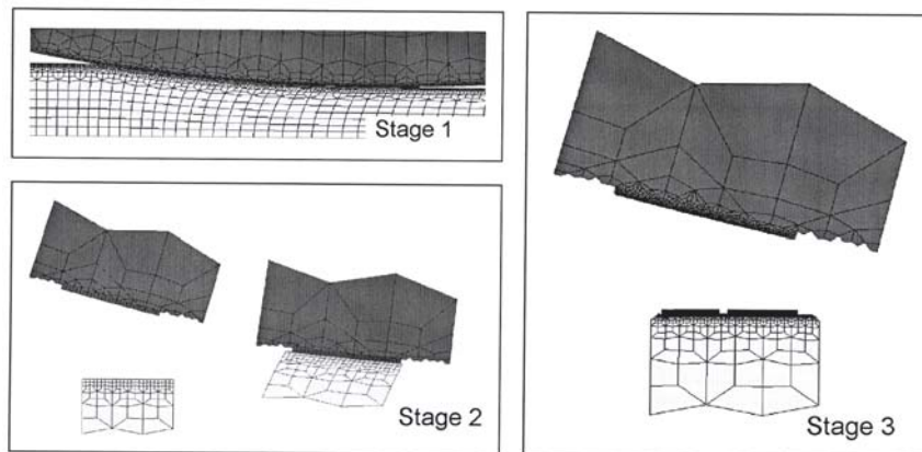
Figure VI-8: Schematic representation of model adjustment stages for evaluating the final state of the surface layer after flat hot rolling.
