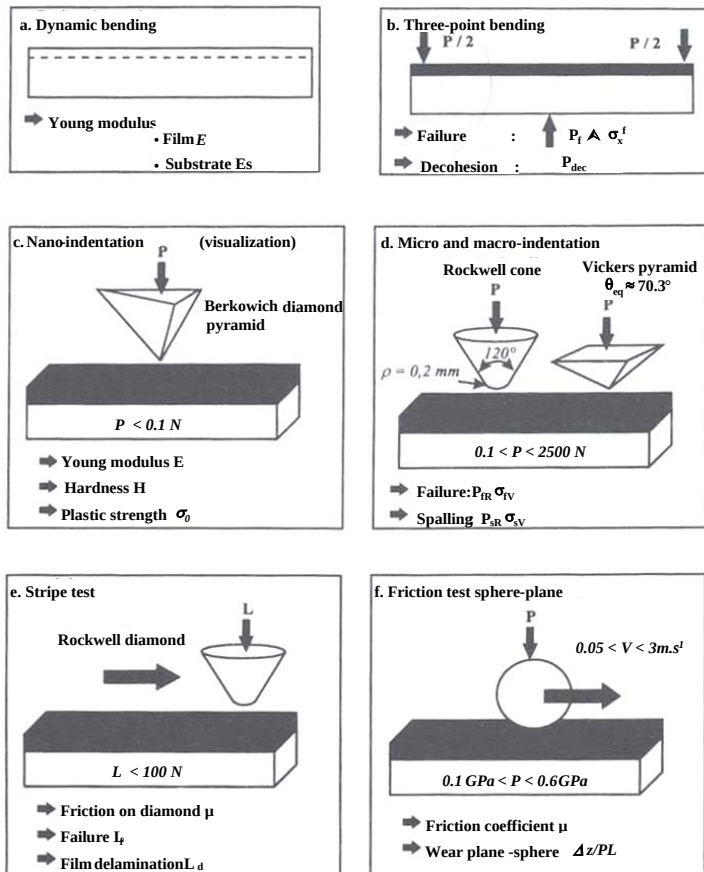
Figure II-25: Mechanical characterization tests.
