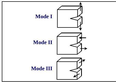
Figure II- 36: Fracture modes.
