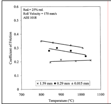
Figure I-14: Influence of scale thickness on friction coefficient [Munt].
