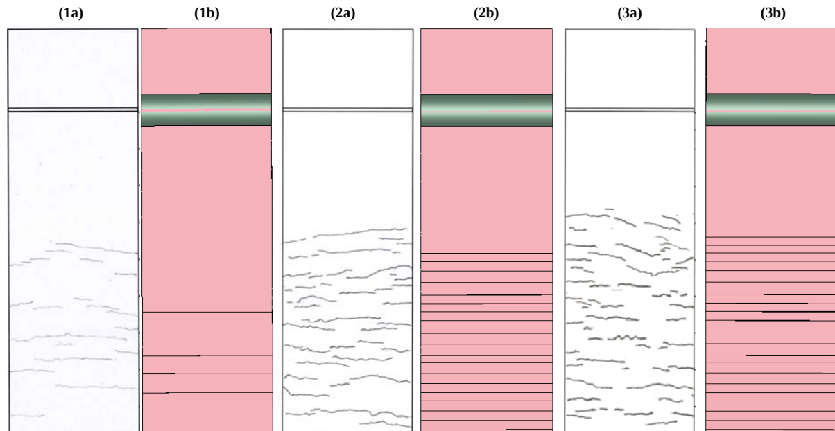
Figure IV-84: Ex-LC deformed using 4-PHBT: 600°C – 1 mm/min - oxide: 100 \mu m. (a) crack mapping of experimental oxidized samples (b) 2D simulation, represented in a 3D configuration for clarity. (1) Deflection = 0.25 mm (2) deflection = 1.2 mm (3) deflection = 2 mm.
