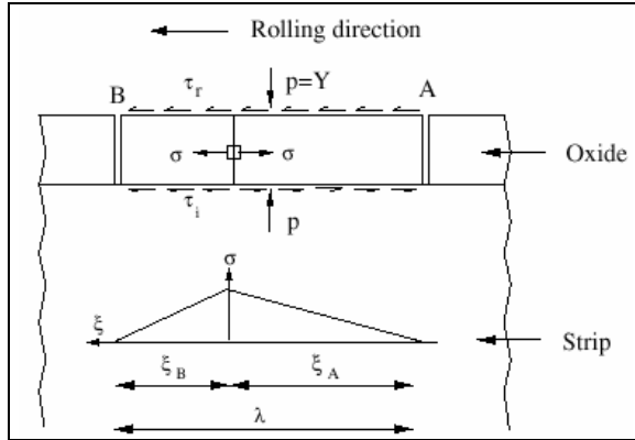
Figure II-52: Model of roll bite oxide fracture due to extension of the substrate metal during rolling [Le]
