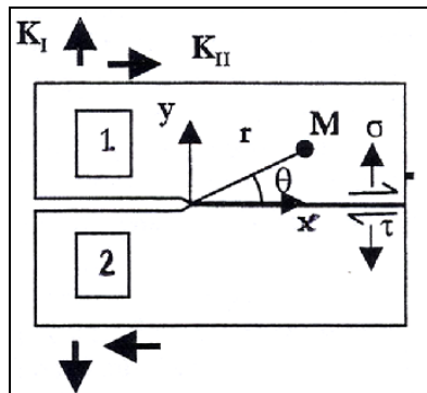
Figure II-37: Interfacial crack representation [Dup].
