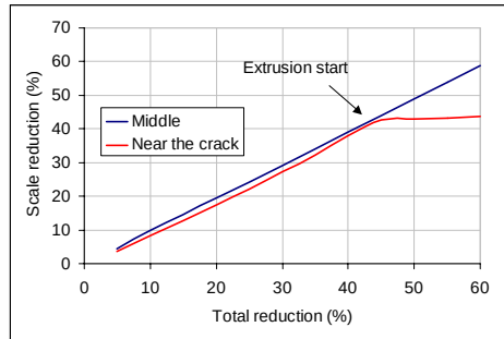
Figure V-40: Extrusion influence on scale reduction (near a crack).
