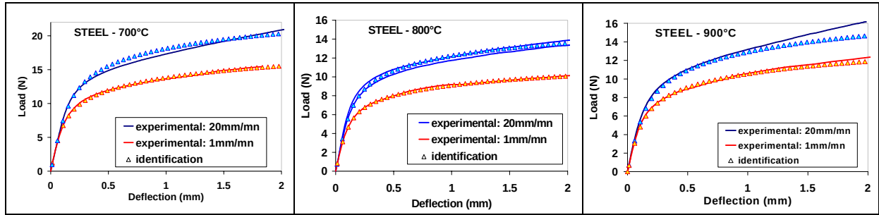
Figure IV-75: Comparison between simulated load-deflection curves (using the identified constitutive parameters) and the Ex-LC experimental curves.
