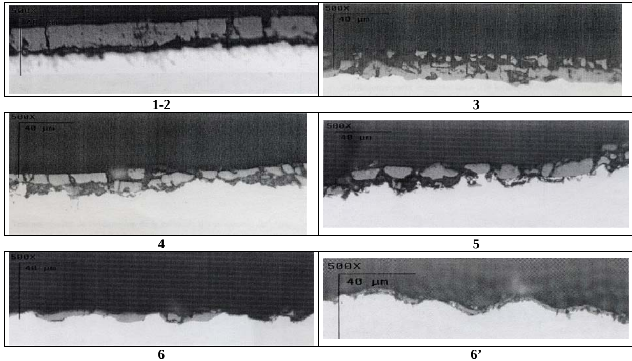
Figure I-44: Secondary scale evolution in stand F1 of the Dunkerque FM.
