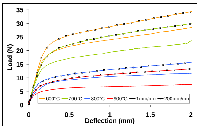
Figure IV-34: Curves of DDS non-oxidized steel tests
