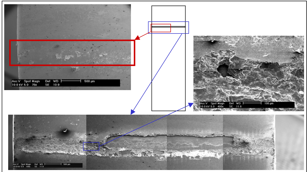
Figure IV-68: Red box: test n°3. Sliding contact between tools and scale : no damage. Blue box: test n°4. Sticking contact: crackling and interface cracks.
