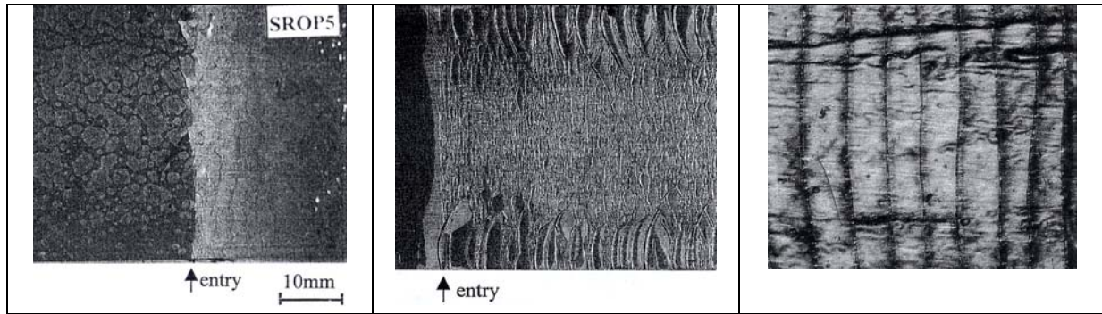
Figure I-50: Oxide scale. Temperature: 890°C, scale thickness: 40µm, reduction: 40%.
