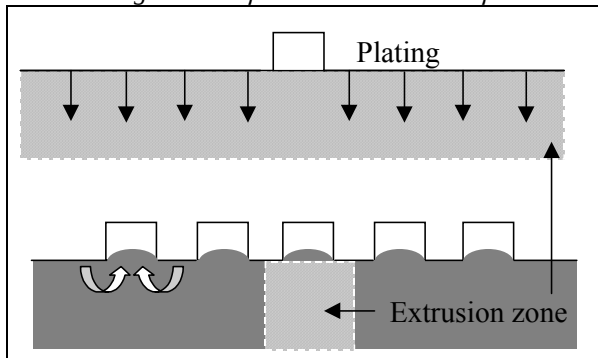
Figure V-50: nearby cracks enhance extrusion.
