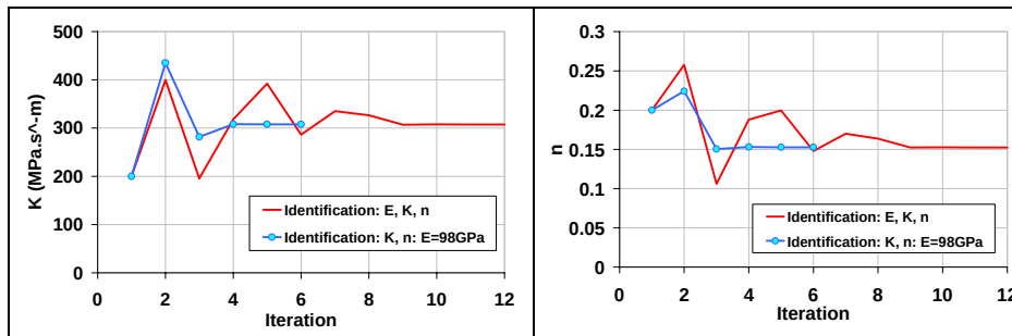
Figure IV-74: Identification of K and n with or without the identification of E.
