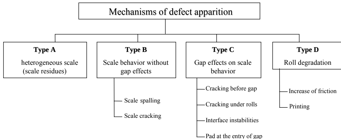
Figure I-34: Decomposition of defect formation related to secondary scale.
