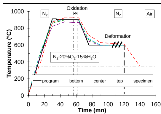
Figure IV-26: Samples thermal cycle of 4-PHBT.
