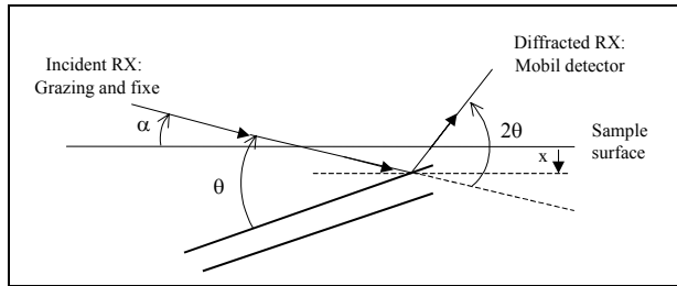
Figure II-15: Incident and diffracted beam.
