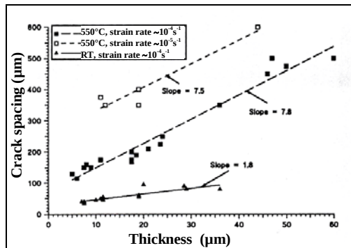
Figure II-46: Crack spacing vs. scale thickness.
