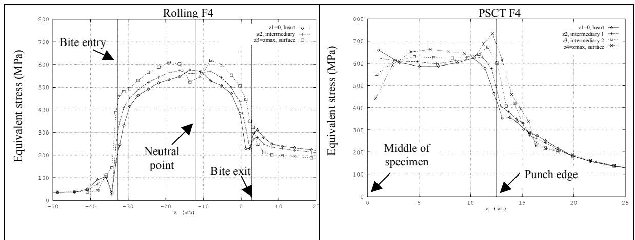
Figure V-26: In bite equivalent stress distribution \sigma_{eq} , at the strip center.
