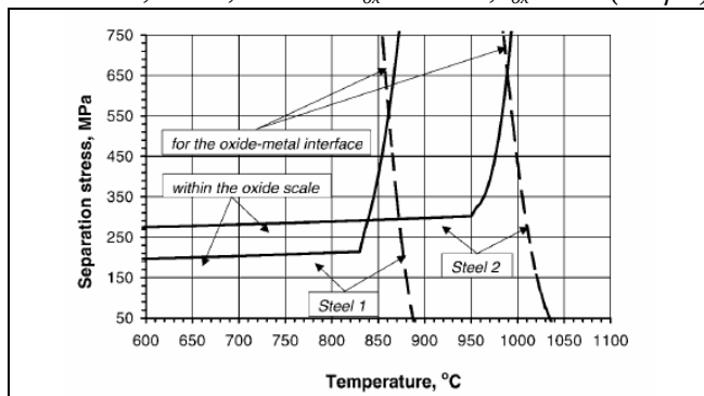
Figure V-5: Effect of temperature on the separation stresses of scale/metal system for two mild steel grades. Model assumption [Krz1, Krz3].
