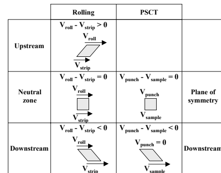
Figure V-28: Simulation of a roll bite using PSCT schematic strain pattern
