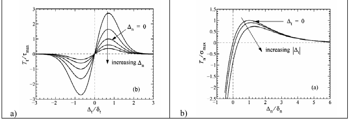
Figure III-7: illustration of the normal (a) and tangential (b) stress – displacement relations. (a,b): CZM-like model of [Abdu]: damage by sliding in the tangential direction decreases adhesion in the normal direction, and vice-versa.
