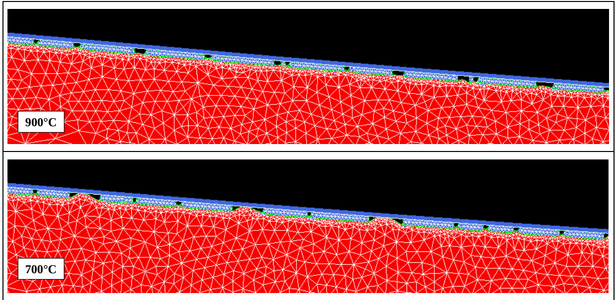
Figure VI-22: Strip cross sections inside the roll bite, under the rolls, at the same location. Same simulations as on Figure VI-21.
