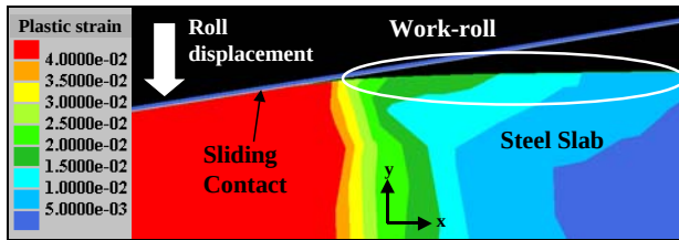
Figure IV-28: Compression test under hot rolling conditions.
