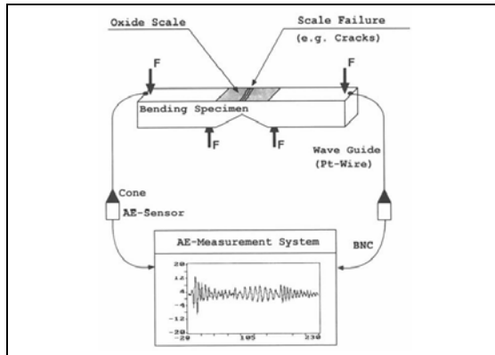
Figure IV-8: Schematic of the test arrangement. The V-shape focuses the deformation in the specimen center [Brun].
