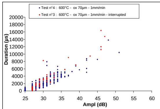
Figure IV-65: Superposition of acoustic signature for both oxidized sample tests. A correlation between the duration and the amplitude reveals a mechanical behavior: here, crack opening.
