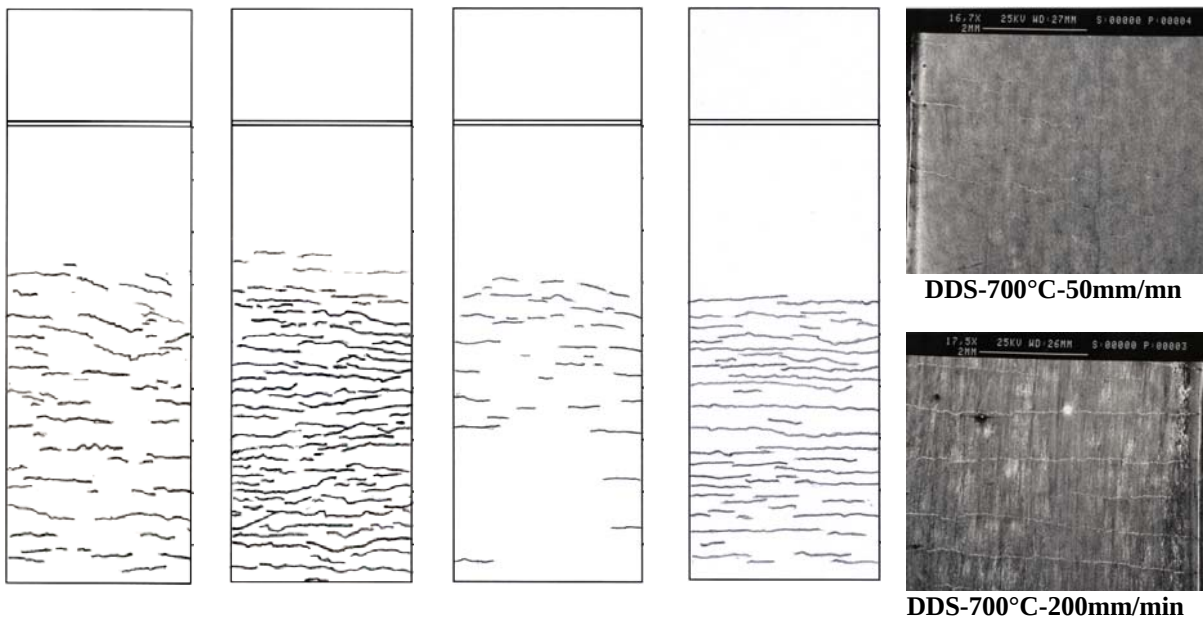
Figure IV-52: Ex-LC: 600°C-deflection = 2 mm - 100µm. Left : 1 mm/min ; Right : 20 mm/min
