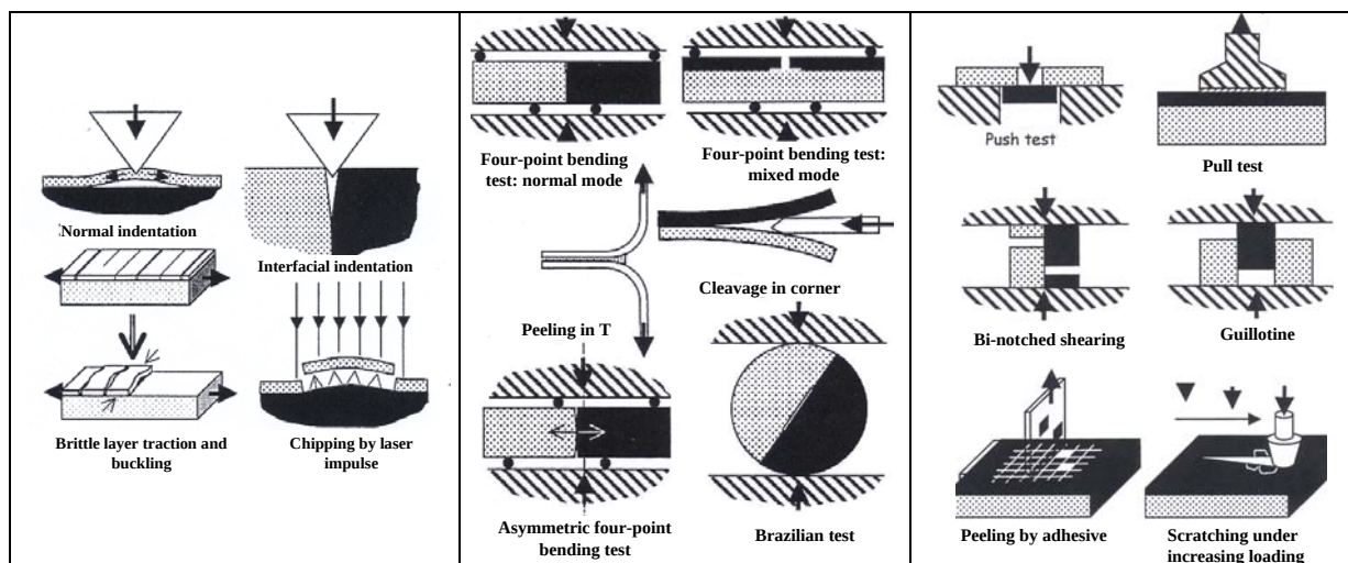
Figure II-26 a) Measurement of decohesion threshold.
