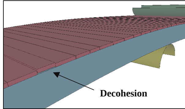
Figure IV-92: Simulation of specimen deformed at 200 mm/mn and 600°C, with decohesion.
