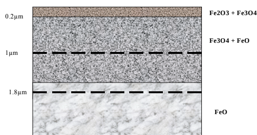
Figure II-17: Schematic representation based on the results obtained in XRD.
