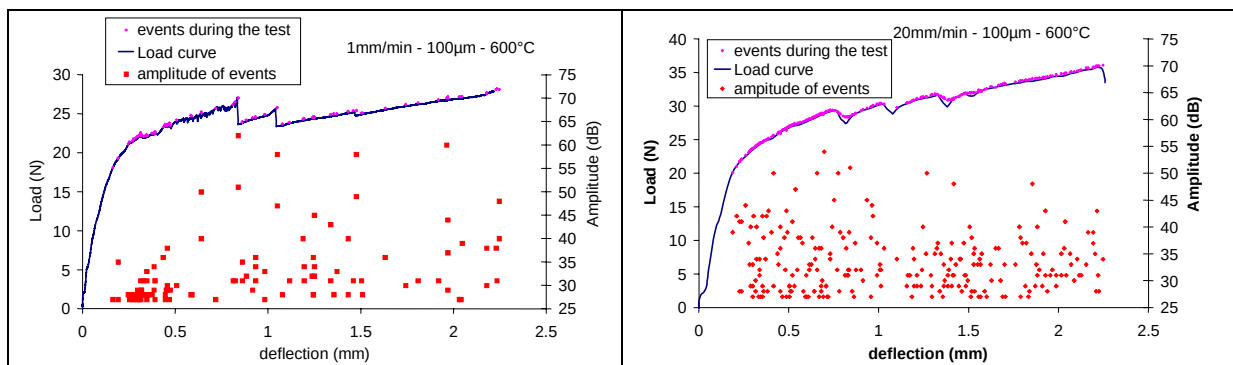
Figure IV-59: AE of test n°2 at 1 mm/min
