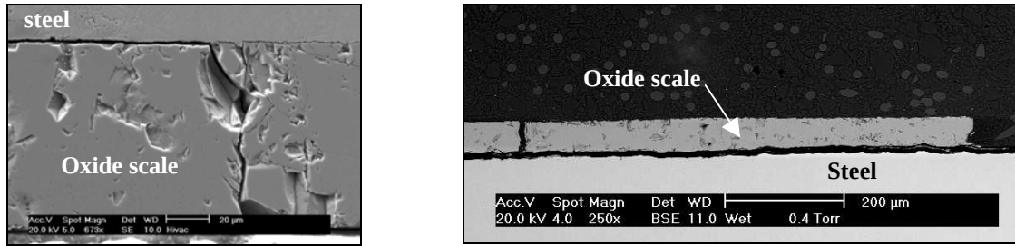
Figure IV-42: Micrographs of a through-thickness crack followed by an interfacial crack. Left : Ex-LC: deflection: 2mm-600°C-1mm/mn-oxide:100µm / Right : Rep: deflection:5mm-600°C-1mm/mn-oxide:60µm.
