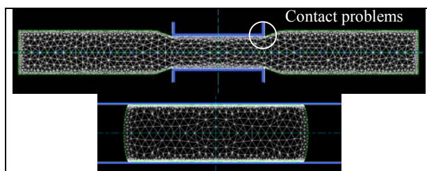
Figure V-33: numerical simulations of PSCT. Simplification of the test.
