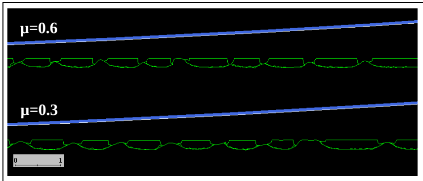
Figure VI-28: Roll / scale friction influence on the steel extrusion.
