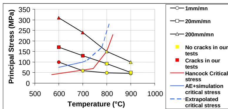
Figure IV-83: Representation of simulated maximal principal stresses reached in a 100 μm-thick scale covering Ex-LC steel samples, at a deflection of 2 mm. Representation of critical principal stress obtained by AE and extrapolation. Comparison with Hancock results [Han].
