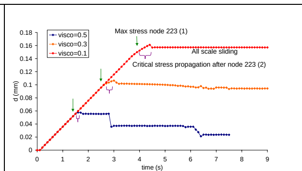
Figure III-15: Displacement of node n°223 along x-axis.
