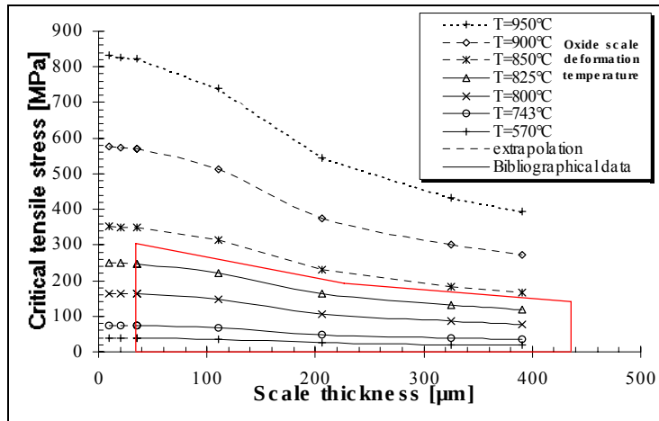
Figure II-43: Critical tensile stress depending on scale thickness and temperature.
