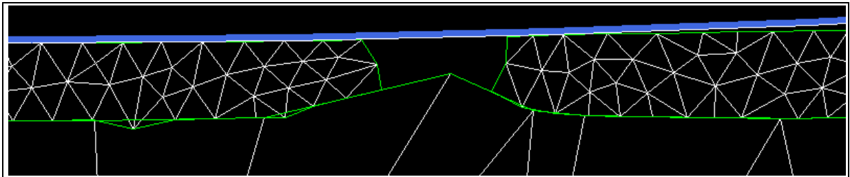
Figure VI-10: extrusion of steel in the roll bite is Impossible due to too large a mesh size for steel.
