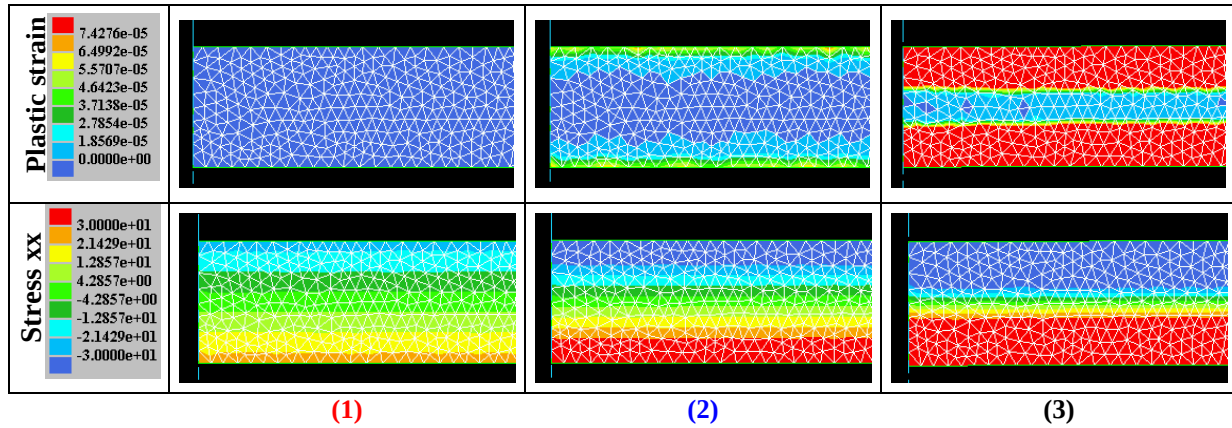
Figure IV-4: 4-PBT simulation of a steel specimen using Forge2®. Visualization of plastic strain and tensile stress (xx) at the three stages of the simulations of Figure IV-3.
