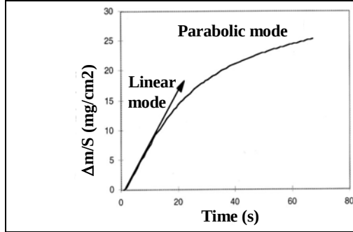
Figure II-7: \Delta m/s=f(t) curve for a DDS steel oxidized at 950°C in a N_2 -20% O_2 -15% H_2O atmosphere.
