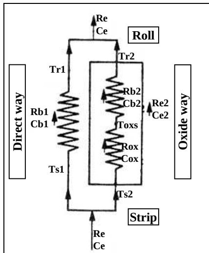
Figure I-20: Thermal circuit [Li3].
