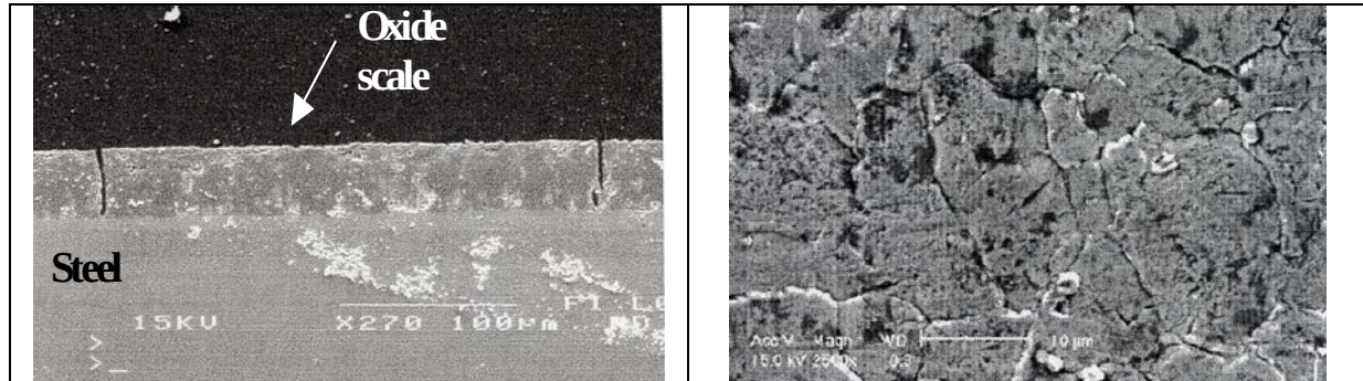
Figure IV-19: Micrograph of specimen oxidized in air at 900°C and deformed at 650°C [Mou2].
