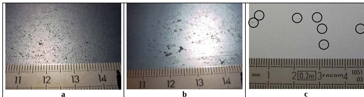
Figure I-29: Arcelor HSM observations: Consequences of rolled-in scale defects initiated in the FM (a), still present on the hot rolled coils (b) and on the cold rolled sheet (c).
