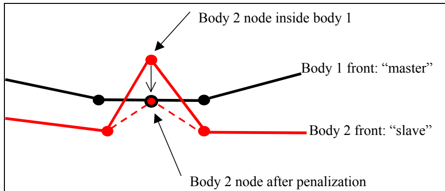
Figure III-4: Illustration of the master-slave version.
