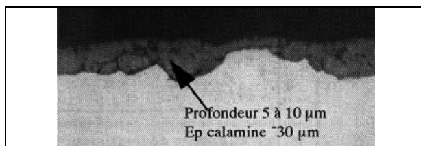
Figure I-28: Rolled-in scale defect: industrial strip; scale thickness=30 \mu m; defect depth=5-10 \mu m.
