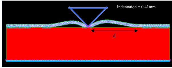
Figure III-20: d = 7,51\text{mm} . Low coupling: \sigma_{nc} decreases by 10% of its original value \sigma_{nc0} .
