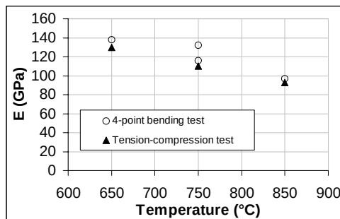
Figure IV-36: Stainless steel chemical composition (in 10 -3 % in weight) and Young's modulus measured on specimens tested on 4-PHBT and tension-compression test at several temperatures.
