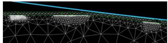
Figure VI-15: Steel mesh refinement at each crack initiation.
