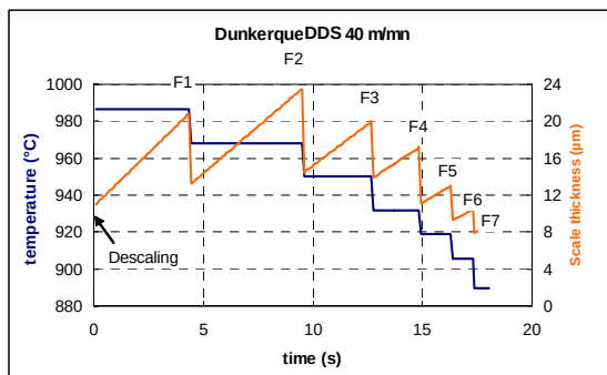
Figure II-22: DDS steel: Maximal scale thickness in stand F2.
