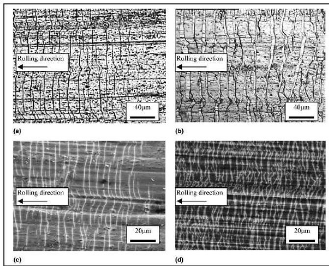
Figure I-59: Micrographs showing cracks on the strip surface. Reduction=30%: a,c) entry of roll bite; b,d) exit; a,b) h=1.8\mu\text{m} ; c,d) h=0.22\mu\text{m} .
