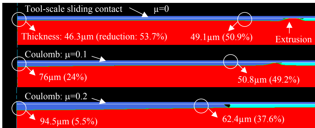
Figure V-39: Influence of tool-scale friction on scale reduction and steel extrusion. Strip reduction: 55% - Initial scale thickness 100 \mu\text{m} – Temperature: 800°C – V_{\text{comp}}=50 mm/s.
