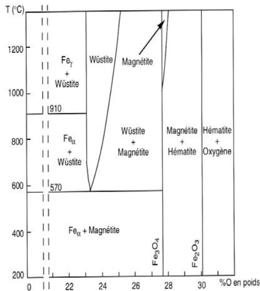
Figure II-4: Equilibrium Fe-O diagram.
