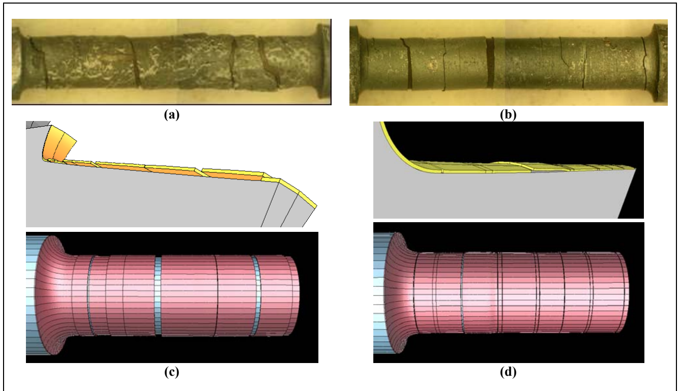
Figure V-20: HTT performed at 8 mm.s -1 . Oxide thickness: 60 μm, elongation 2 mm (a) experimental 700°C (b) experimental 900°C (c) numerical 700°C, \sigma_{tc} = 180 MPa, \sigma_{ip} = 180 MPa (d) numerical 900°C, \sigma_{tc} = 180 MPa, \sigma_{ip} = 130 MPa.
