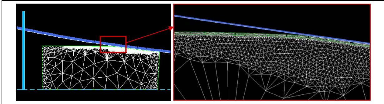
Figure VI-16: Steel mesh refinement at the location and at the moment of the crack initiation.
