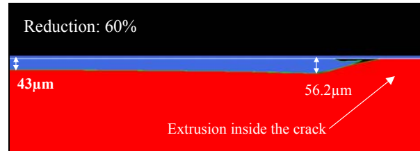
Figure V-41: Scale swelling near the extrusion. Initial scale: 100µm – Temp: 800°C – V_{comp}=50 mm/s.
