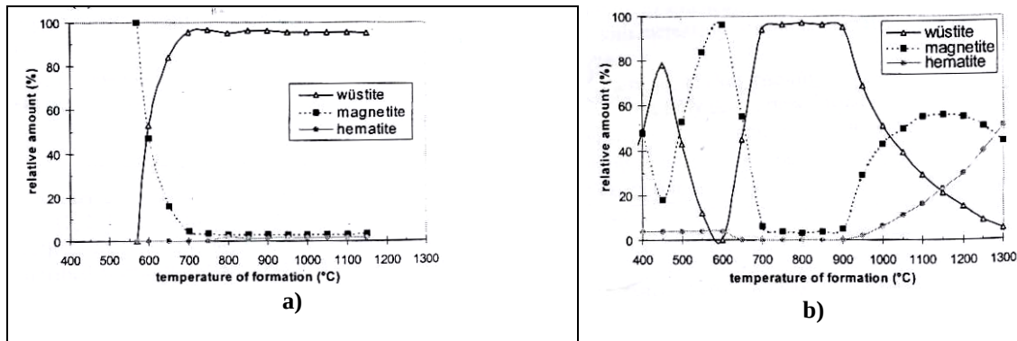
Figure II-10: a) Païdassi representation for pure iron
