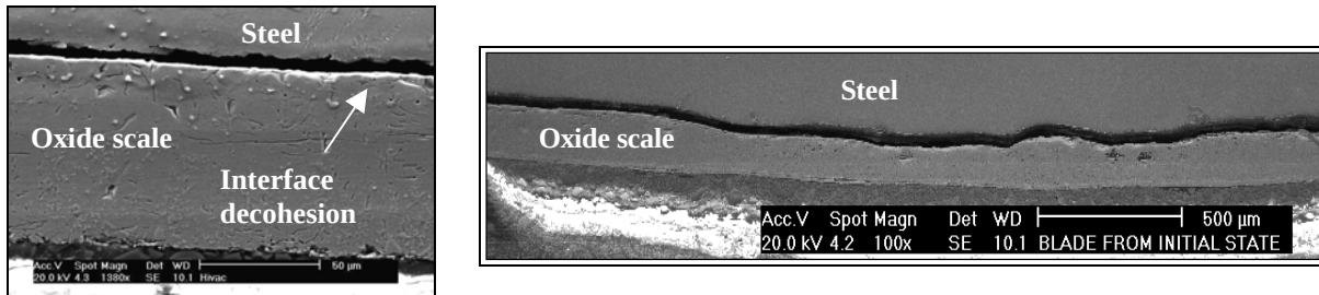
Figure IV-43: Decohesion at the metal-oxide interface. Ex-LC: deflection: 2mm - 1mm/mn-oxide:100µm. Left : 700°C / Right : 800°C.
