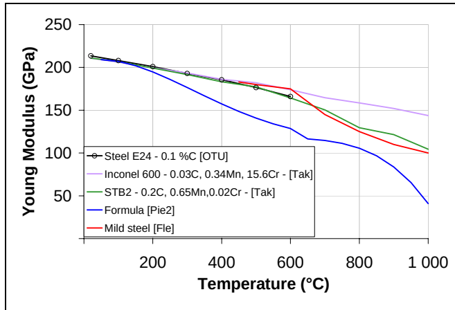
Figure A1-1: Young' modulus of steel vs. Temperature.
