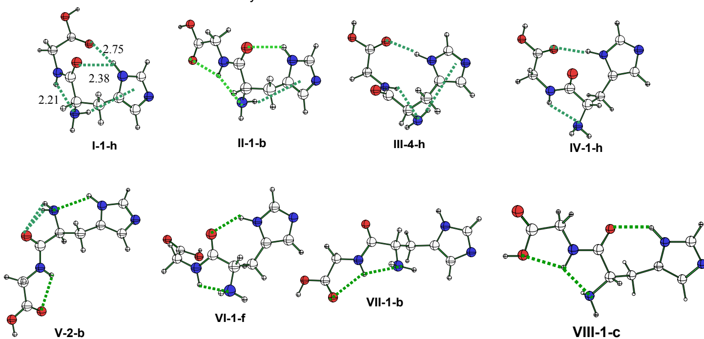
Figure 6 : Structure of the lowest energy conformer for each of the eight families of the \text{N}^{\text{D}}\text{-H} tautomer of HisGly.
