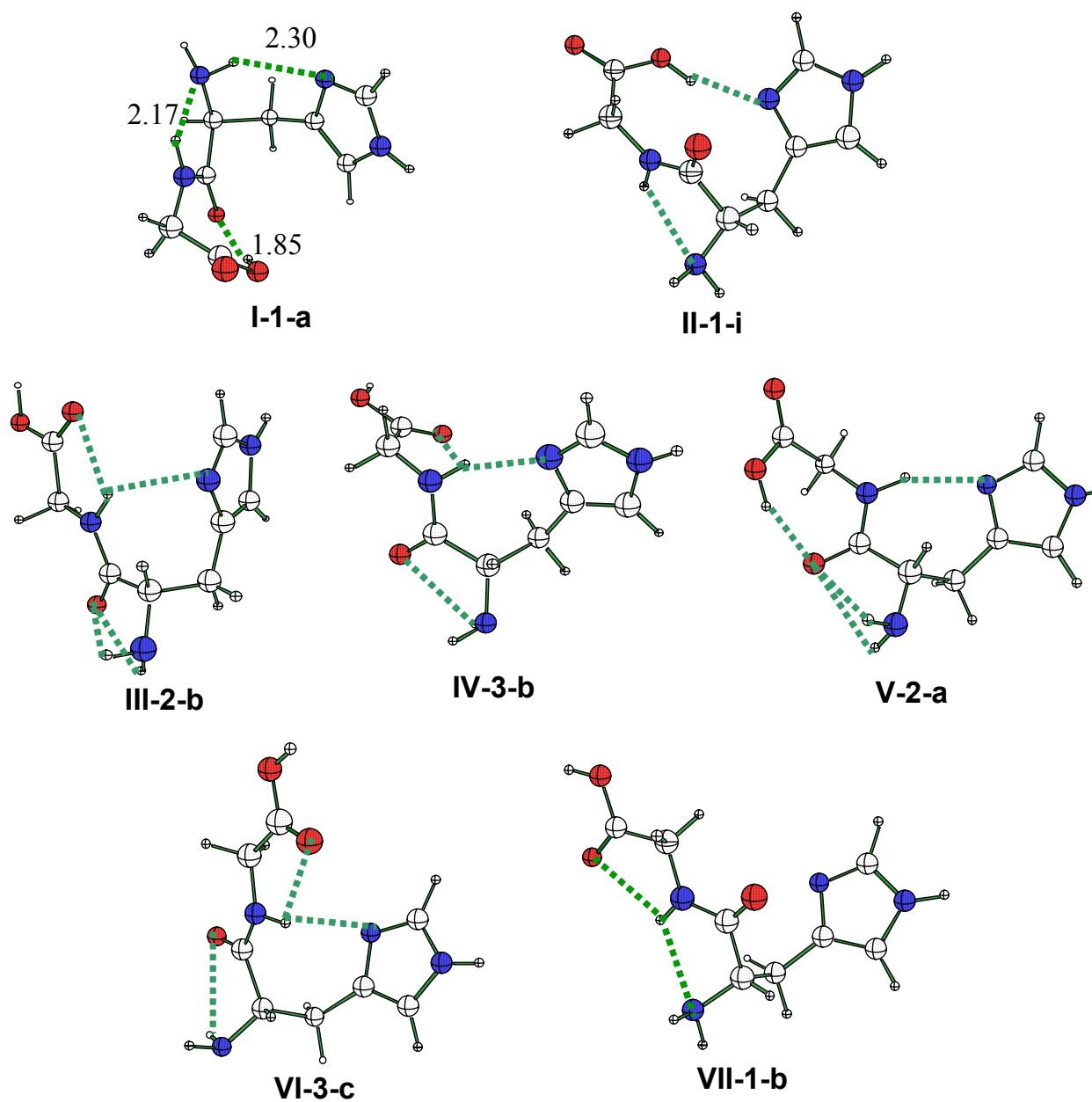
Figure 7 : Structure of the lowest energy conformer for each of the seven families of the \text{N}^\epsilon\text{-H} tautomer of HisGly.
