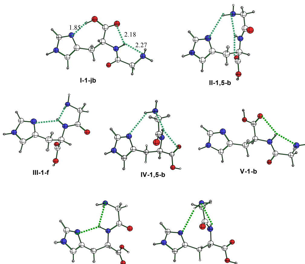
Figure 5 : Structure of the lowest energy conformer for each of the seven families of the \text{N}^{\text{E}}\text{-H} tautomer of GlyHis.
