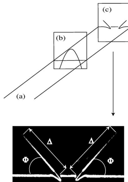
Fig. 6. In our experiment, a laser sheet (a) is refracted by the dry arch (b), the result being visualized on a screen (c) put behind the glass plate.
