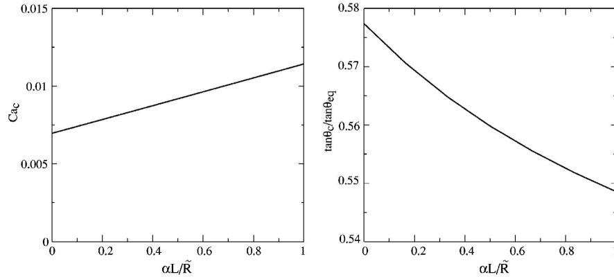
FIG. 11. The critical capillary number, \widetilde{Ca}_c , and critical slope, \tan \theta_c / \tan \theta_{eq} , as a function of the dimensionless contact line curvature \alpha L / \tilde{R} obtained from Eq. (18). These features are in qualitative agreement with full simulations of Eq. (17).
