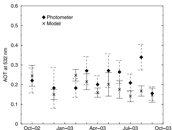
Figure 4. Monthly mean aerosol optical thickness at 532 nm, issued from Sun photometer measurements and CHIMERE simulations at Palaiseau, France, between October 2002 and September 2003.
