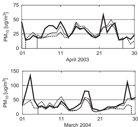
Fig. 6. Daily mean PM_{10} concentrations ( \mu\text{g m}^{-3} ) simulated by CHIMERE (thick line) and observed at Gennevilliers using both routine TEOM (dotted line) and reference PARTISOL (thin line) instruments.
