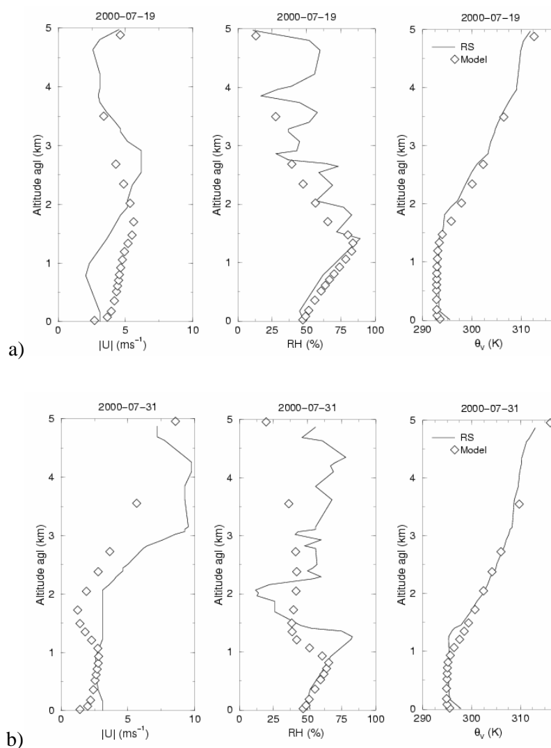
Figure 4: Vertical profiles of wind speed ( U ), relative humidity ( RH ) and potential temperature ( \Theta_v ) observed by Trappes ( 48.78^\circ\text{N} , 2^\circ\text{E} ) radiosoundings (solid line) and simulated by the model (diamonds) on 19 (a) and 31 (b) July 2000.
