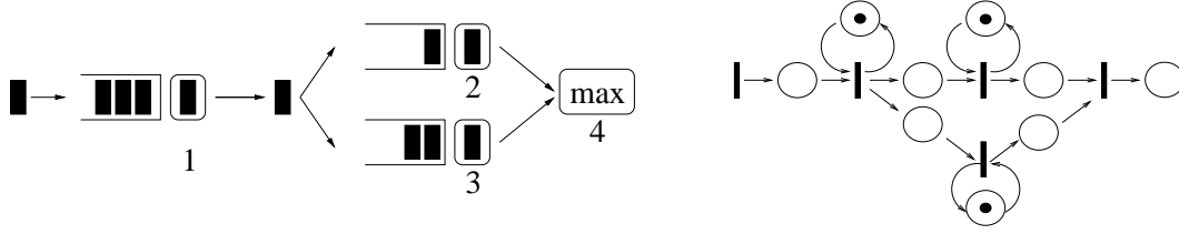
FIG. 2.2 – Tree Network
