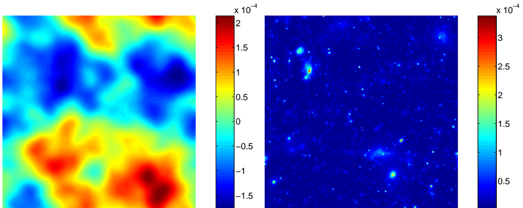
FIG. 5.1 – Simulated 1 degree by 1 degree maps. Left panel : CMB, Right panel : SZ clusters.
