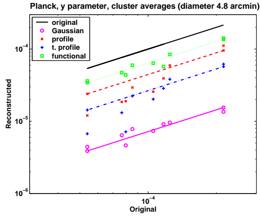
FIG. 5.19 – Reconstructed versus original central y -parameter (4.8 arcmin average).
