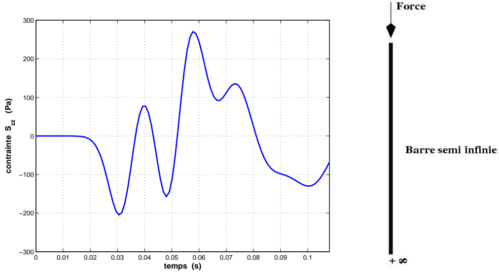
FIGURE 3.12. Contrainte verticale (maximale) \sigma_{zz}
