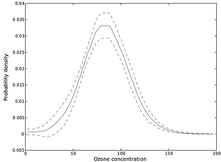
Figure 3.17: Relative frequency distribution f([\text{O}_3]) of the ozone concentrations ( \mu\text{g} \cdot \text{m}^{-3} ) of the reference simulation and the functions f([\text{O}_3]) \pm \sigma_f([\text{O}_3]) where \sigma_f([\text{O}_3]) is the standard deviation of f([\text{O}_3]) computed from all simulations.
