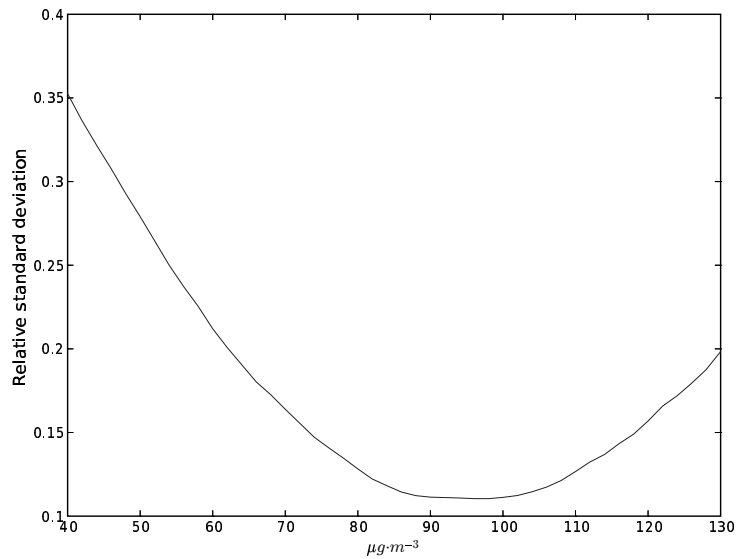
Figure 3.21: Relative standard deviation of the ensemble versus ozone concentrations. The average standard deviation is 17%.
