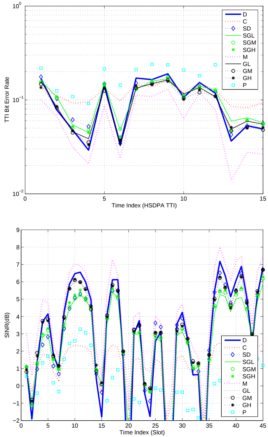
Figure 6.10: vA120 channel profile, 5 codes, E_c/\hat{I}_{or} = -3dB , \hat{I}_{or}/I_{oc} = 6dB
