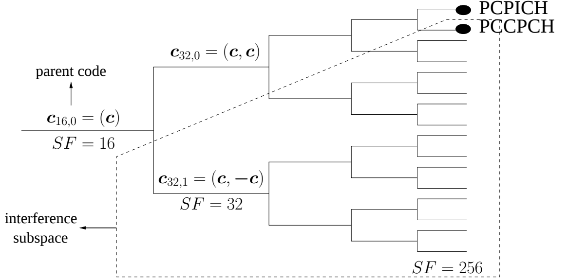
Figure 5.2: OVSF subtree rooted from c_{16,0} code
