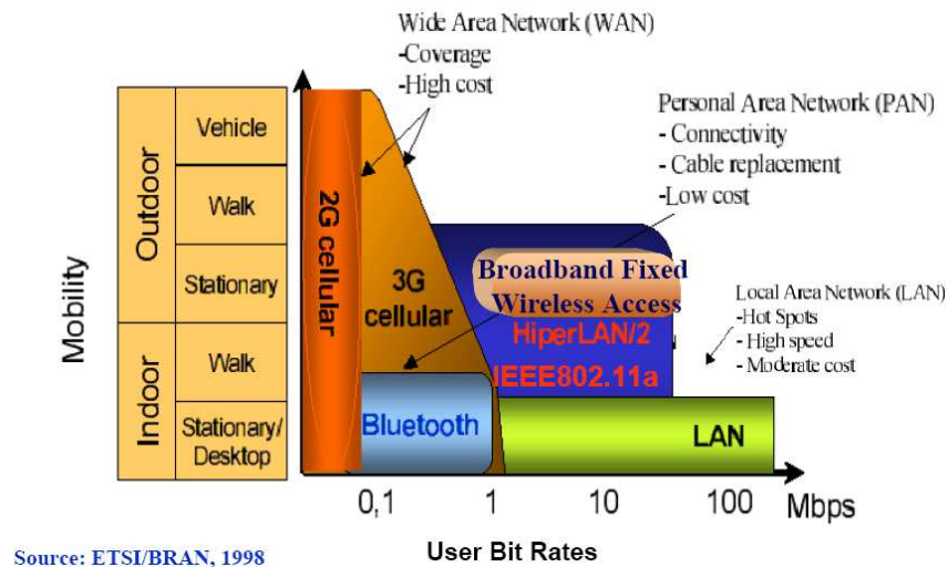
Figure 1.2: Mobility Versus Data Rates for Different Communication Systems
