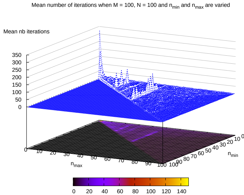
Figure 7.25: Impact of the n_{\min} and n_{\max} Variations on the Mean Number of Negotiation Steps
