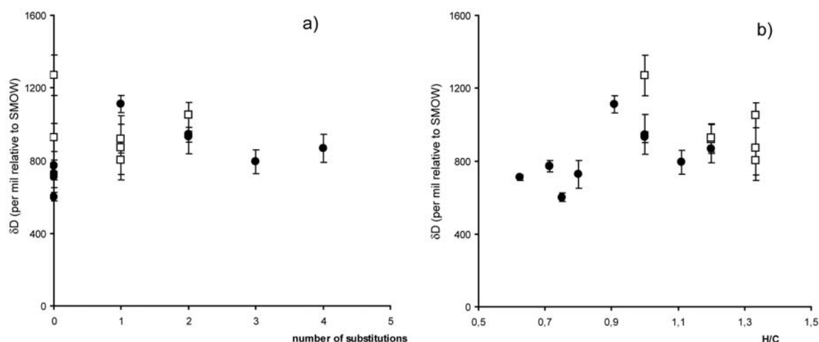
Figure 5-5: \delta D of aliphatic and aromatic compounds as of function of a) number of substitutions (number of carbons in the side chain) and b) H/C ratio. No obvious correlation is observed leading to the interpretation that the \delta D cannot be interpreted by considering the size of the moiety. Open squares represent aliphatic moieties, black circles aromatic ones.
