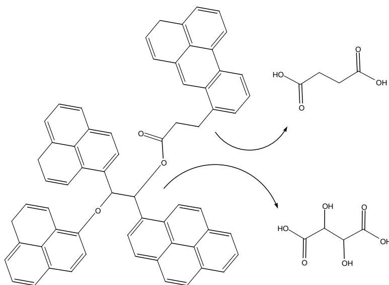
Figure 4-5 : Schematic pathway of ruthenium oxidation of four polycyclic aromatic units linked by an aliphatic chain with ether and ester functional groups (aromatic moieties are not representative of the chemical structure of the chondritic IOM).
