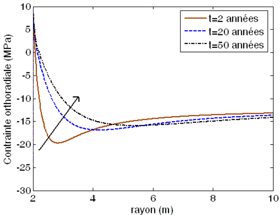
Figure 5-4 : Variation de la contrainte orthoradiale (98%RH-60%RH).
