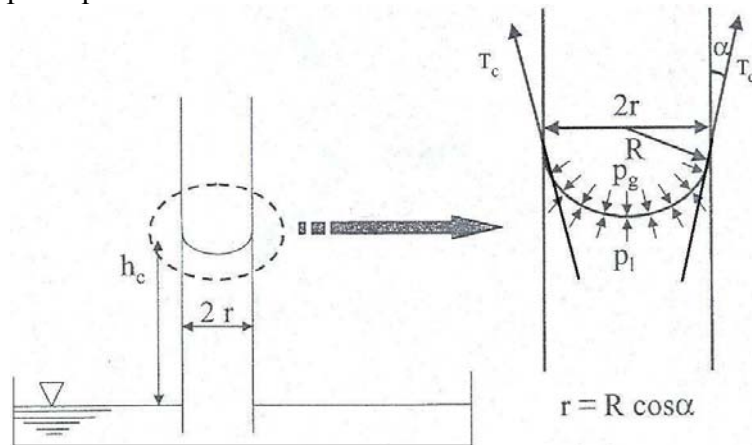
Figure 1-7 : Tube capillaire.
