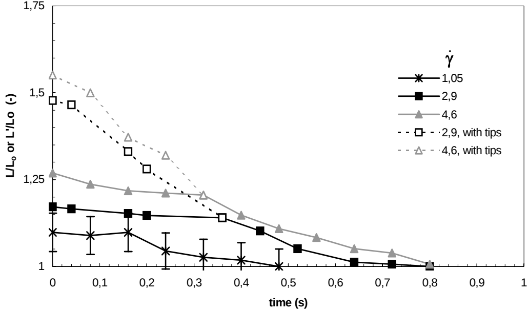
Figure 3.27: Shape relaxation of a gel particle swollen with 1 % HPC solution after having been submitted to different shear rates. Matrix fluid was PDMS 200, D_0 = 150 \mu\text{m} .
