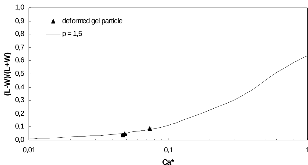
Figure 3.24: Experimental data compared to the modified Cox model for gels swollen with 1 % HPC solution ( Q = 80 g/g) suspended in PDMS 200.
