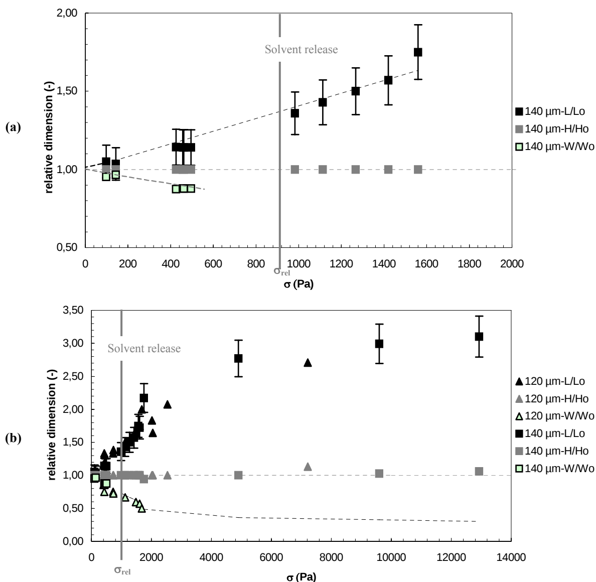
Figure 3.11: Pseudo-steady state deformation as a function of applied shear stress for particles swollen with 10 % HPC to 80 g/g, L_0 = 140 (■) and 120 (▲). Upper graph is a close-up of the initial part.
