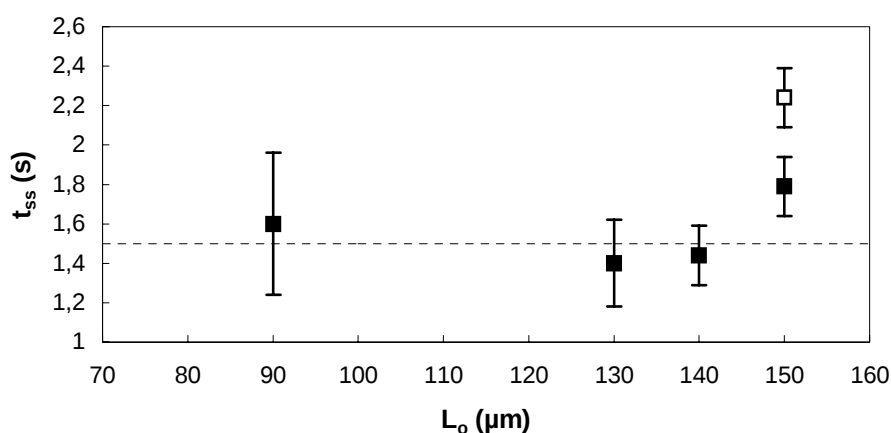
Figure 3.6: Effect of initial size on t_{ss} . Gel swollen with 10 % HPC solution, Q = 80 g/g immersed in PDMS 200. Shear rate \sim 5,5 \text{ s}^{-1} . The open symbol represents steady state of tips.
