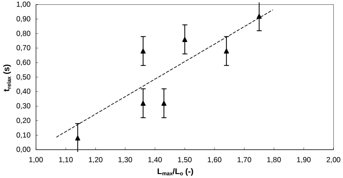
Figure 3.29: Relaxation times of gel particles swollen with 10 % HPC solution ( Q = 80 g/g, D_0 = 140 \mu\text{m} ) in PDMS 200.
