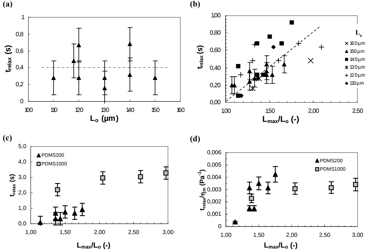
Figure 3.32: Effect of various parameters on relaxation times of gels swollen with 10 % HPC (80 g/g) in PDMS 200 except where precised differently. (a) Relaxation times for particles of different size with the same deformation before relaxation; (b) Relaxation time as a function of deformation before cessation of flow, sizes separated; (c, d) Effect of matrix viscosity on relaxation time for particles of the same size ( L_o = 140 \mu\text{m} ). Relaxation time is scaled with matrix viscosity in (d).
