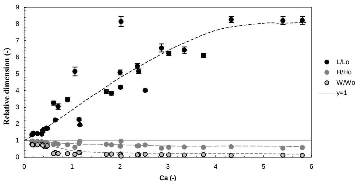
Figure 3.19: Relative dimensions at steady state of a 10 % HPC droplet immersed in PDMS 100 and 200.
