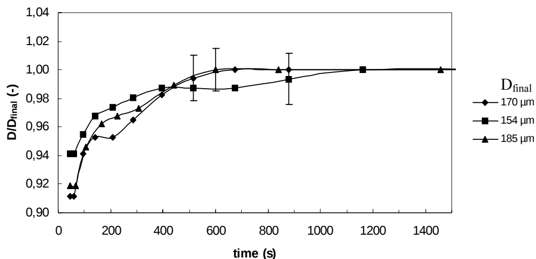
Figure 2.19: Swelling kinetics of Aqua Keep particles in 10 % HPC.
