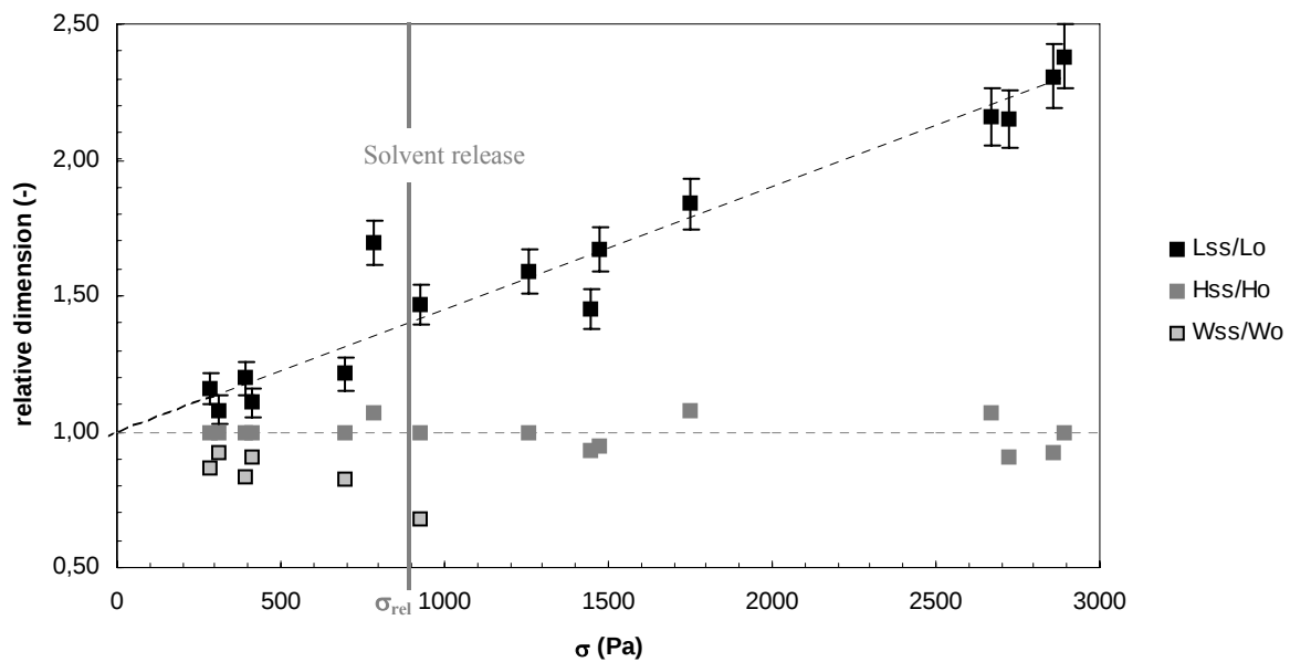
Figure 3.10: Stress-deformation data for particles swollen with 5 % HPC ( Q=80 g/g). D_o=110 \mu\text{m} .
