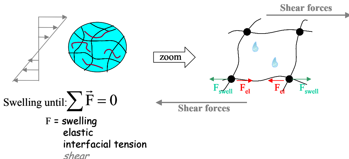
Figure 4.17: Schematic representation of stresses acting on a swollen gel under shear.
