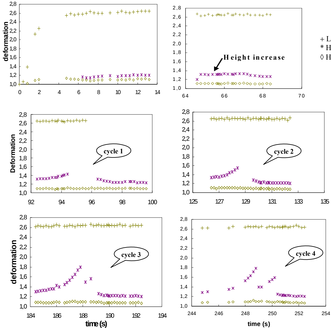
Figure 4.13: Kinetics of particle dimension stabilisation for a gel particle swollen with 10 % HPC in PDMS 200 at 2700 Pa. L adopts a steady value within the first 10 s. H and H' only start growing after a longer time. H' increases until the cap shape becomes impossible to measure, but H' can be measured again after mushroom detachment.
