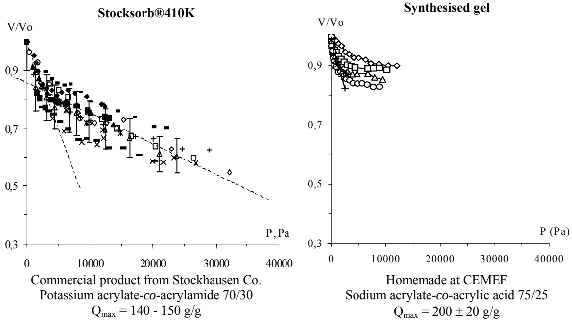
Figure 5.7: Comparison of volume loss between gels of different nature.
