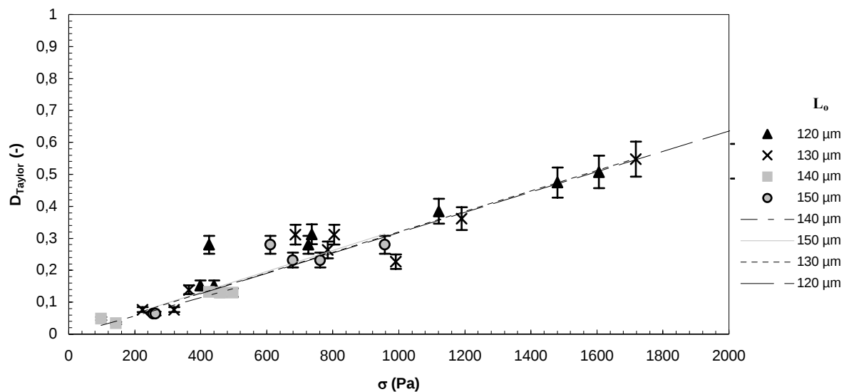
Figure 3.13: Steady state deformation (without tips) as a function of applied shear stress for different particle sizes. Particles are swollen with 10 % HPC, Q = 80 g/g. Lines are linear trends through the data series.
