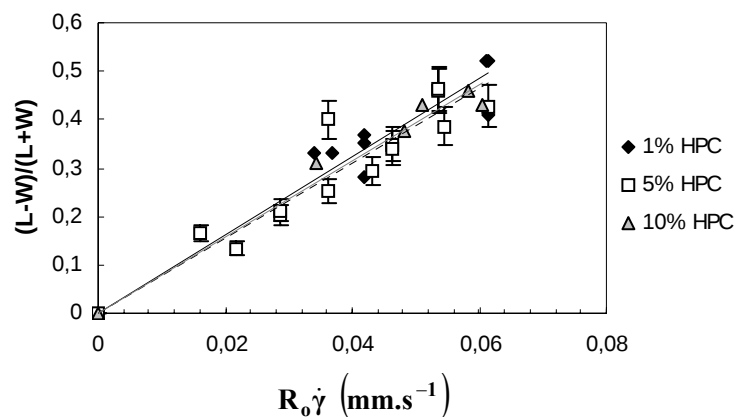
Figure 2.21: Taylor deformation as a function of R_o \dot{\gamma} for droplets of HPC solutions of different concentrations in PDMS 100. Straight lines are linear fits whose slopes determine interfacial tension: full black line: 1 % HPC; dashed black line: 5 % HPC; full grey line: 10 % HPC. Error bars are only shown for one series to avoid overloading the graph.
