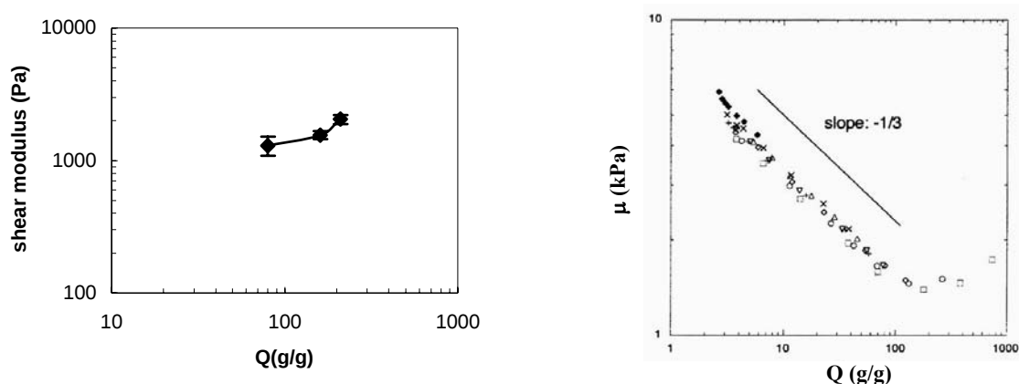
Figure 3.17: Gel swollen with 5 % HPC. (a) Effect of Q on \mu . (b) Comparison with tendency from literature [From Horkay et al., 2000].
