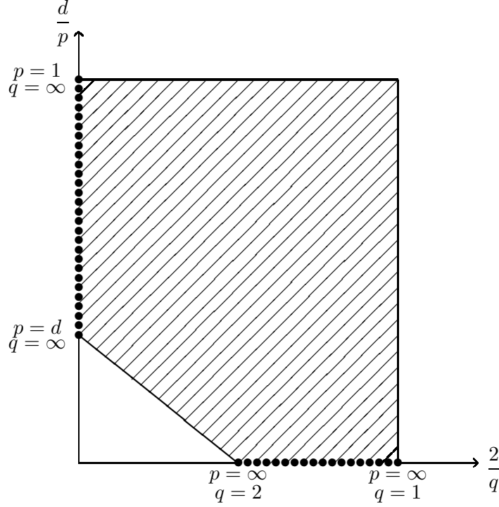
Figure 3.3: Initial value spaces (\dot{B}_{p,q}^{-1+d/p})_\sigma for which weak-strong uniqueness holds
