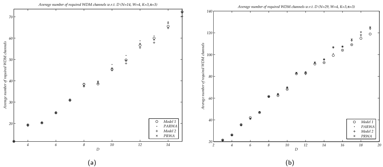
Figure 4.9 : Average number of required WDM channels w.r.t. D
