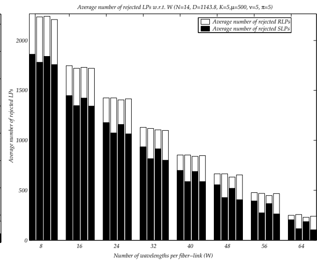
Figure 5.14 : average number of rejected lightpaths
