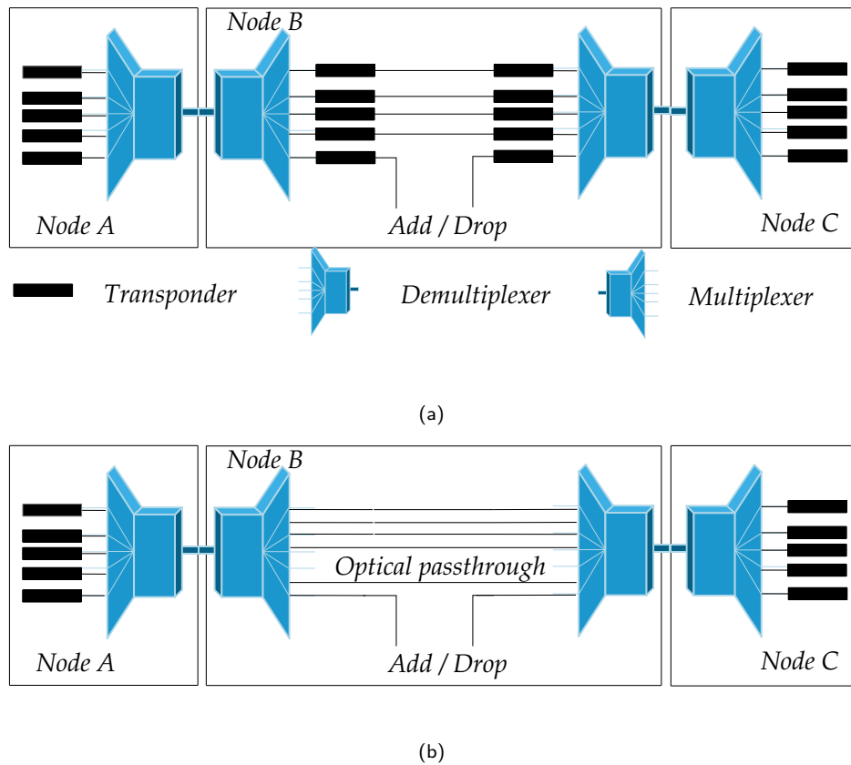
Figure 2.1 : A three-node network example to illustrate the role of OADM
