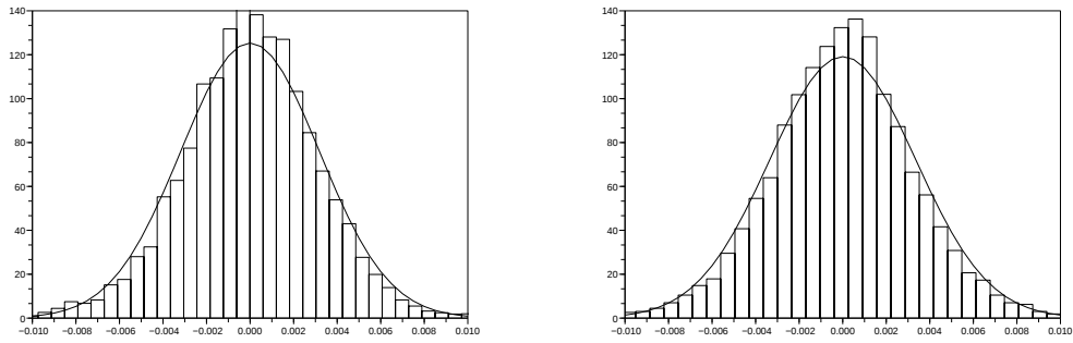
FIG. 4.11 – Histograms of the residues \hat{\epsilon}_{2n} (new poles, left) and \hat{\epsilon}_{2n+1} (old poles, right), and their fit to Gaussian distributions
