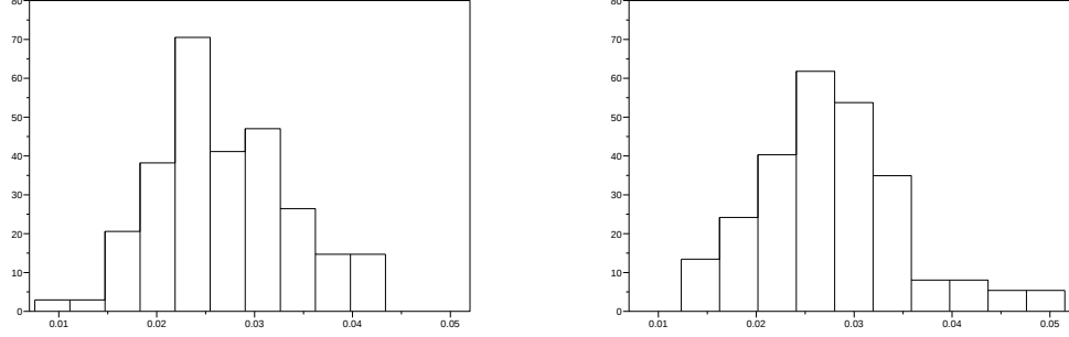
FIG. 4.9 – Histograms of \hat{\beta}_0 (left) and \hat{\beta}_1 (right)
