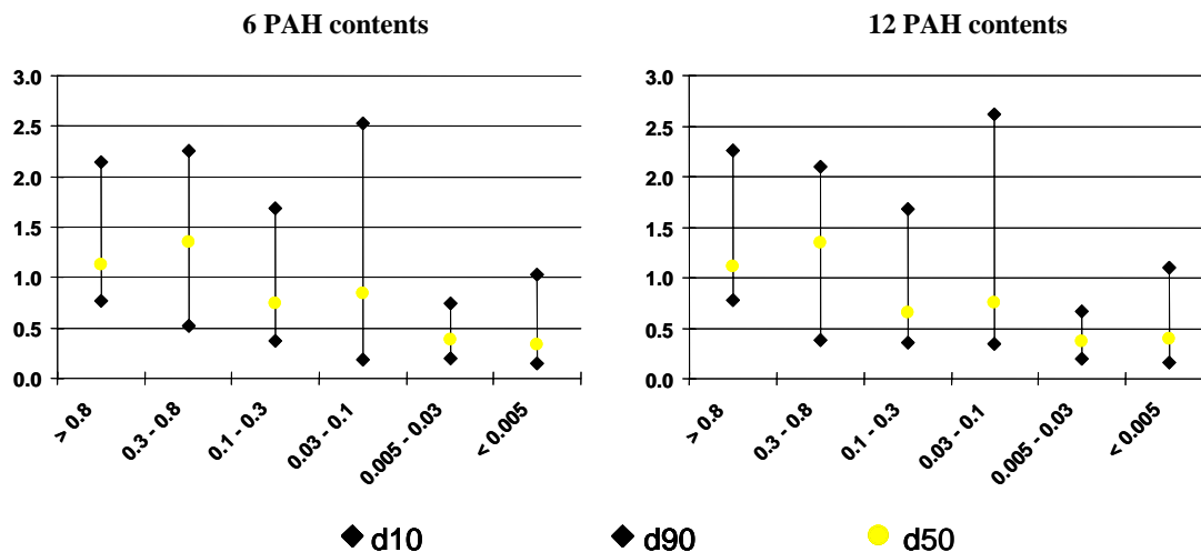
Figure 5: Standardised contents of PAHs within settling velocity fractions
