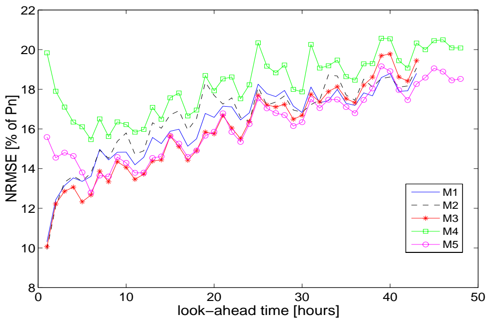
Figure D.14: Performance evaluation of the forecasting methods by the use of the NRMSE measure as a function of the look-ahead time.
