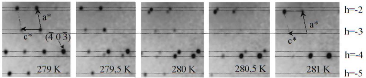
Figure 2. a) Temperature dependence of the diffraction intensity in the reciprocal lattice (h0l) . For clarity a zoom is made around the (403) Bragg reflection (strong Bragg reflection). The horizontal dotted lines correspond to the h lines in the two reciprocal lattices. The coexistence of the M and I phases gives rise to the coexistence of the corresponding Bragg peaks. The (40l) and (50l) peaks are present only in the I phase due to the symmetry breaking.
