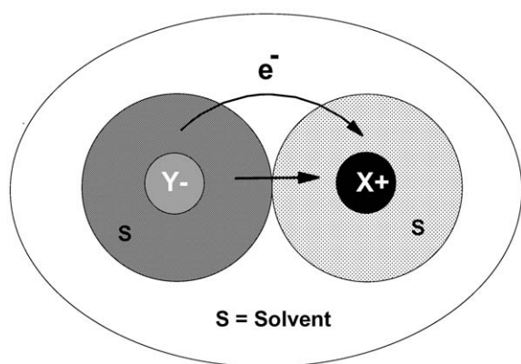
Fig. 1. Different electron transfer trajectories in solvent-bridged
