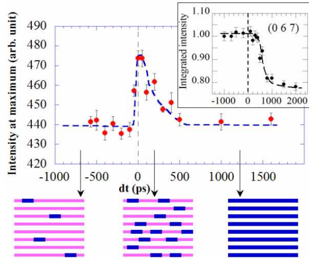
Fig.3 : Time dependence of the intensity at maximum of the diffuse scattering. The increase of the diffuse scattering signal, measured at (3\ 1\ -0.8) as on Fig. 1d, is associated with the formation of exciton-strings (blue strings in the scheme) and is characteristic of local precursor phenomenon. The macroscopic 3D transition takes place in a second step, changing the intensity of Bragg peaks such as the (0\ 6\ 7) (inset from ref. 6).
