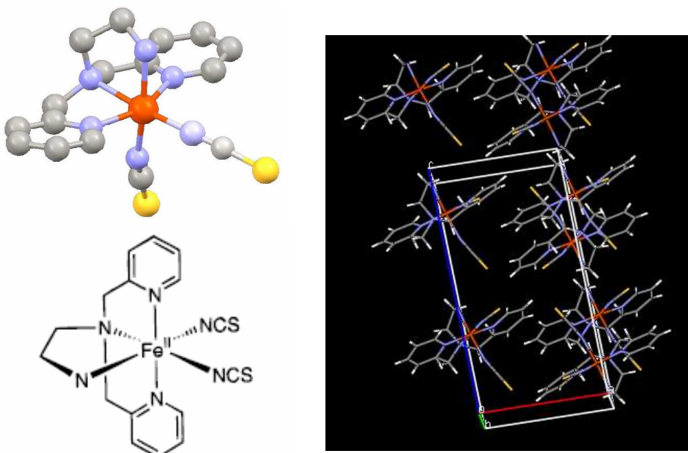
Figure 2.11: Structure cristalline 3D du complexe [Fe(DPEA)(NCS)_2] .
