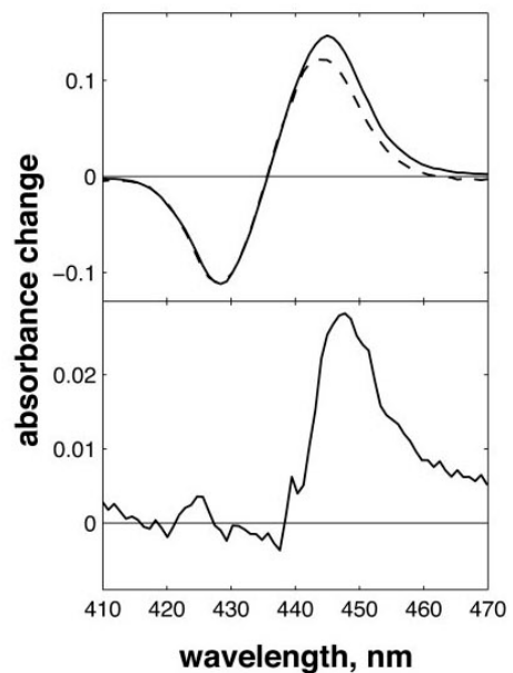
Fig. 2. CO photolysis spectra in CcO, obtained from extrapolating global fits to the data at t > 30 ps to t = 0 . (Upper) CO photolysis spectra in FR (solid line) and MV (dashed line) states, normalized at 428 nm. Both spectra are calculated to be isotropic ((\Delta A_{\parallel} + 2\Delta A_{\perp})/3) . (Lower) the difference spectrum.
